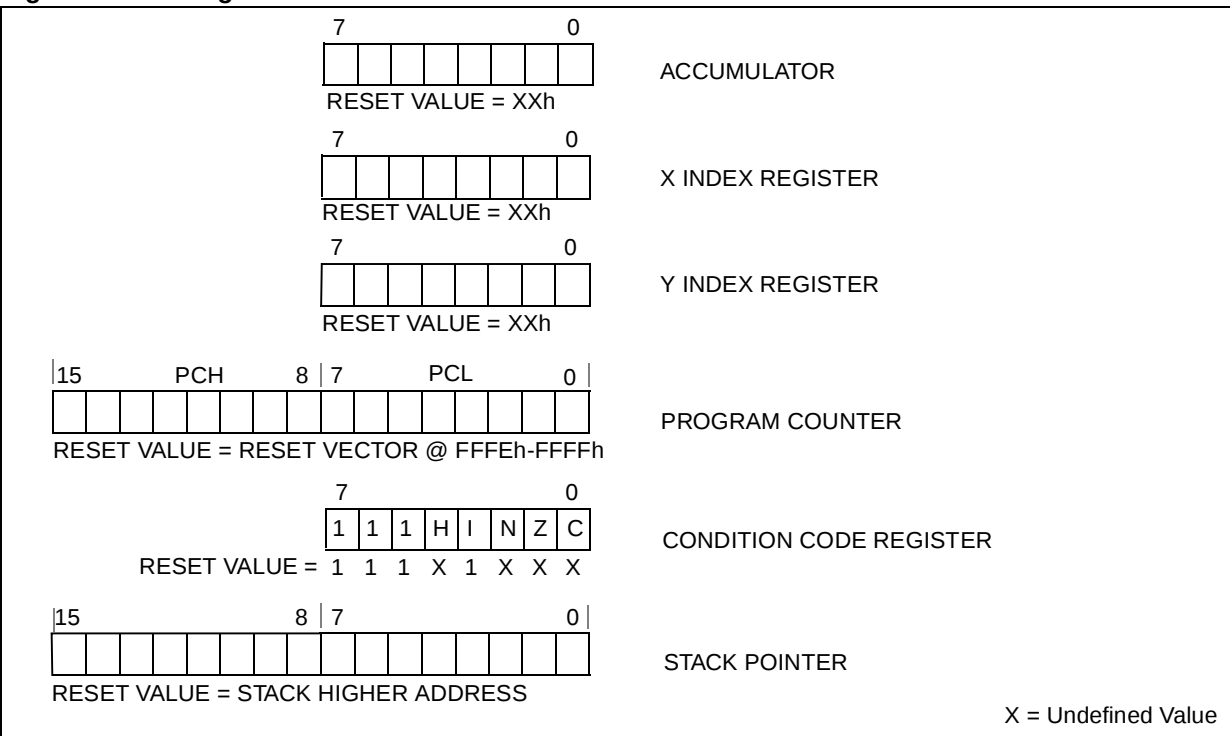
Figure 6. CPU Registers
