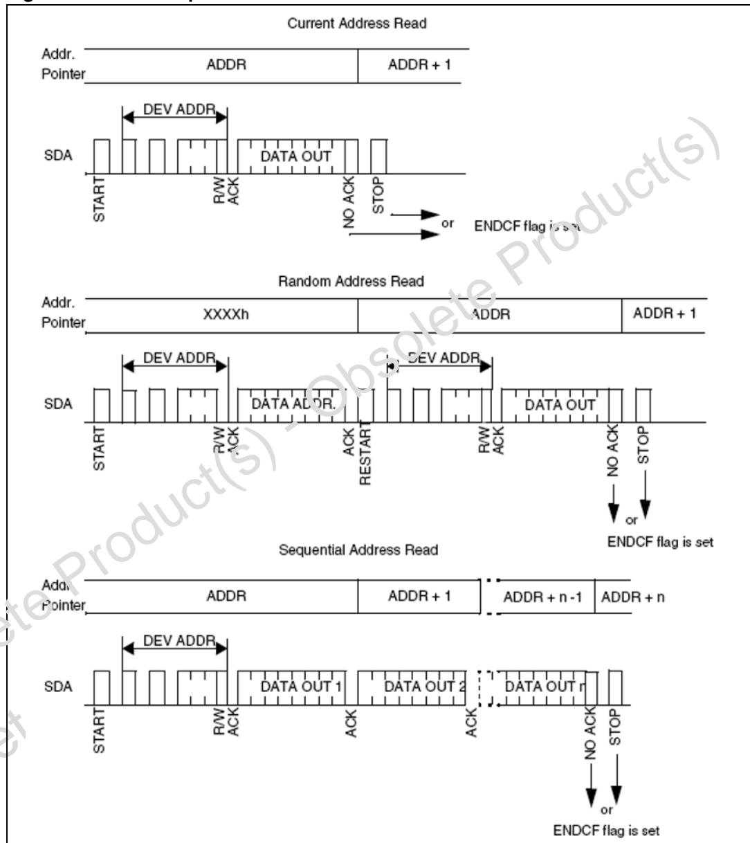
Figure 38. Read sequences
