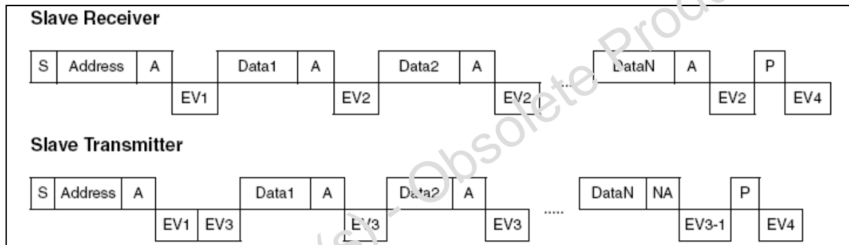
Figure 39. Transfer sequencing
