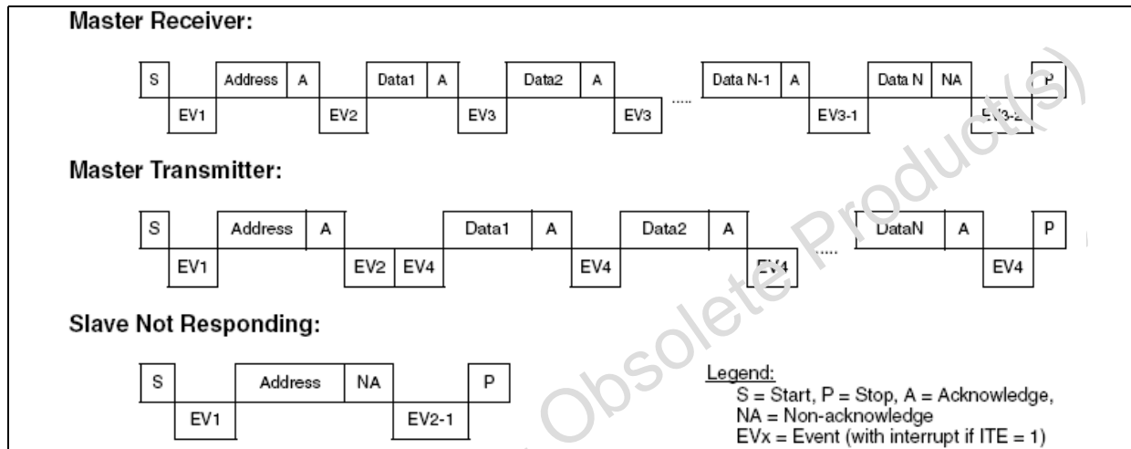
Figure 30. Transfer sequencing
