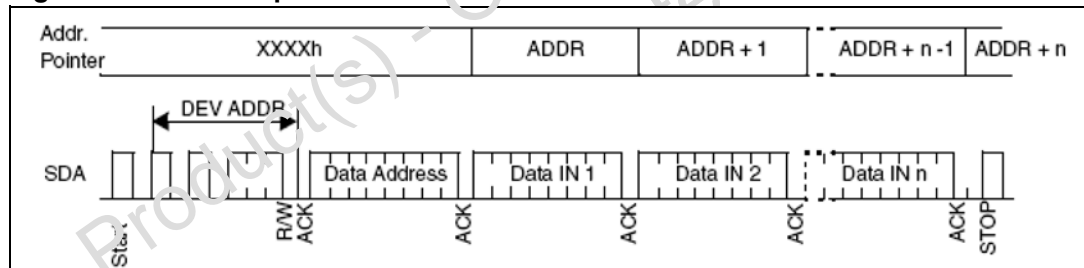
Figure 37. Write sequence
