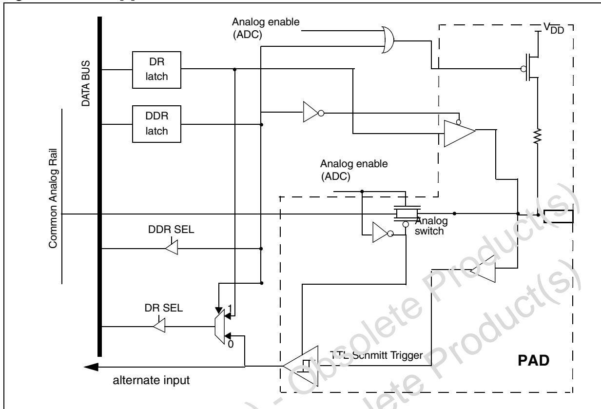
Figure 20. Port B [3]
