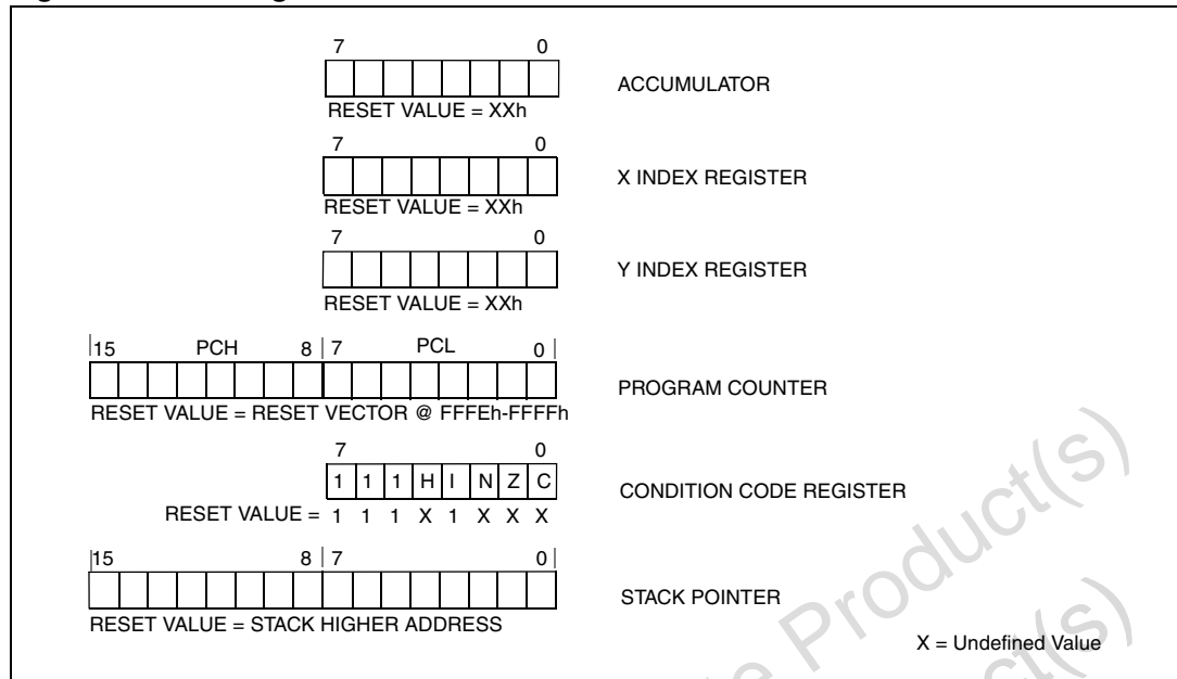
Figure 5. CPU registers
