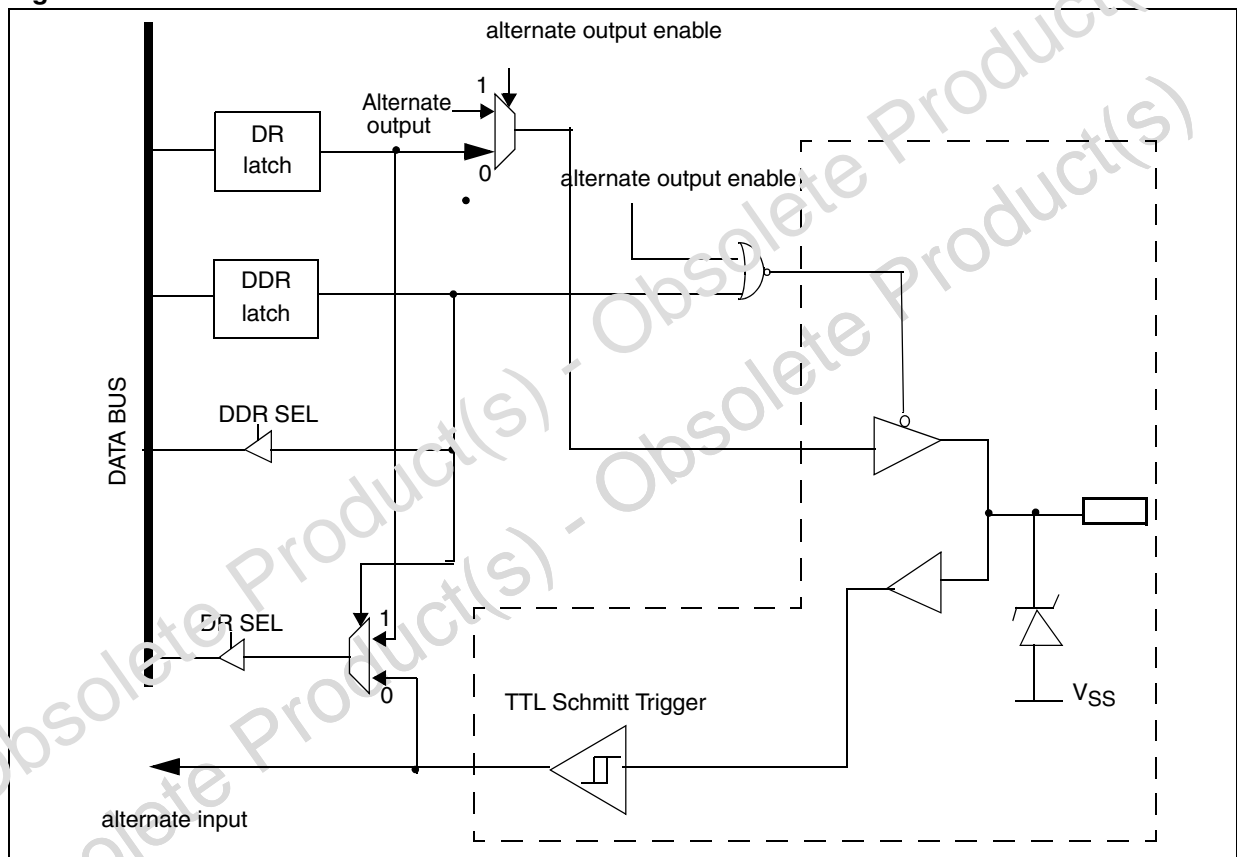
Figure 22. Port D
