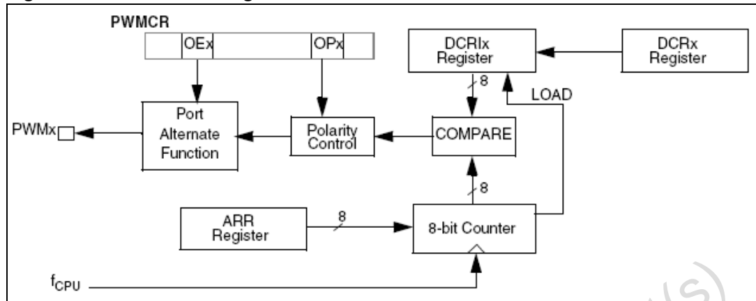
Figure 24. PWM generation
