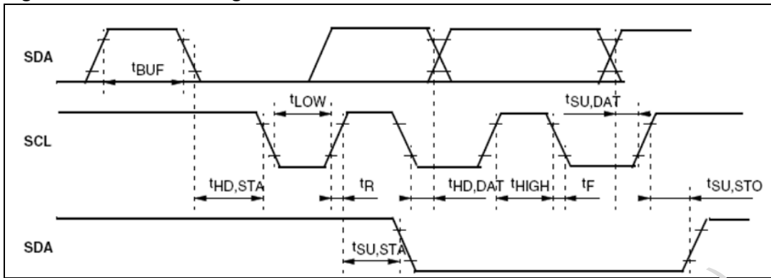
Figure 45. I2C bus timing
