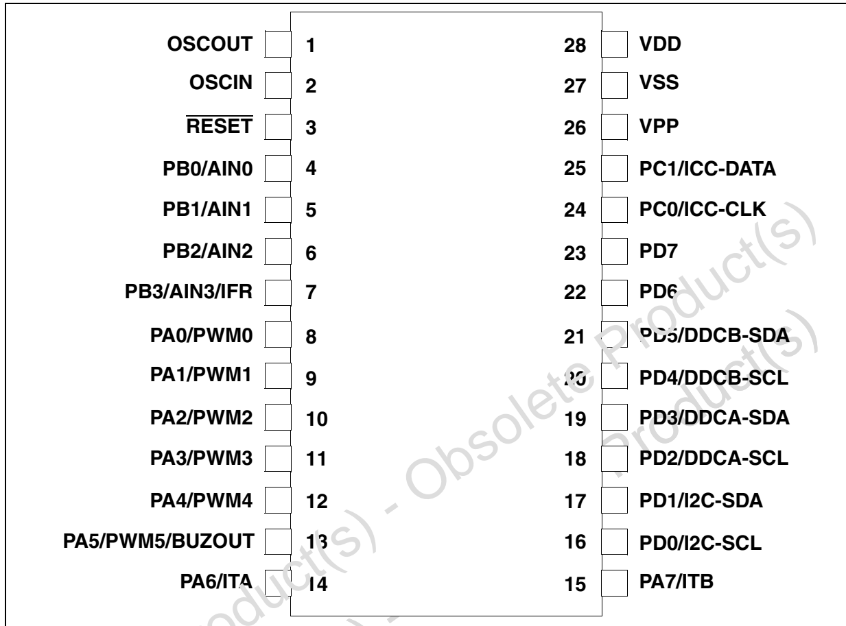
Figure 2. 28-pin small outline package (SO28) pinout
