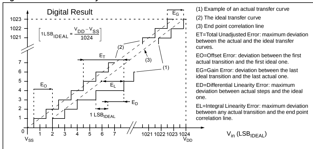
Figure 92. ADC accuracy characteristics
