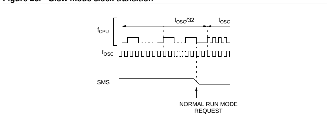
Figure 23. Slow mode clock transition
