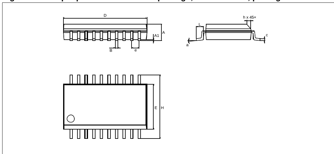
Figure 94. 20-pin plastic small outline package, 300-mil width, package outline
