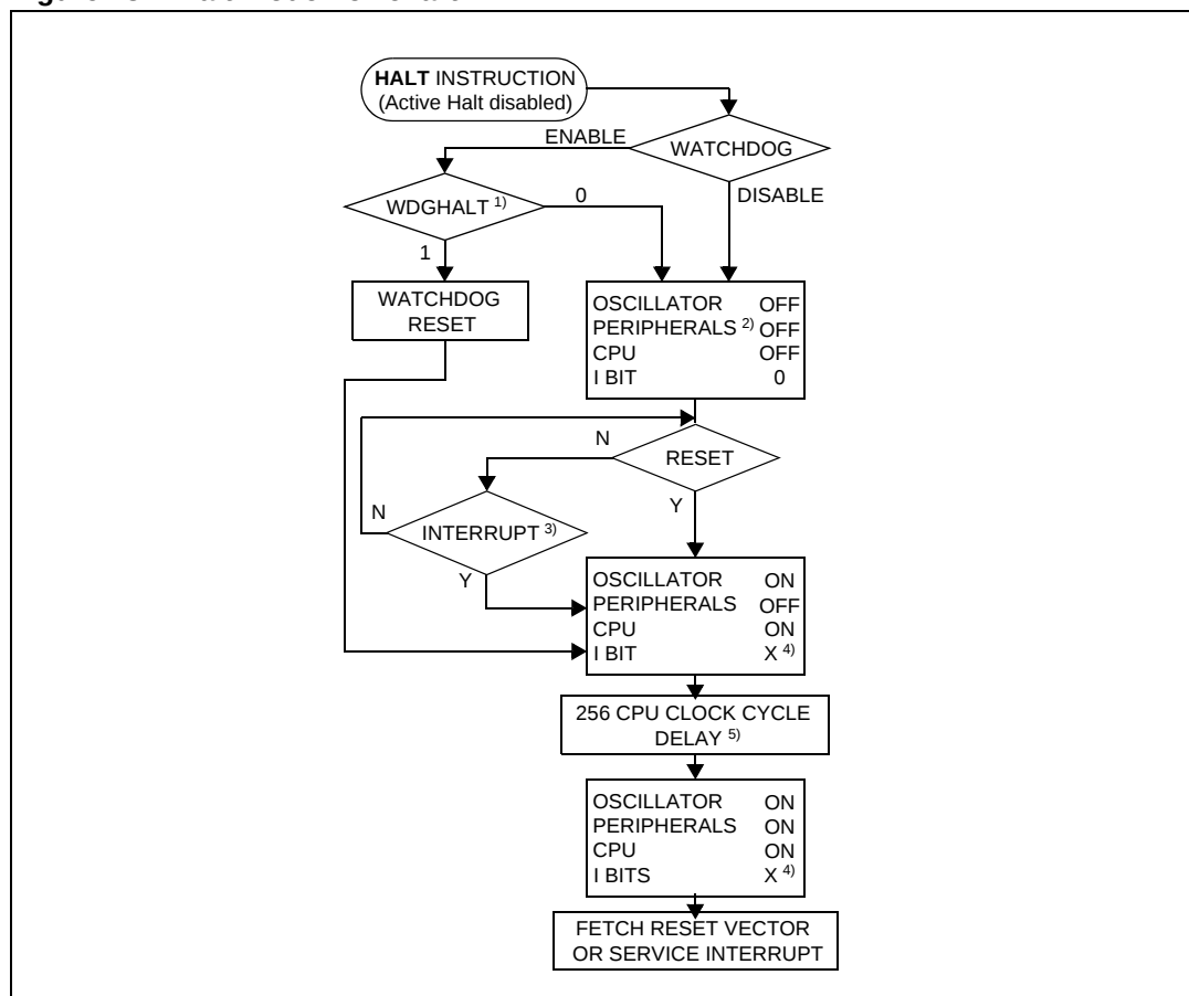
Figure 28. Halt mode flowchart
