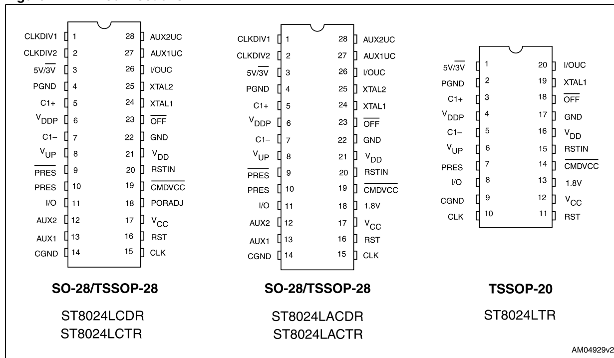
Figure 2. Pin connections
