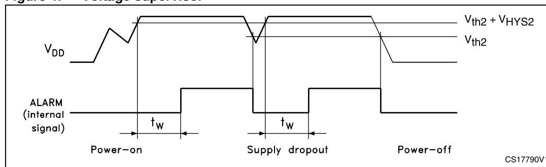
Figure 4. Voltage supervisor
