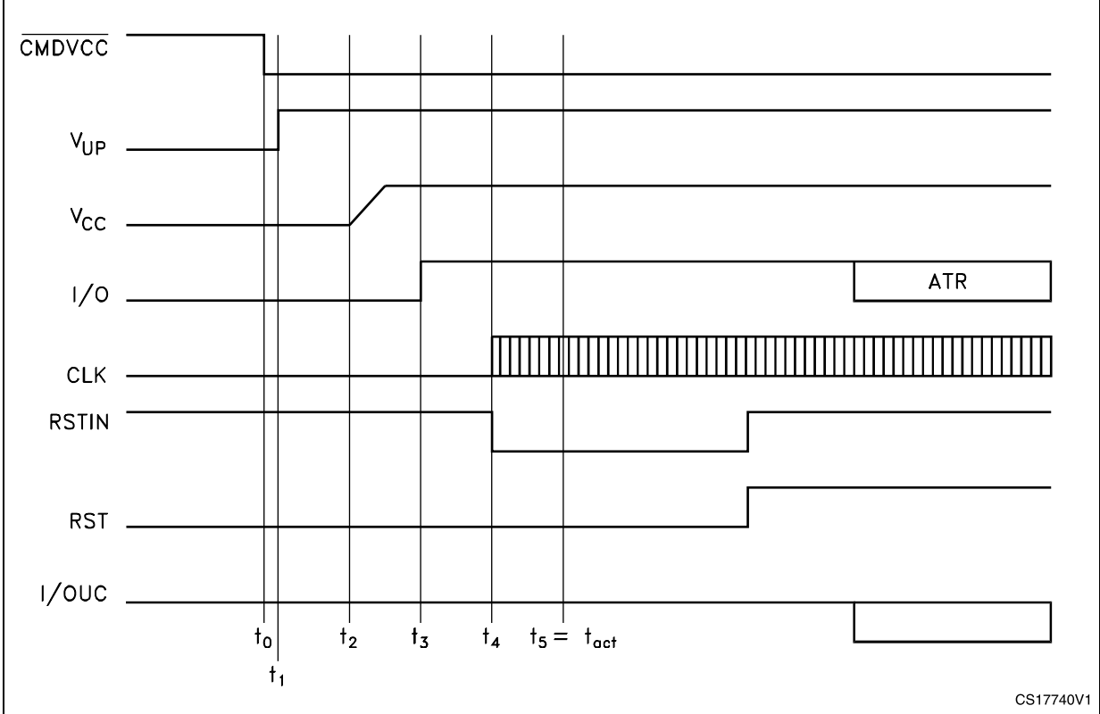
Figure 5. Activation sequence using RSTIN and CMDVCC
