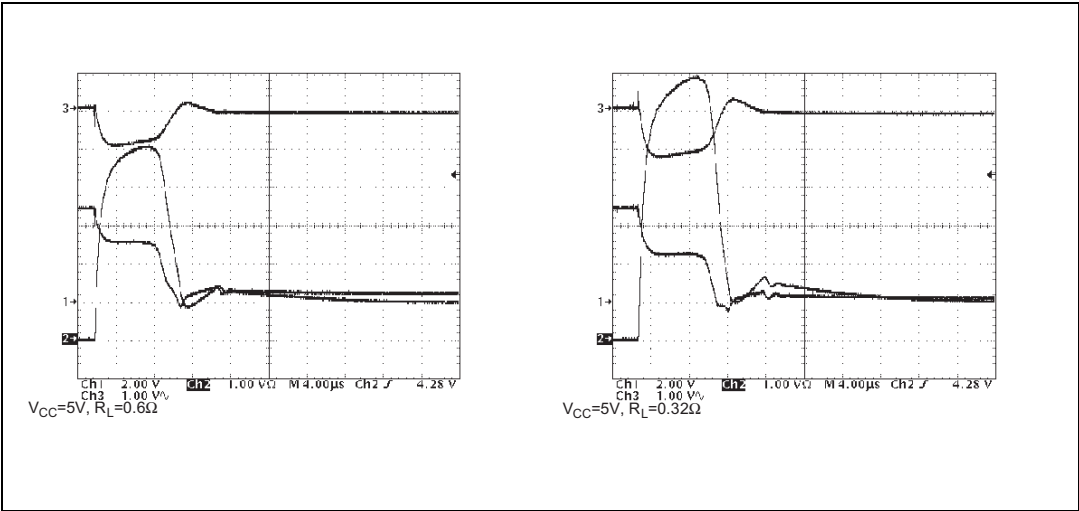
Figure 7. Switching waveforms
