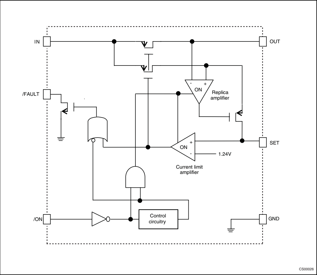
Figure 3. Schematic diagram
