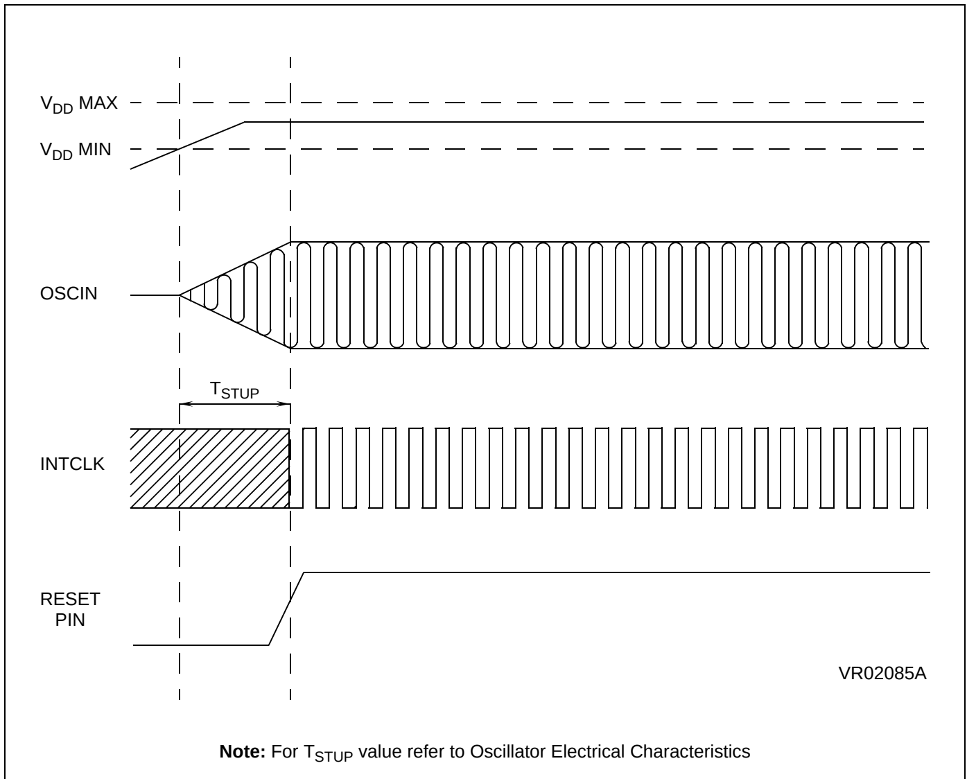
Figure 53. Oscillator Start-up Sequence and Reset Timing
