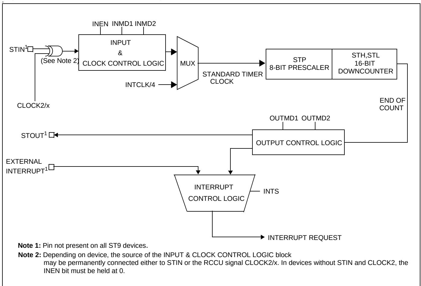
Figure 72. Standard Timer Block Diagram
