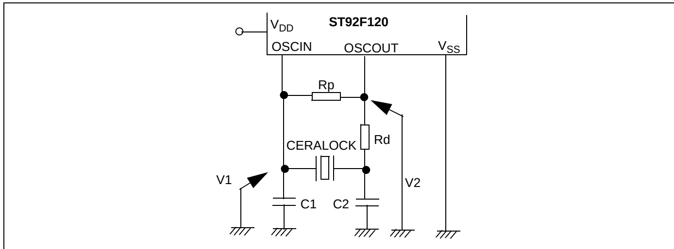
Figure 52. Test Circuit
