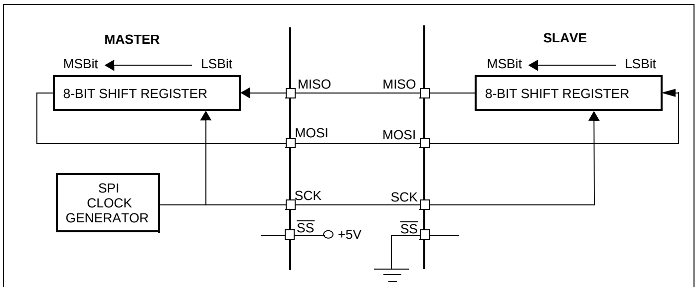
Figure 99. Serial Peripheral Interface Master/Slave
