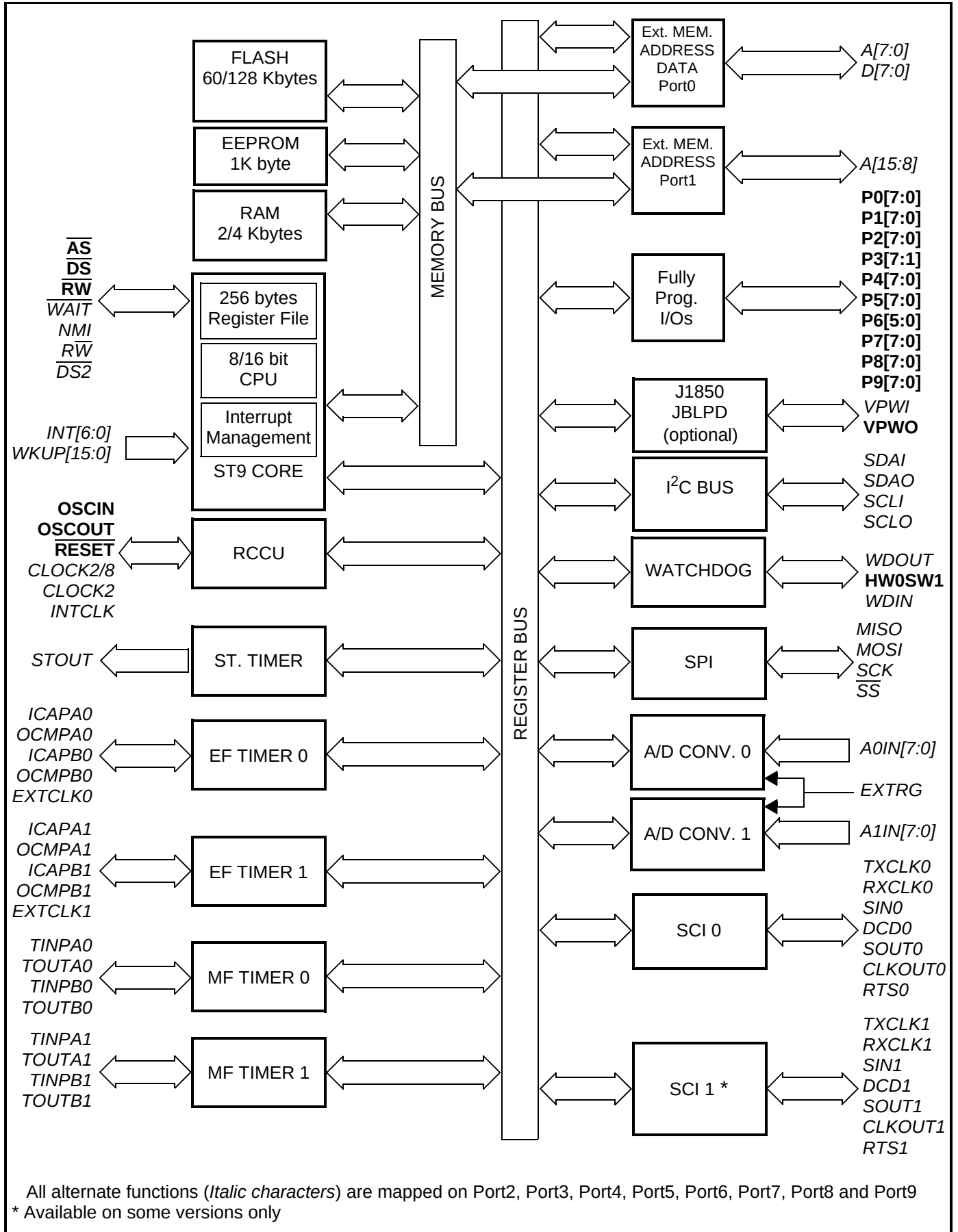
Figure 1. ST92F120JV: Architectural Block Diagram
