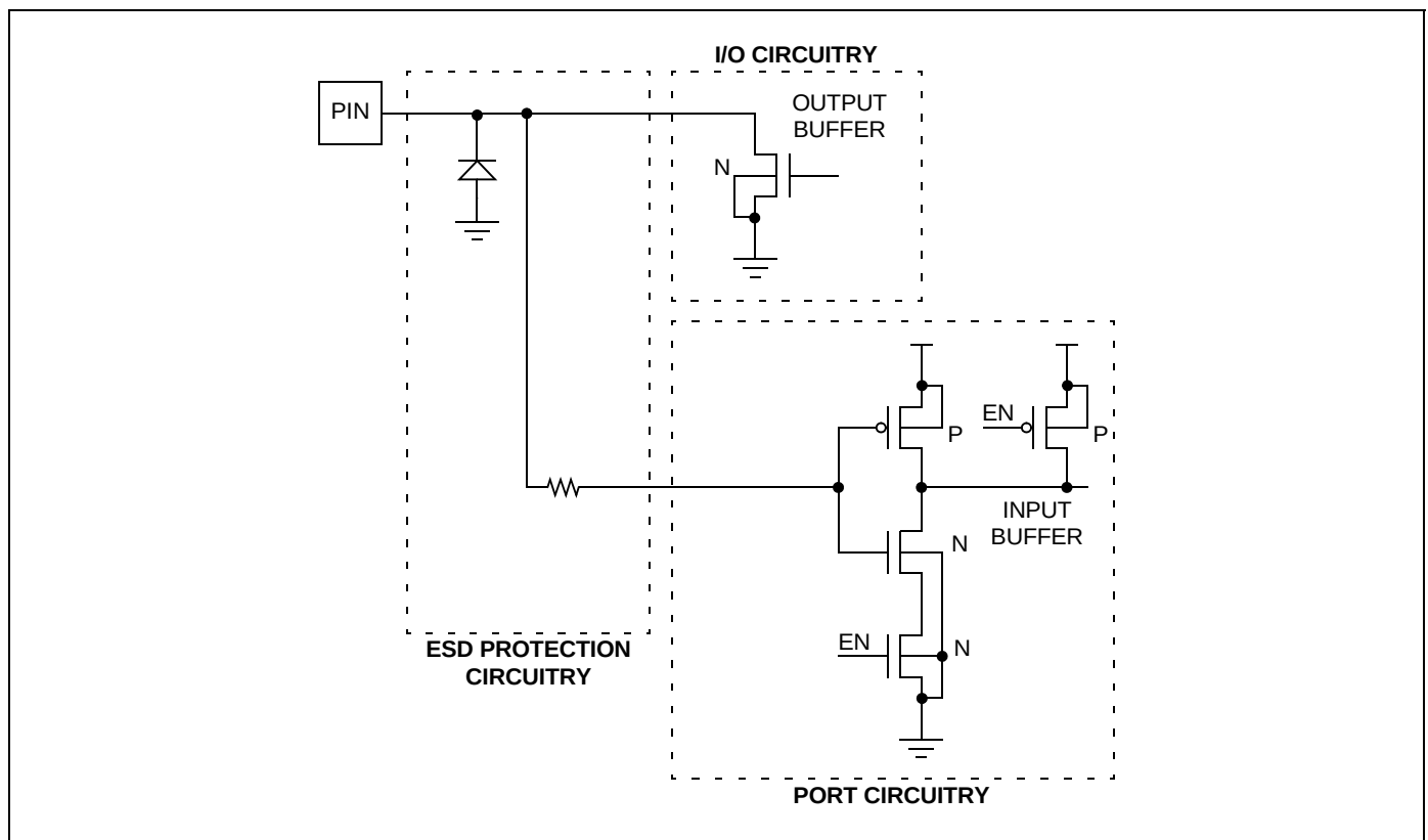
Figure 4. Digital Input/Output - True Open Drain Output
