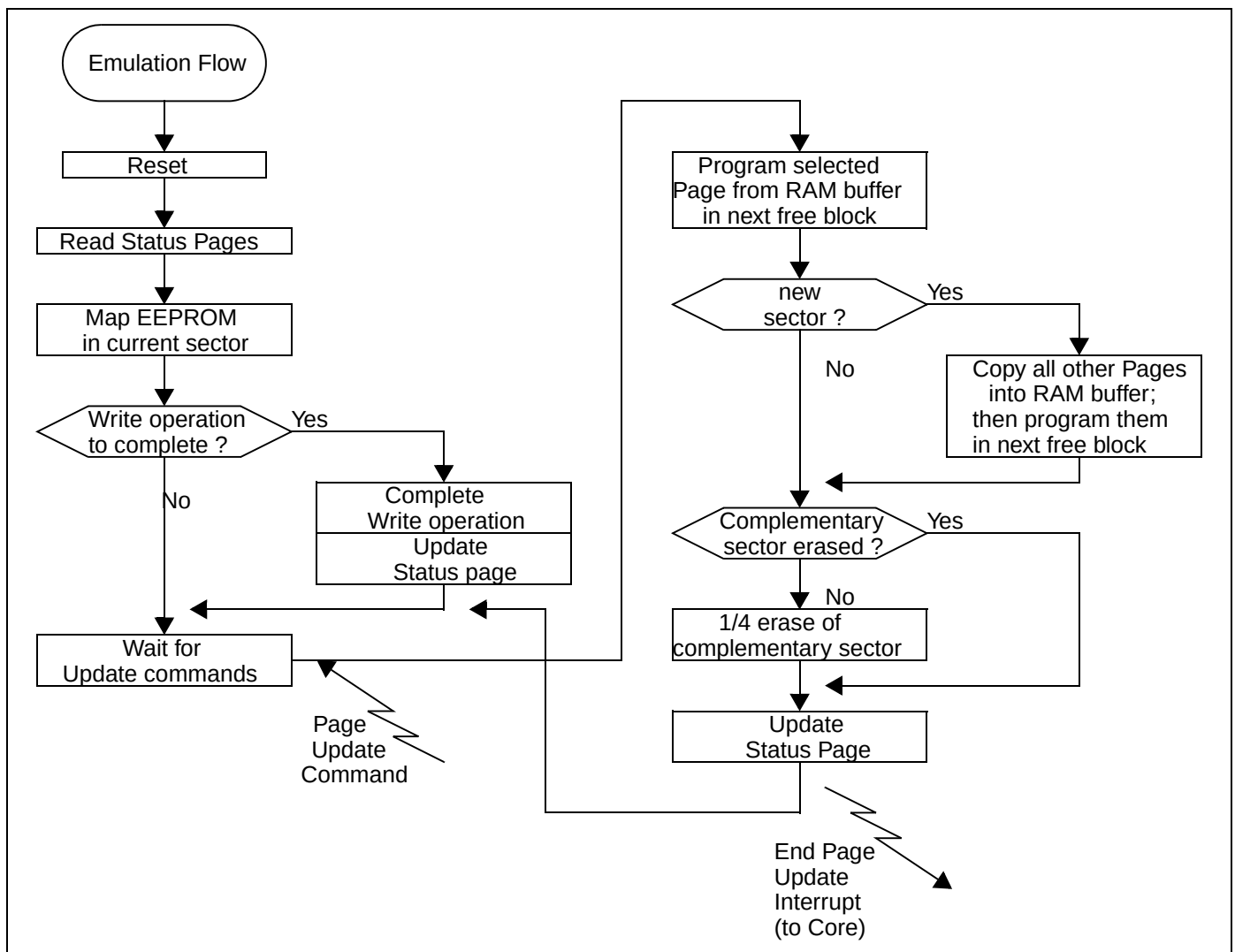
Figure 24. Hardware Emulation Flow
