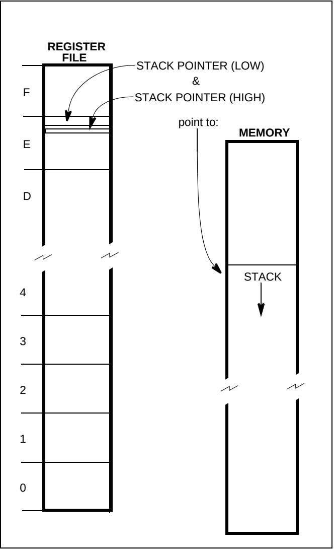
Figure 16. External Stack Mode
