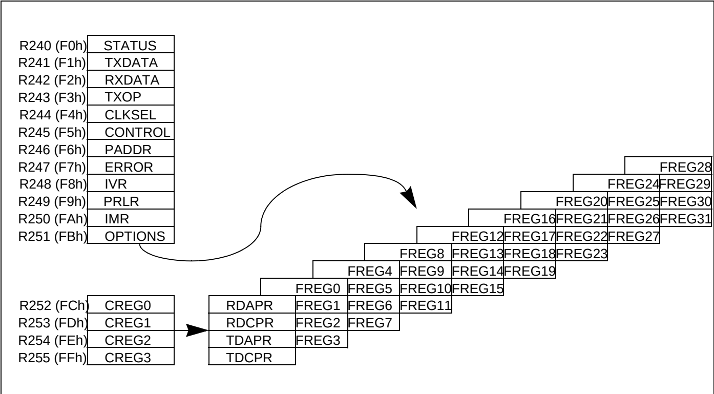
Figure 120. JBLPD Register Map
