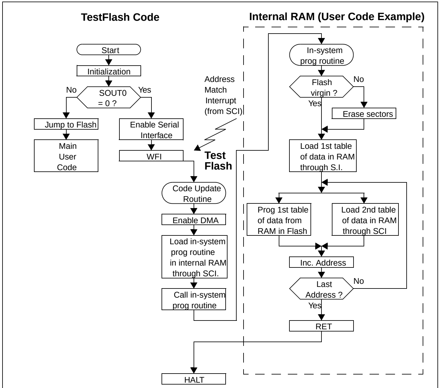
Figure 26. Flash in-system Programming
