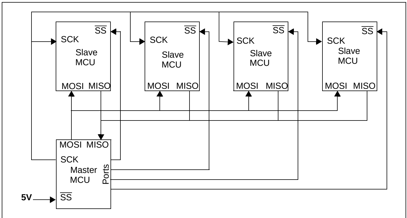
Figure 104. Single Master Configuration
