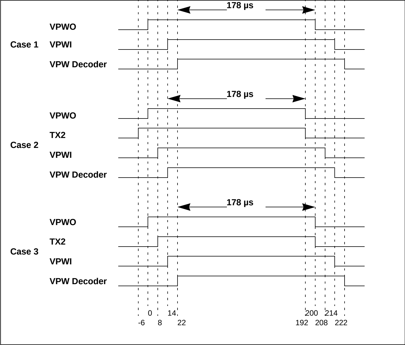
Figure 115. J1850 Received Symbol Timing
