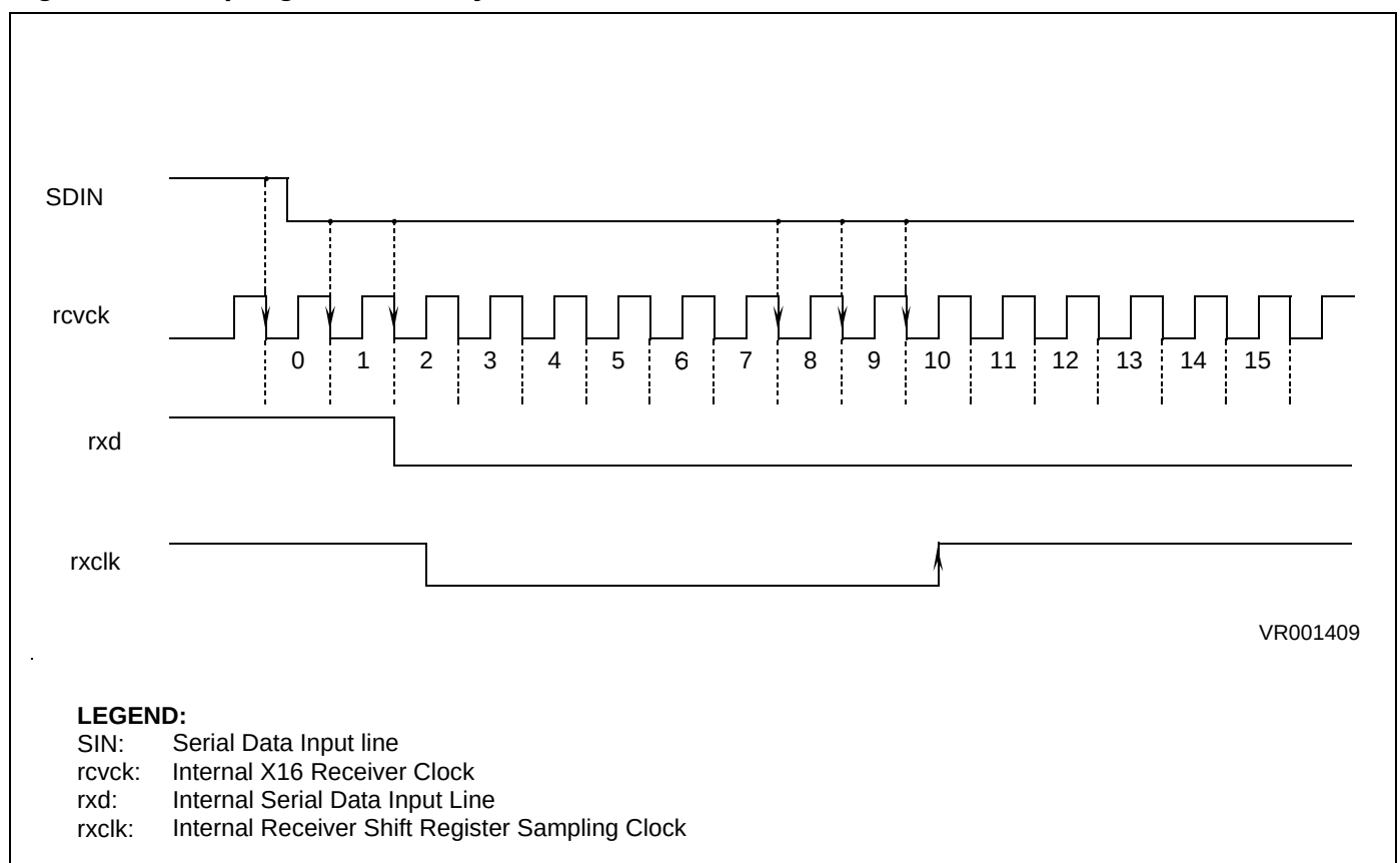
Figure 90. Sampling Times in Asynchronous Format
