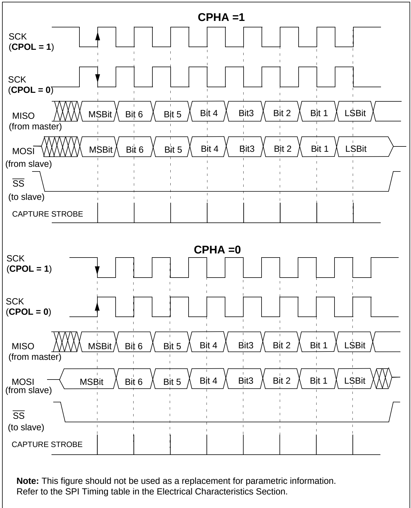
Figure 102. Data Clock Timing Diagram
