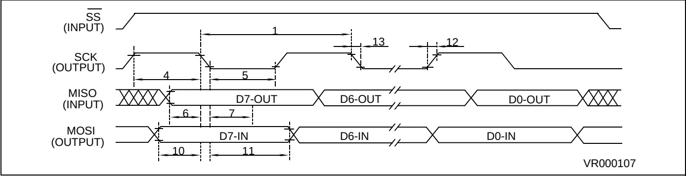
SPI Master Timing Diagram CPHA=1, CPOL=1
