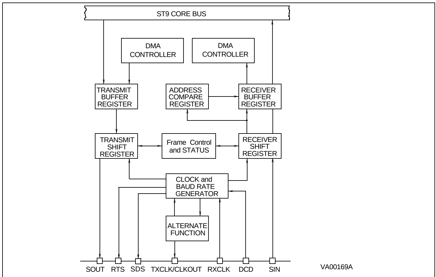
Figure 88. SCI-M Block Diagram
