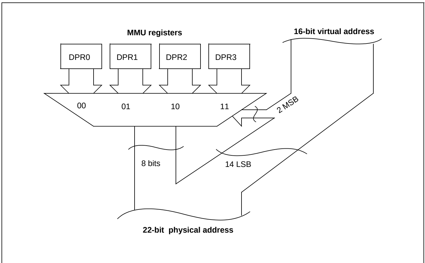
Figure 18. Addressing via DPR[3:0]
