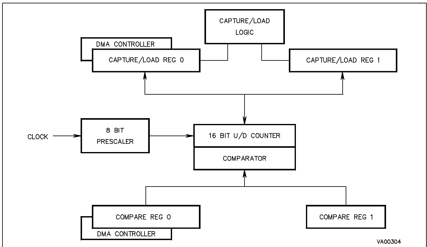
Figure 83. MFT Simplified Block Diagram
