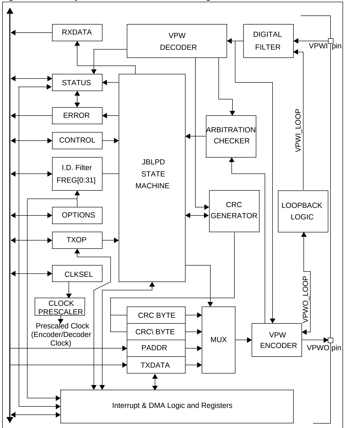
Figure 109. JBLPD Byte Level Protocol Decoder Block Diagram
