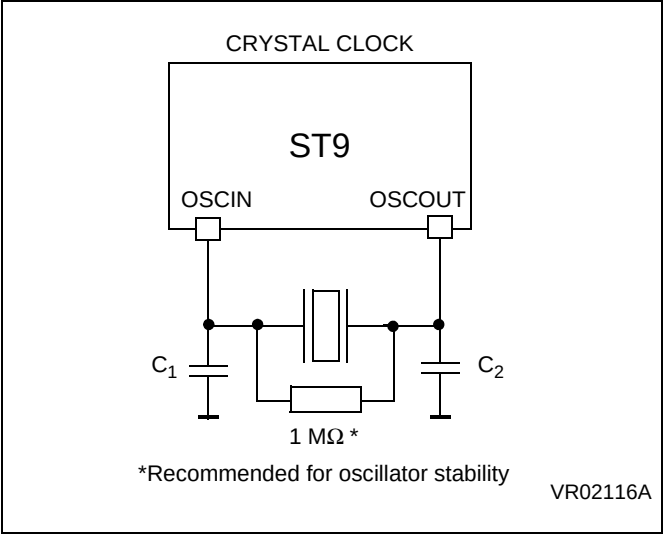
Figure 49. Crystal Oscillator
