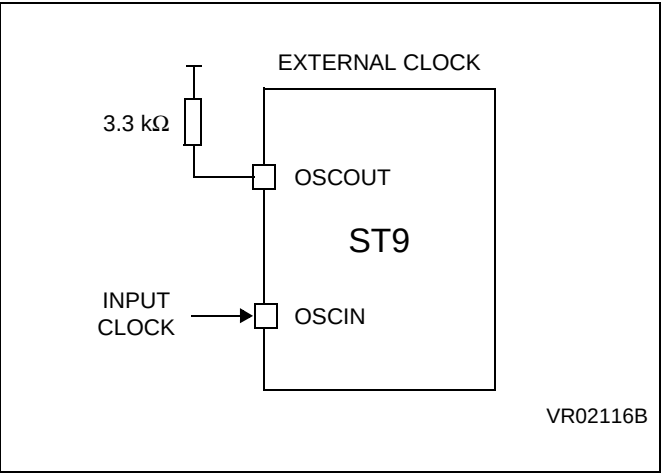
Figure 51. External Clock
