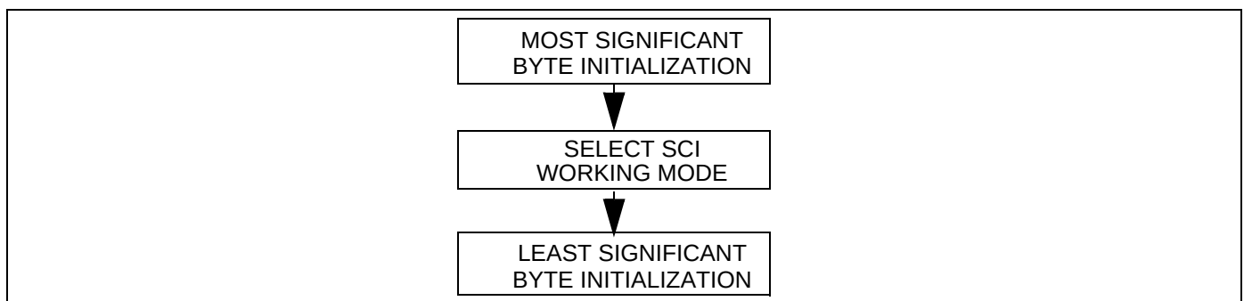
Figure 96. SCI-M Baud Rate Generator Initialization Sequence
