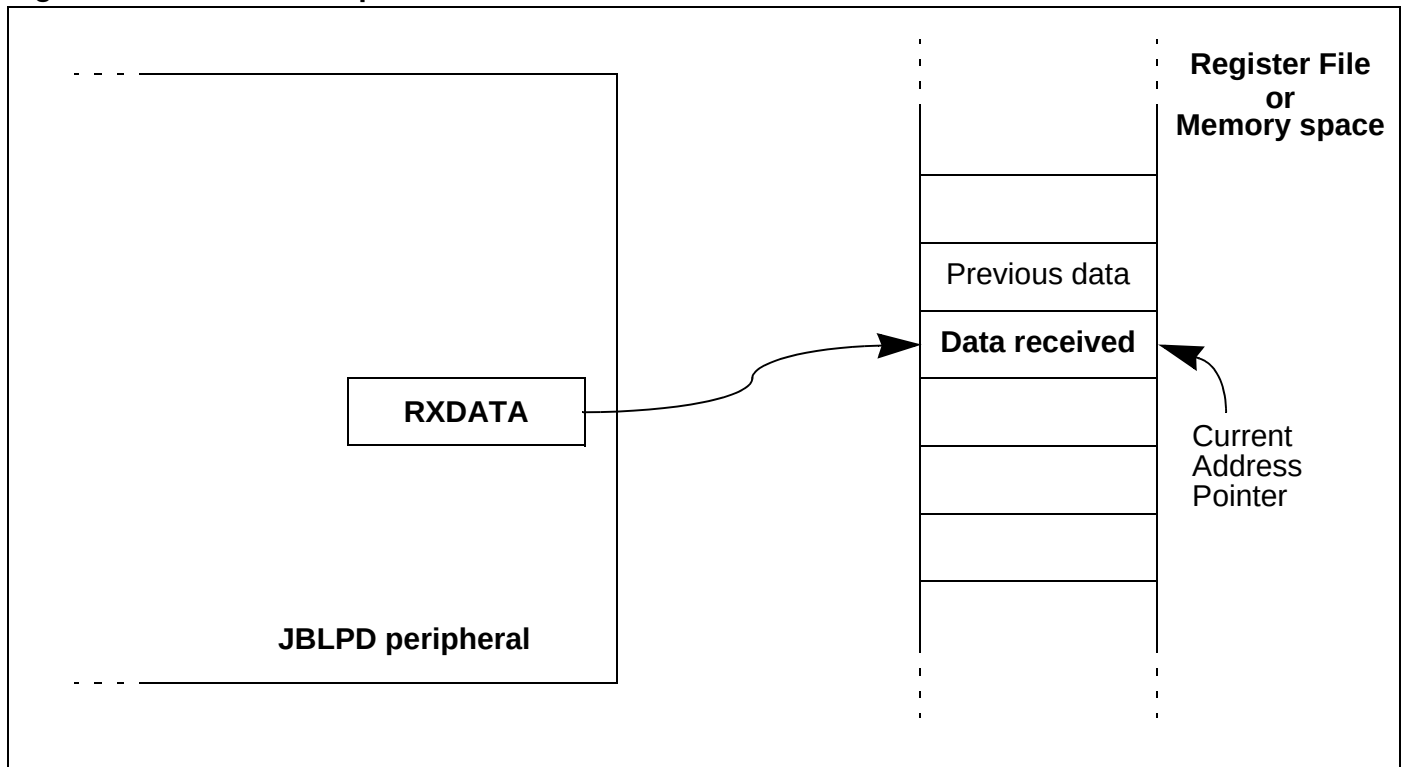
Figure 118. DMA in Reception Mode
