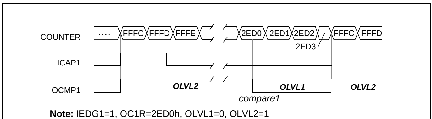
Figure 81. One Pulse Mode Timing
