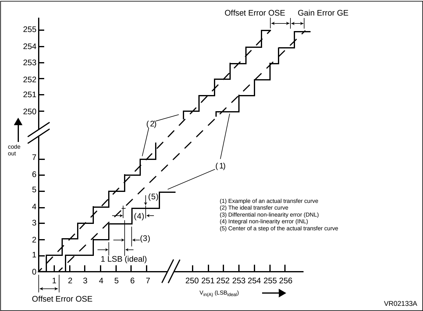
Figure 124. A/D Conversion Characteristics
