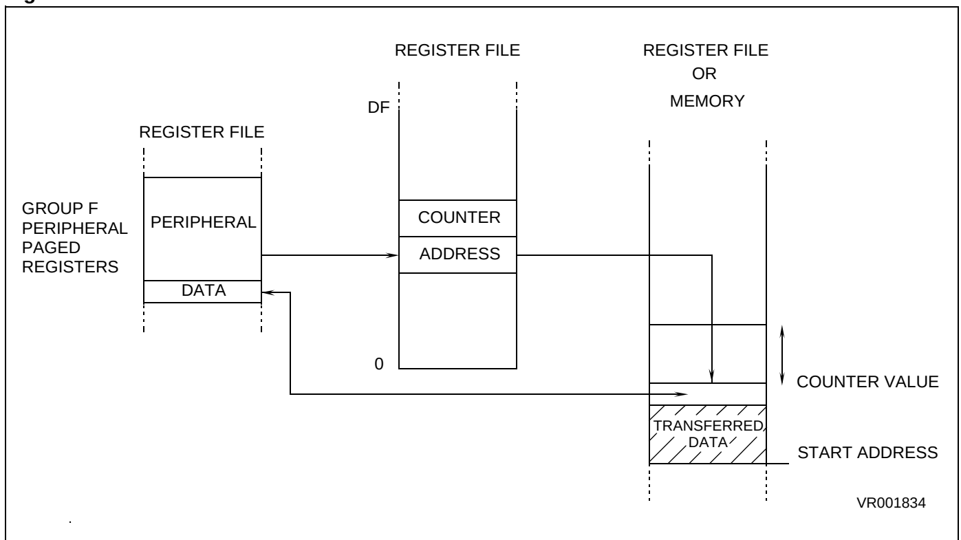
Figure 40. DMA Data Transfer
