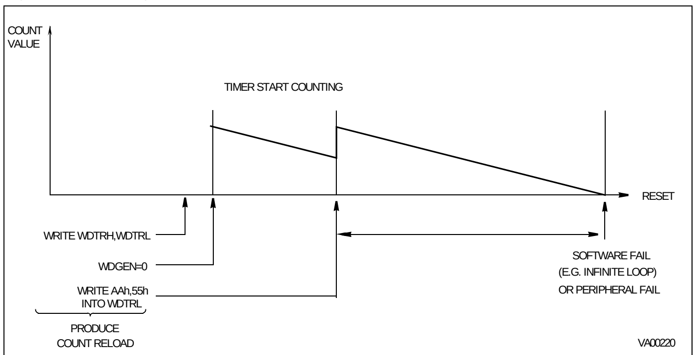
Figure 70. Watchdog Timer Mode
