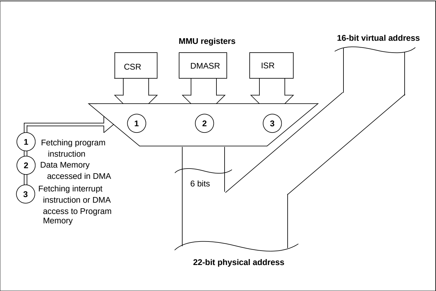
Figure 19. Addressing via CSR, ISR, and DMASR
