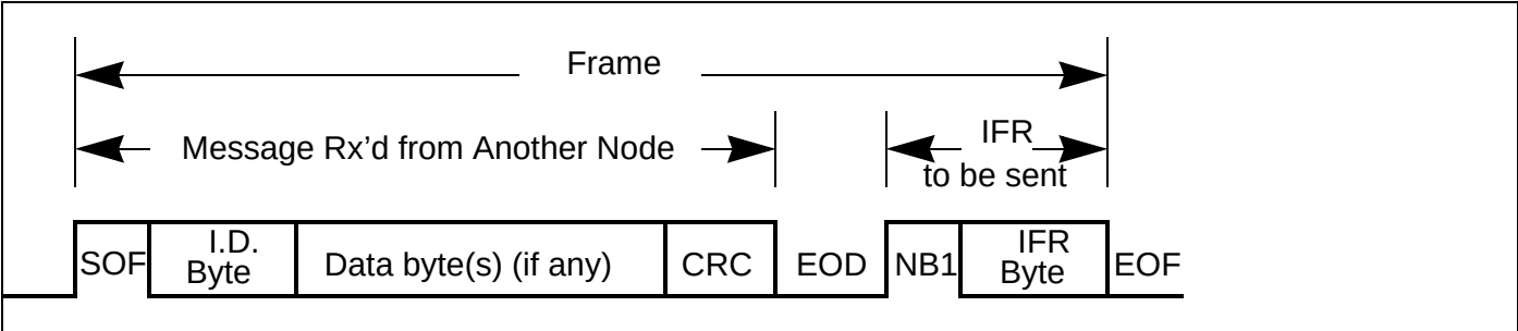
Figure 111. J1850 String Transmission Type 1
