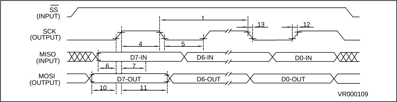
SPI Master Timing Diagram CPHA=0, CPOL=1
