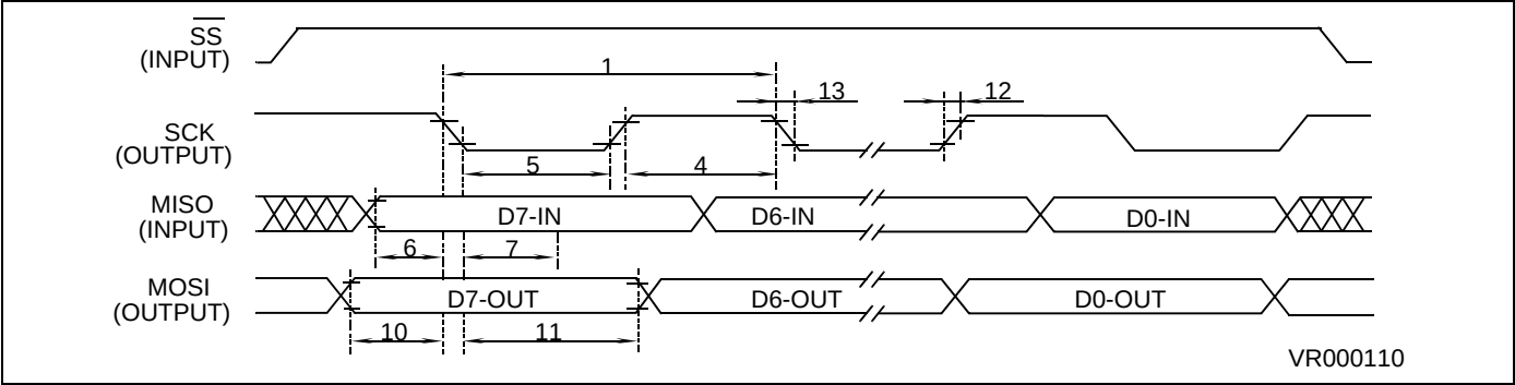
SPI Master Timing Diagram CPHA=1, CPOL=0
