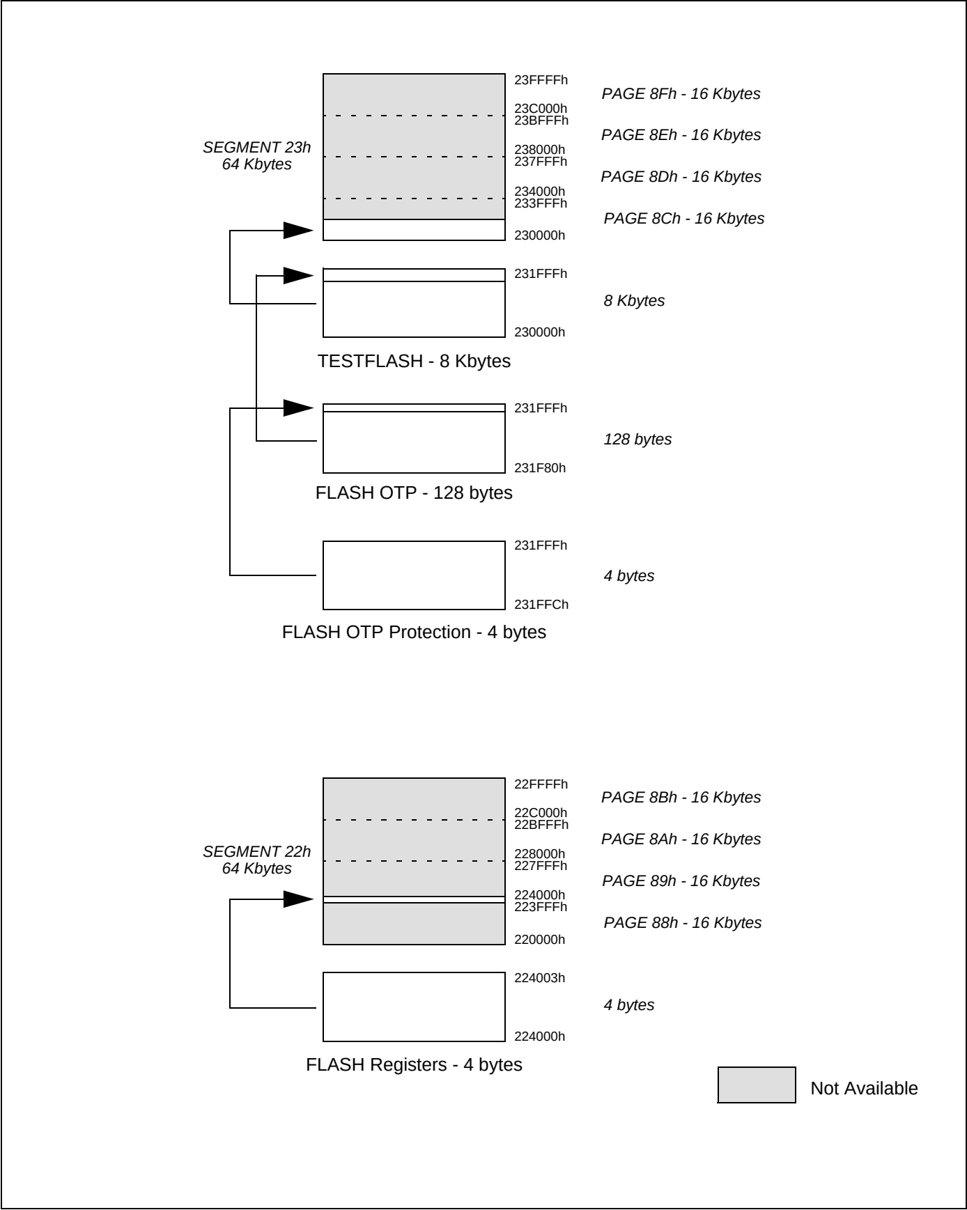
Figure 28. ST92F120JV1Q7/ST92F120V1Q7 User Memory Map (part 2)
