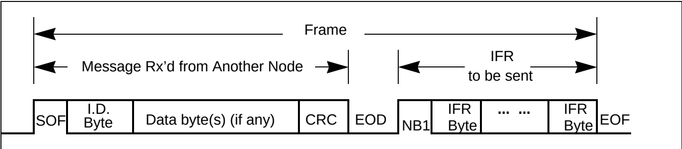
Figure 113. J1850 String Transmission Type 3
