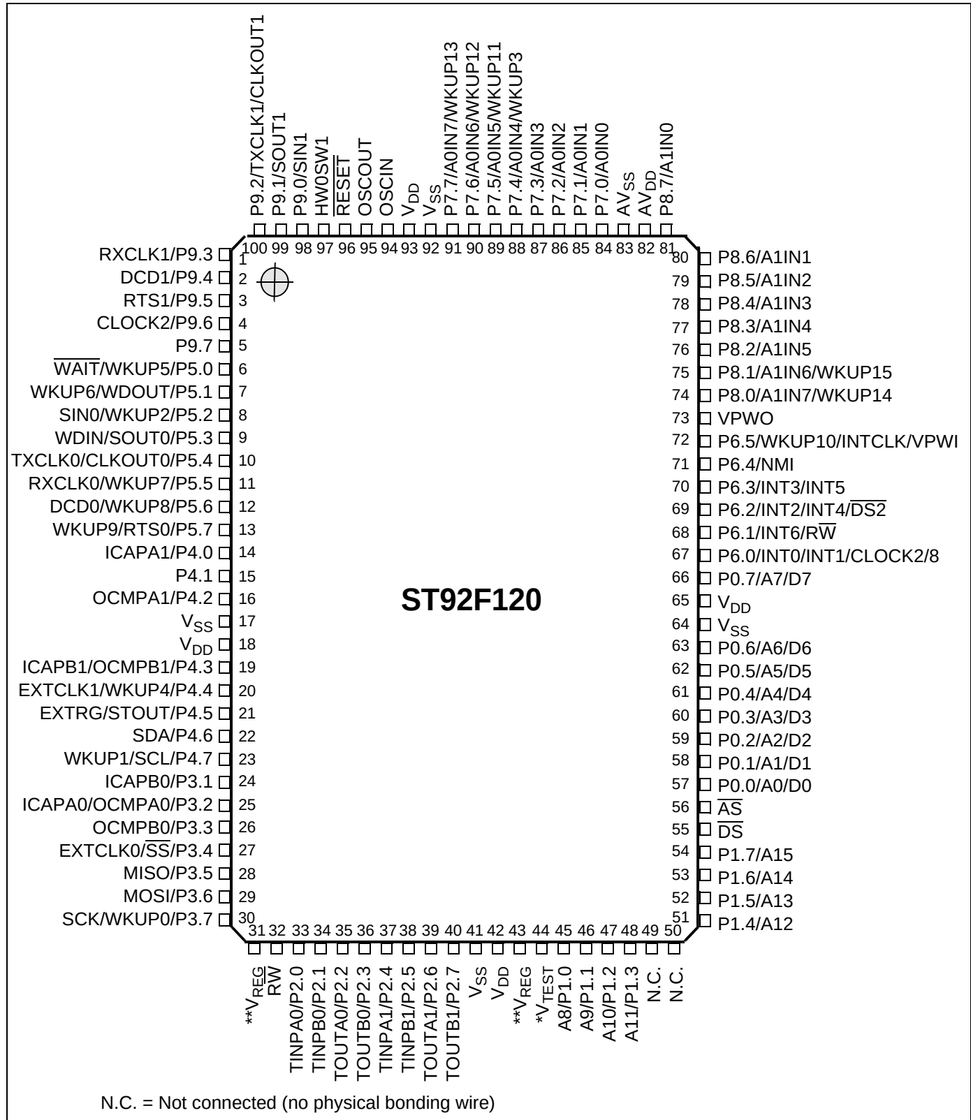
Figure 7. ST92F120: Pin Configuration (Top-view PQFP100)
