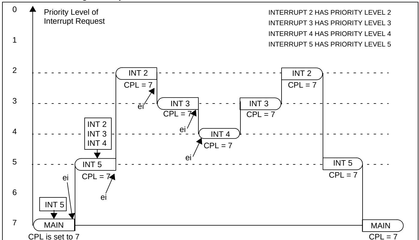
Figure 33. Complex Example of a Sequence of Interrupt Requests with:
