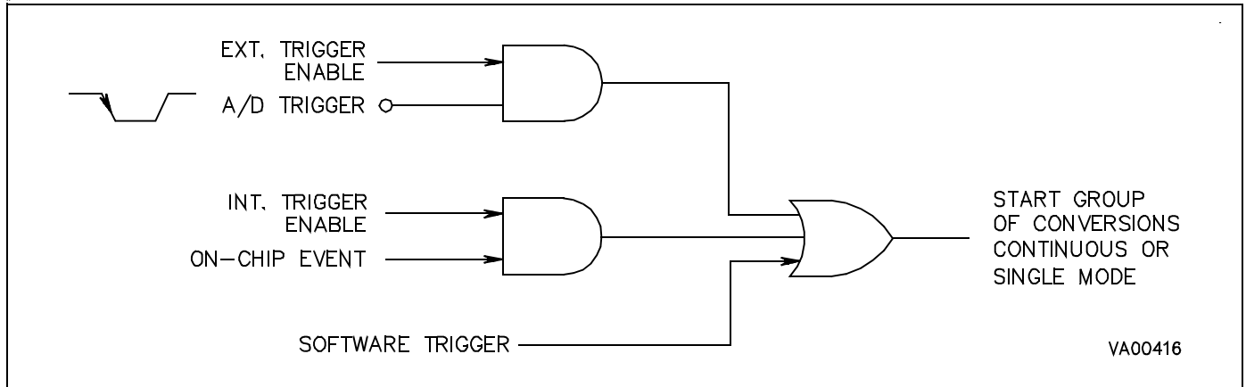
Figure 122. A/D Trigger Source
