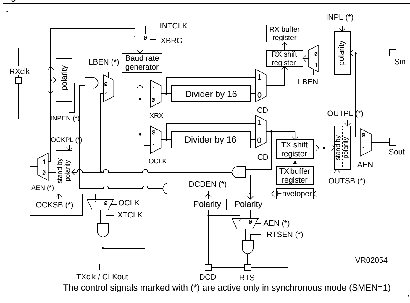
Figure 89. SCI -M Functional Schematic
