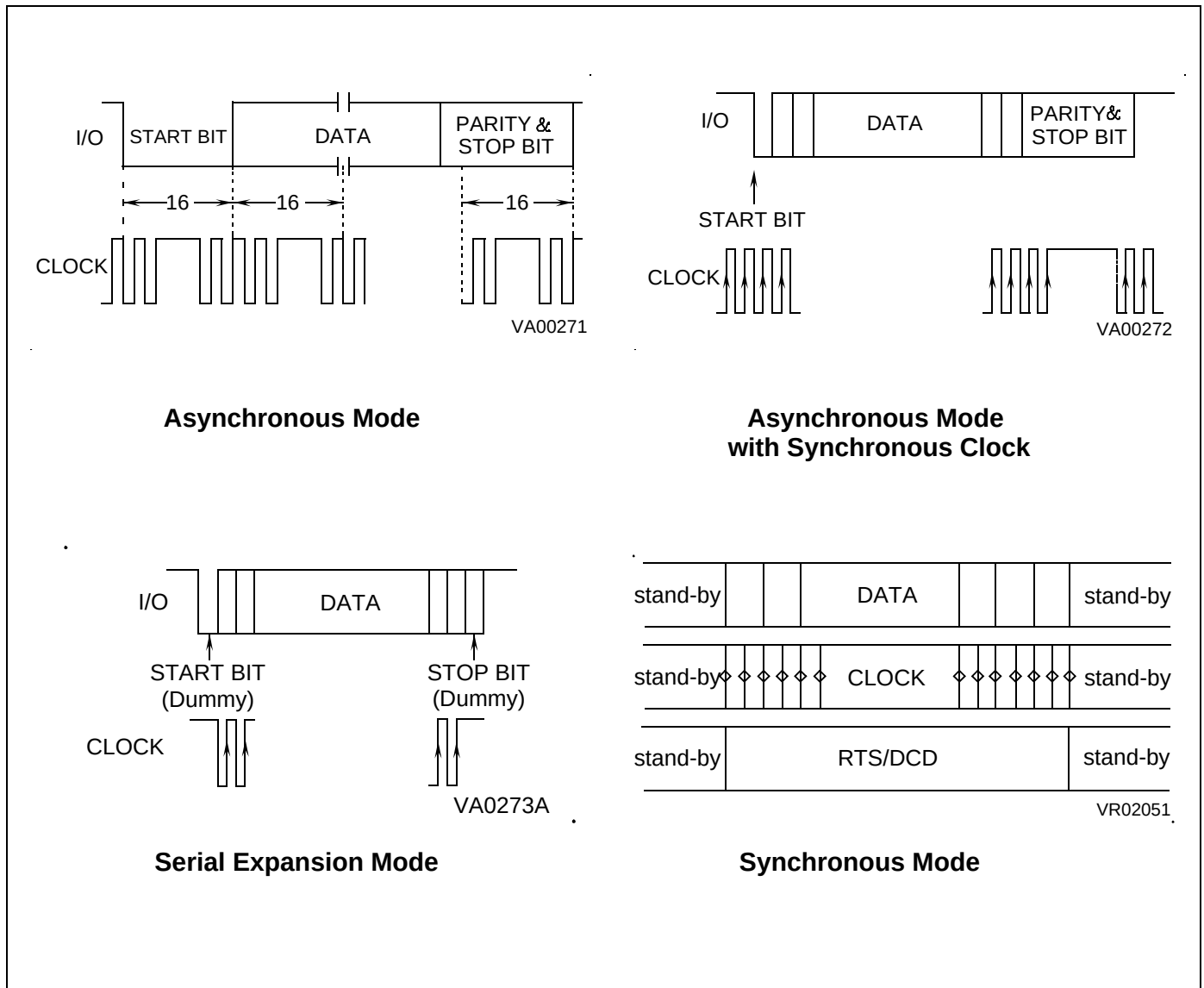
Figure 91. SCI -M Operating Modes
