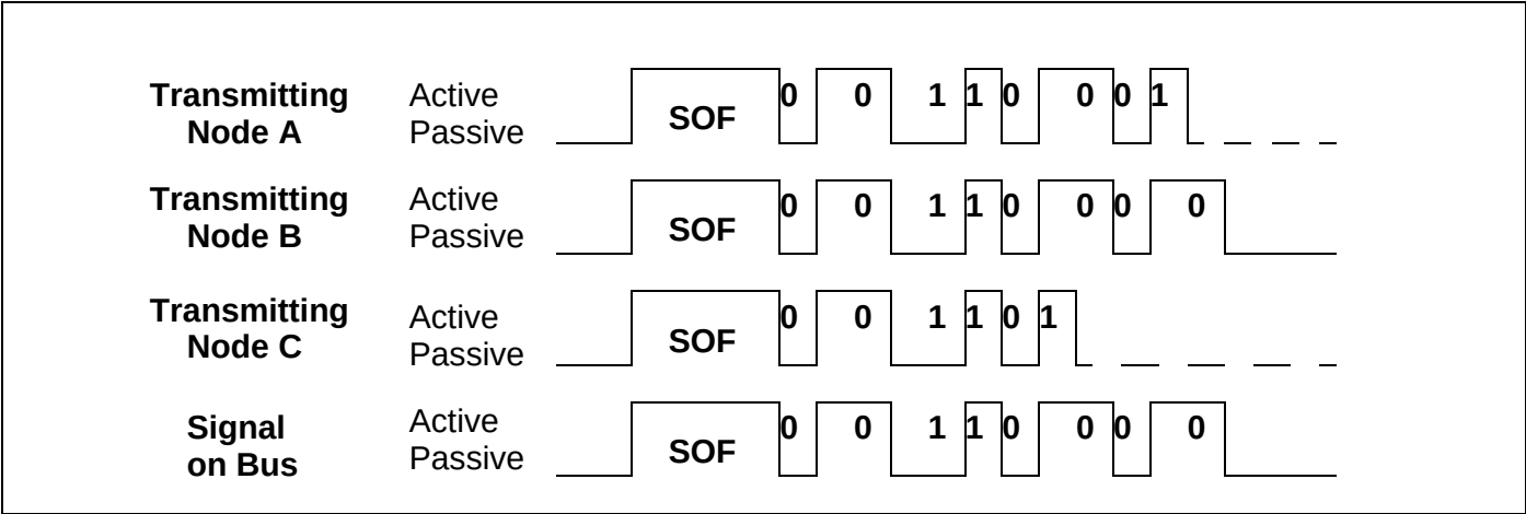
Figure 114. J1850 Arbitration Example
