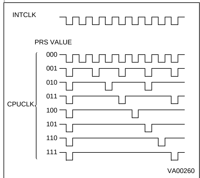
Figure 45. CPU Clock Prescaling
