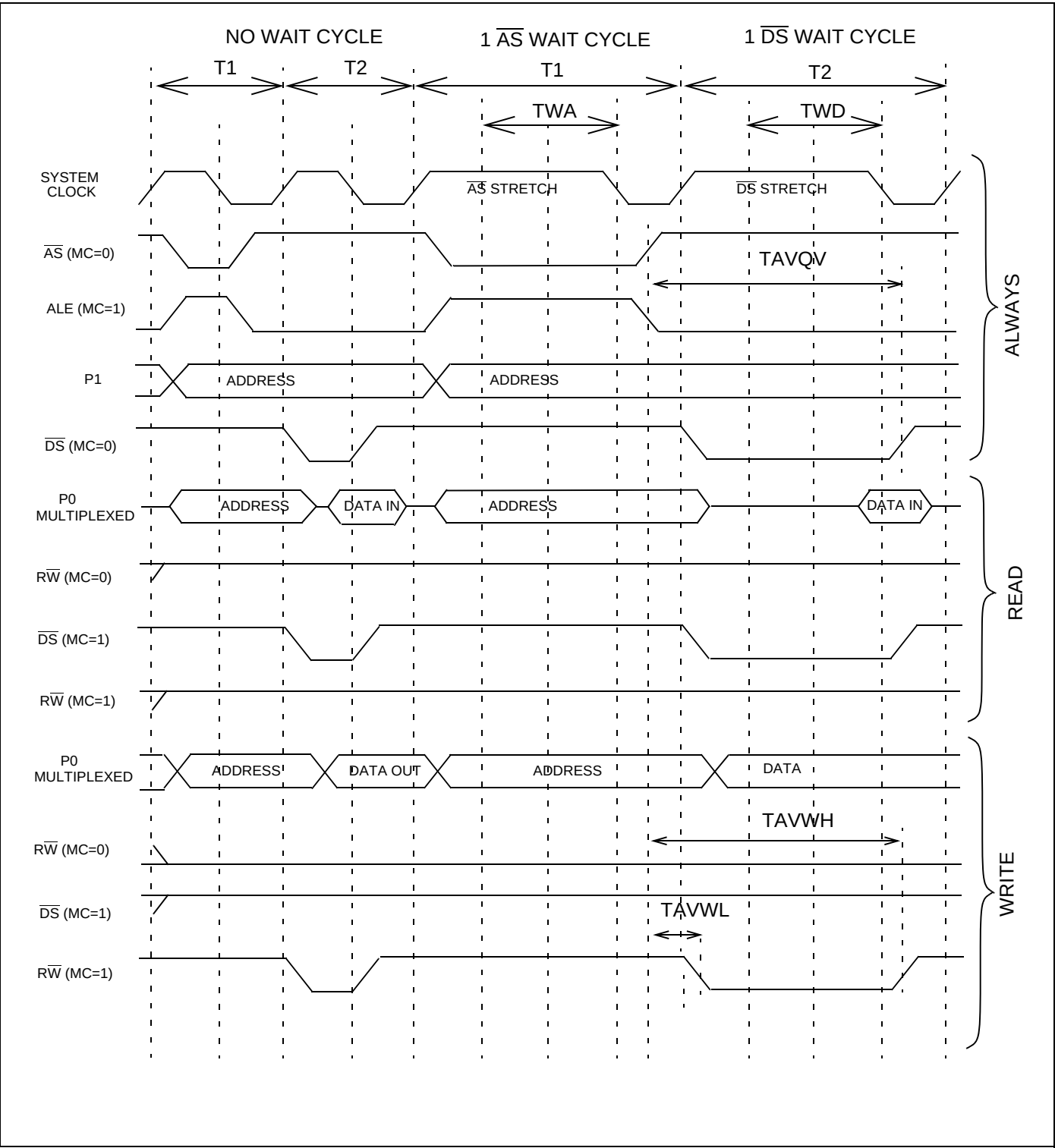
Figure 58. External Memory Read/Write with a Programmable Wait
