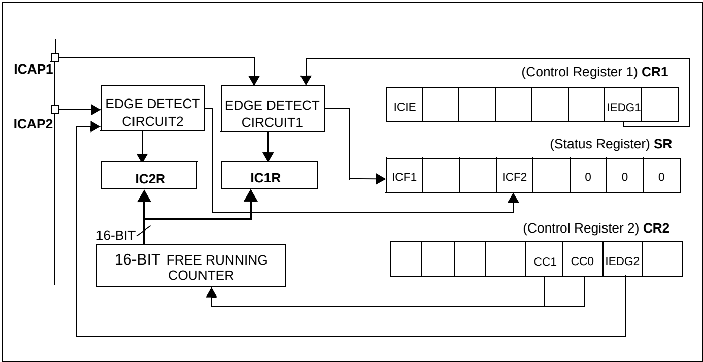
Figure 77. Input Capture Block Diagram
