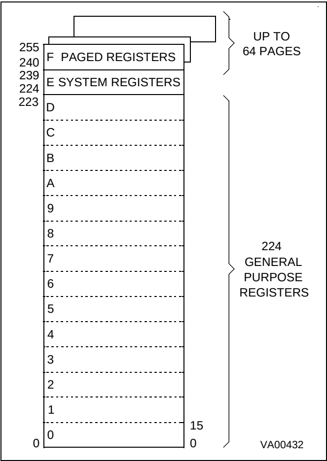
Figure 12. Addressing the Register File
