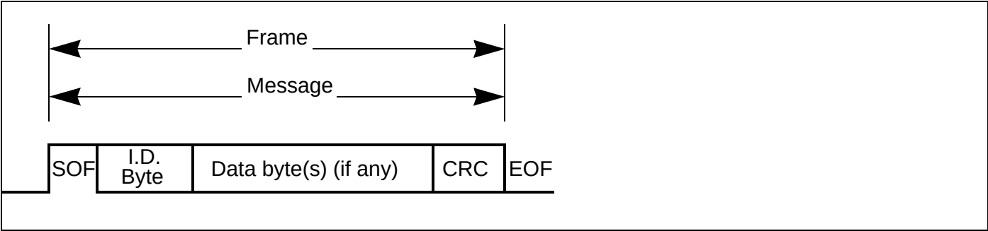
Figure 111. J1850 String Transmission Type 1
