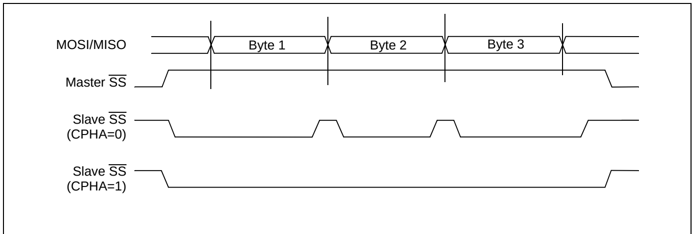
Figure 101. CPHA / \overline{SS} Timing Diagram
