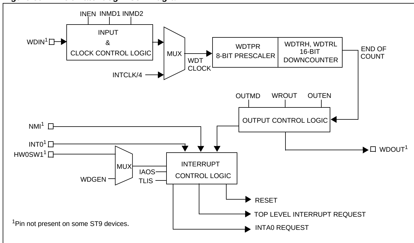
Figure 69. Timer/Watchdog Block Diagram
