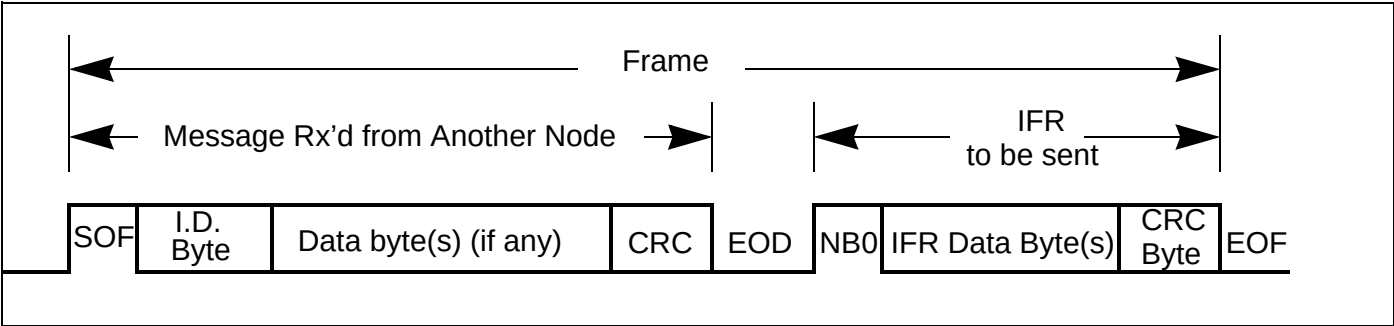
Figure 113. J1850 String Transmission Type 3
