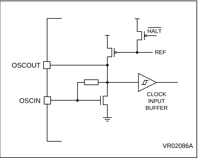
Figure 51. External Clock
