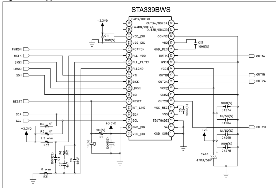
Figure 21. Applications circuit
