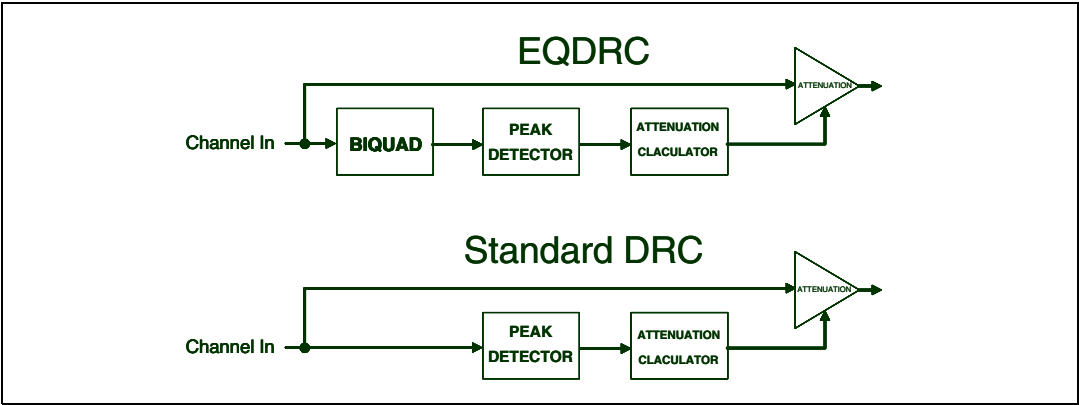
Figure 20. EQDRC scheme
