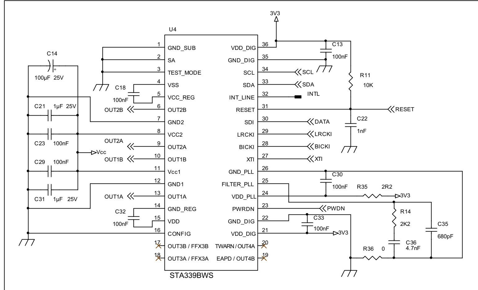
Figure 22. Applications circuit
