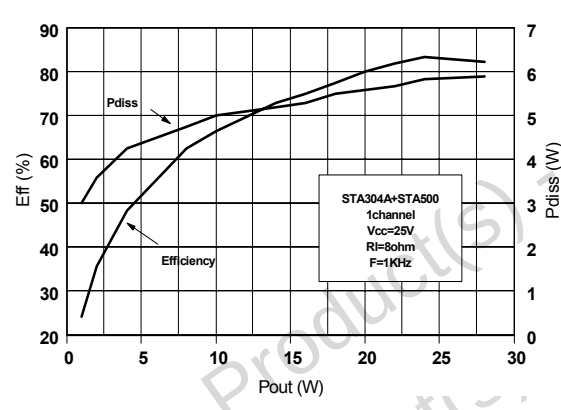
Figure 6. Total Power Dissipation & Efficiency vs Output Power
