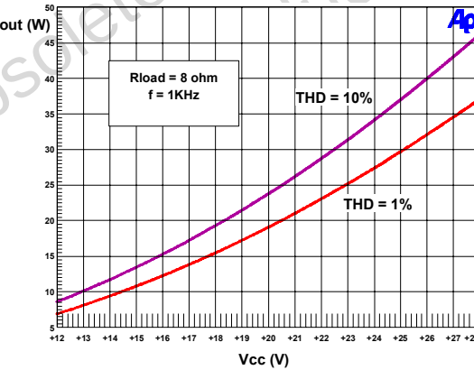
Figure 8. Output Power vs Supply Voltage (STA304A+STA500)
