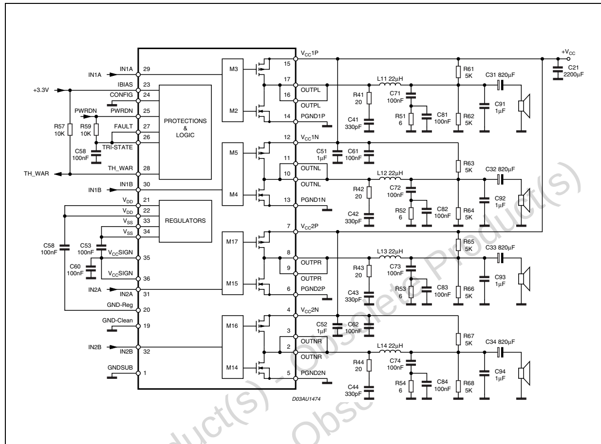
Figure 4. Typical Quad Half Bridge Configuration
