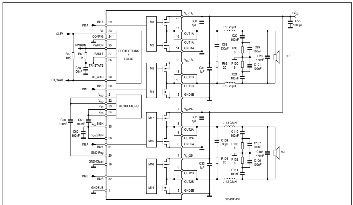
Figure 2. Audio Application Circuit (Dual BTL) Pin Description
