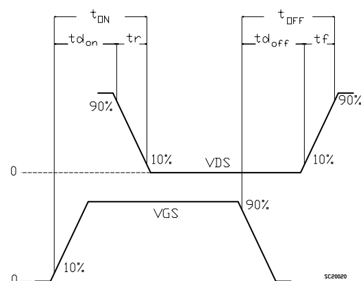
Figure 22. Switching time waveform
