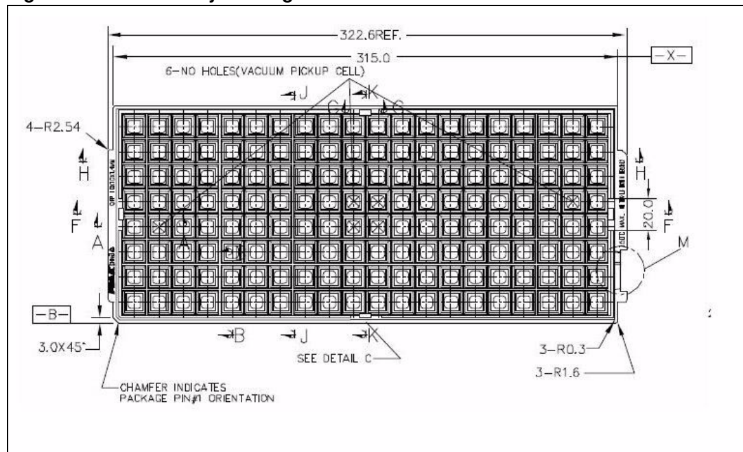
Figure 23. TQFP64 tray drawing
