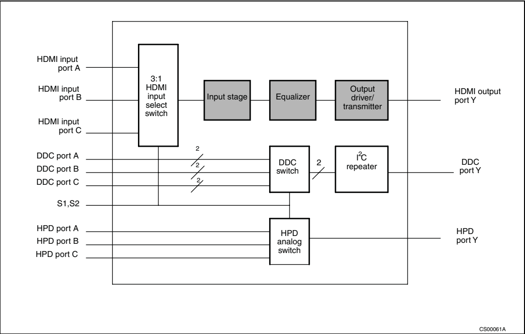
Figure 1. STDVE103A block diagram
