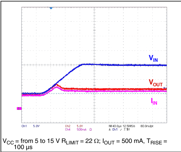
Figure 17. Line transient
