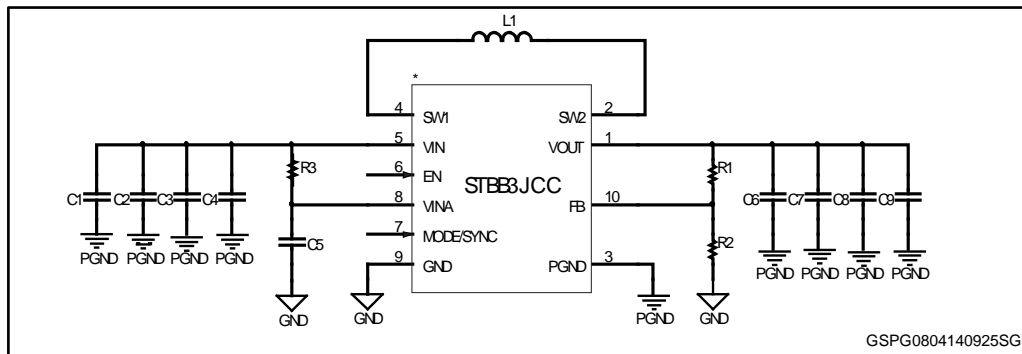
Figure 1: STEVAL-ISA141V2 circuit schematic
