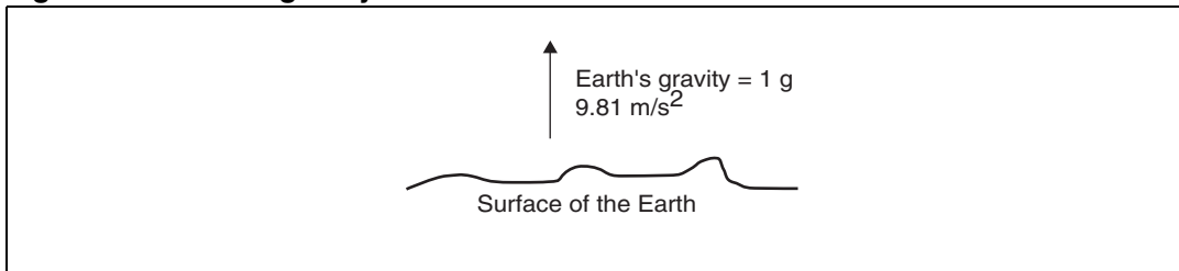
Figure 21. Earth's gravity
