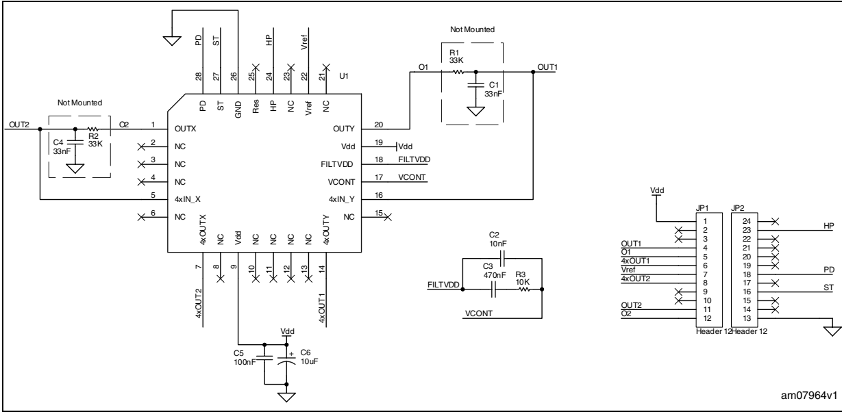
Figure 1. Internal schematic
