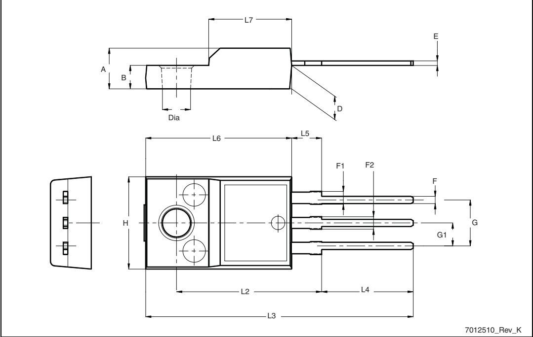
Figure 30. TO-220FP drawing
