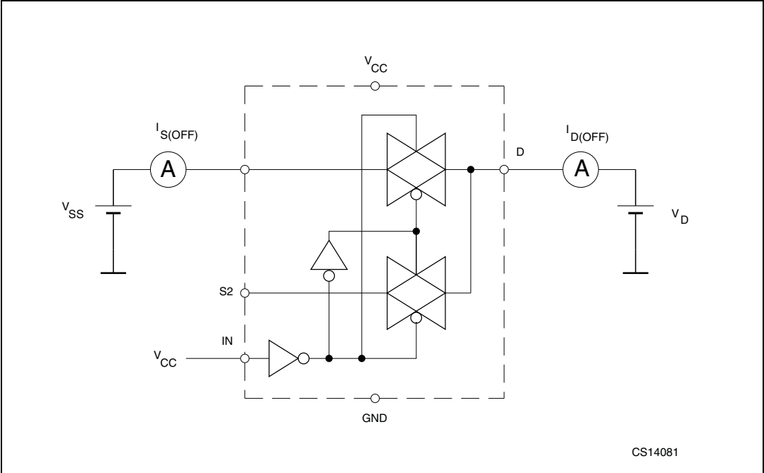
Figure 6. OFF leakage
