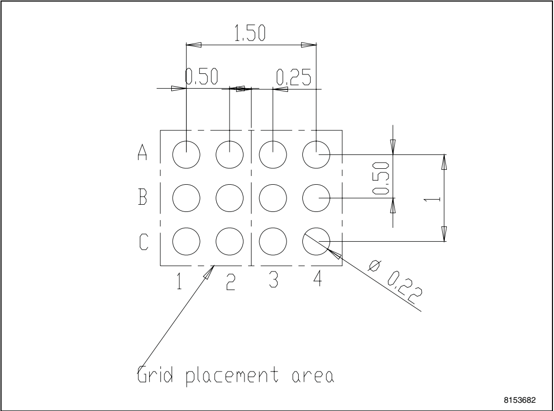
Figure 14. Footprint recommendation
