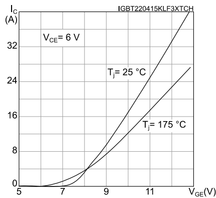
Figure 10: Transfer characteristics
