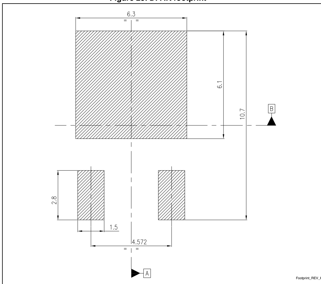
Figure 23. DPAK footprint (b)
