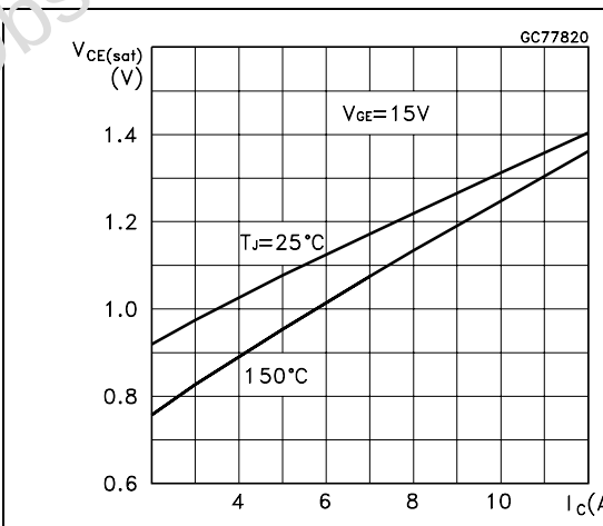
Figure 6. Collector-emitter on voltage vs collector current
