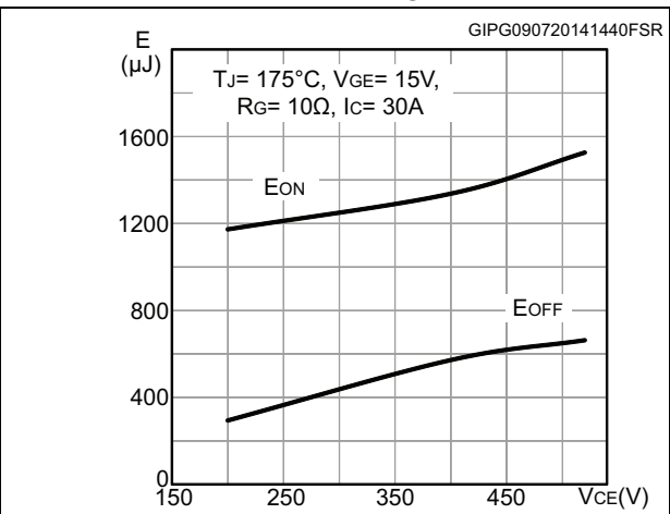
Figure 19. Switching energy vs collector-emitter voltage
