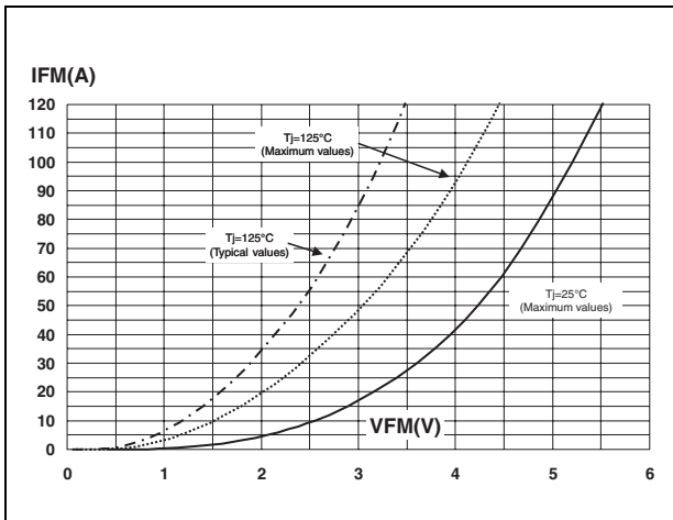
Figure 16. Emitter-collector diode characteristics
