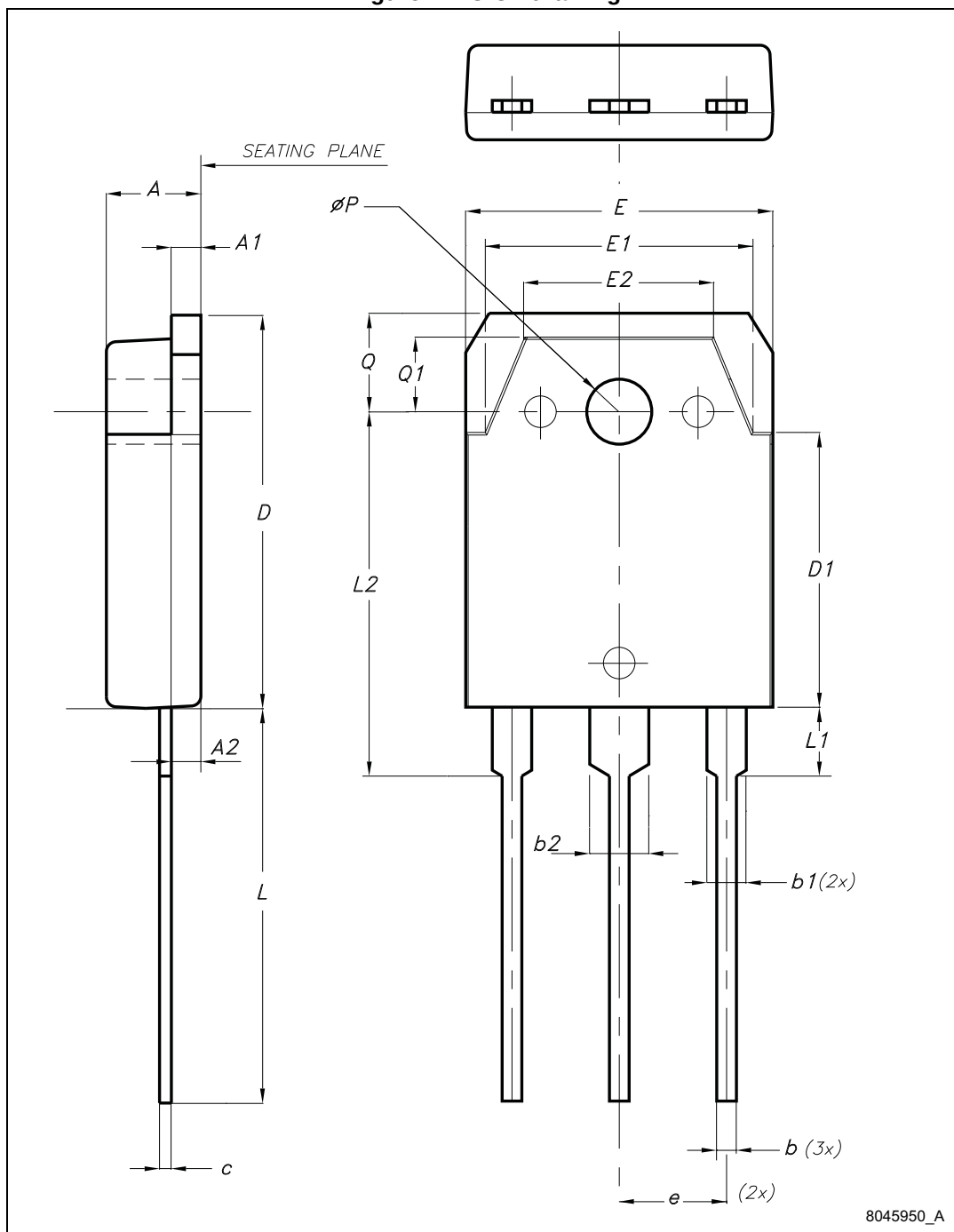
Figure 7. TO-3P drawing
