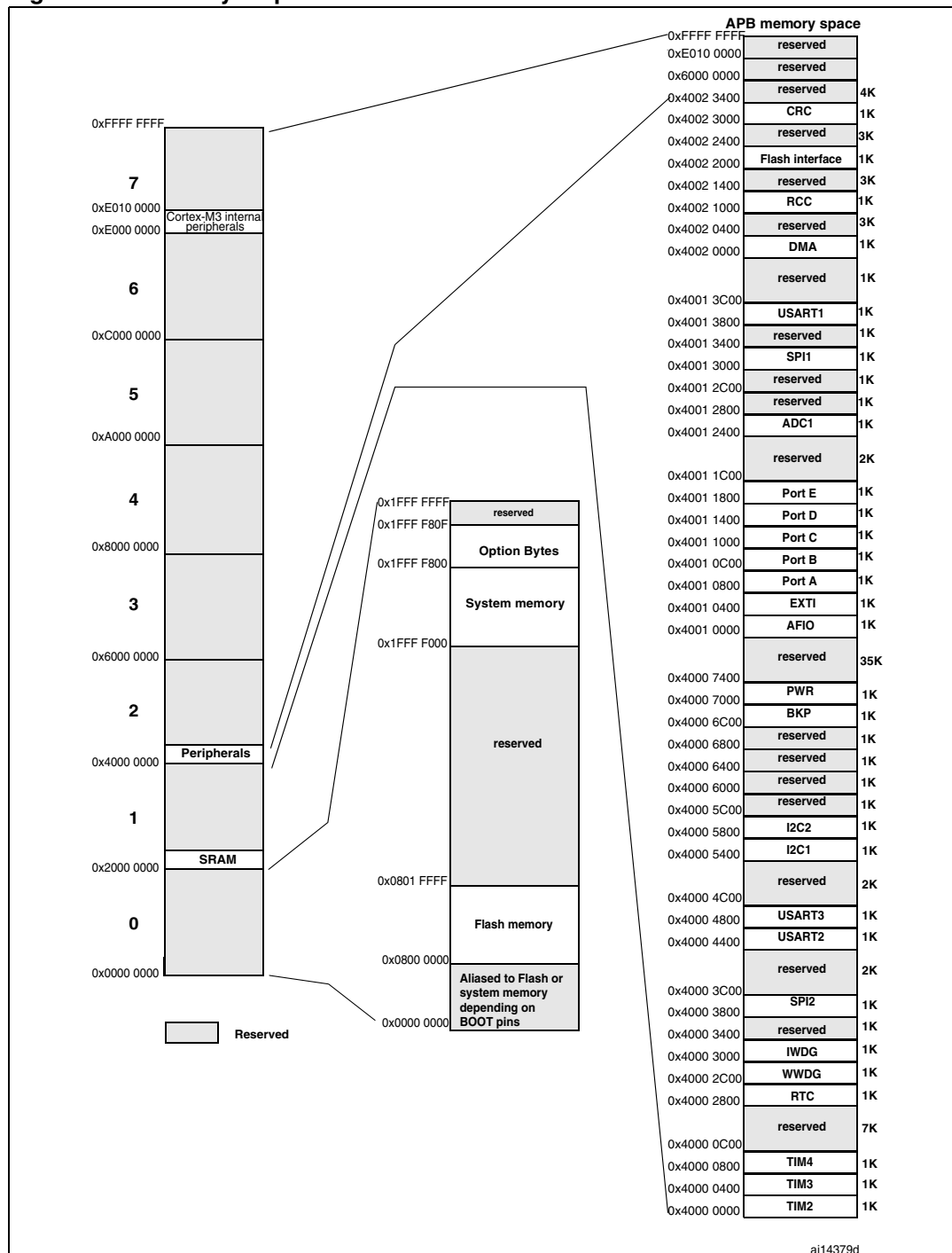
Figure 7. Memory map
