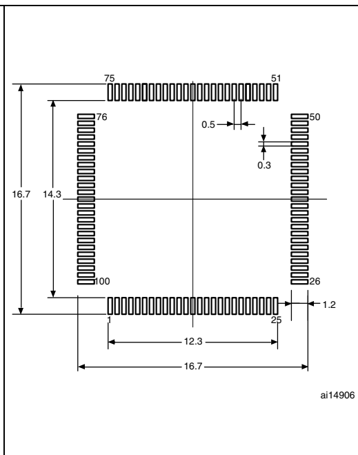
Figure 34. Recommended footprint (1)(2)
