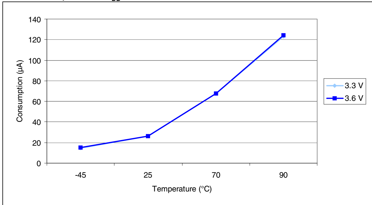
Figure 14. Typical current consumption in Stop mode with regulator in Run mode versus temperature at V_{DD} = 3.3\text{ V} and 3.6\text{ V}
