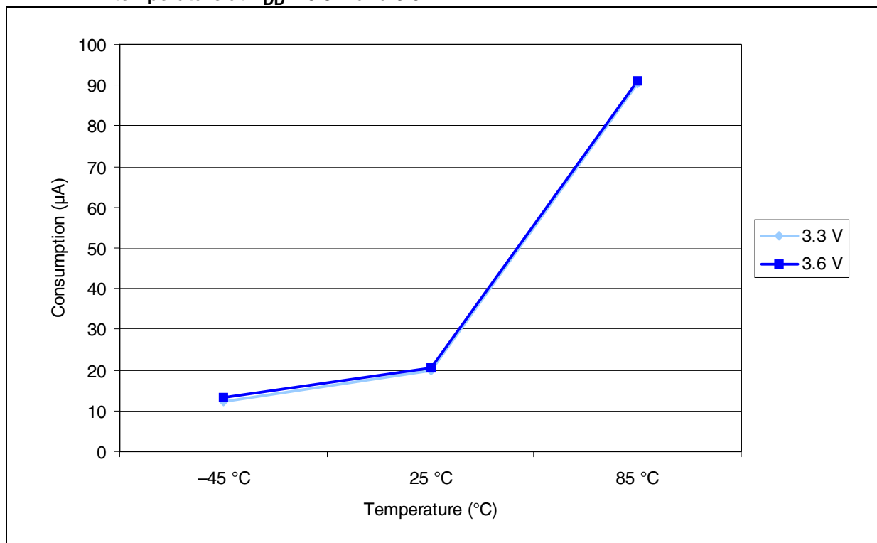
Figure 15. Typical current consumption in Stop mode with regulator in Low-power mode versus temperature at V_{DD} = 3.3\text{ V} and 3.6\text{ V}
