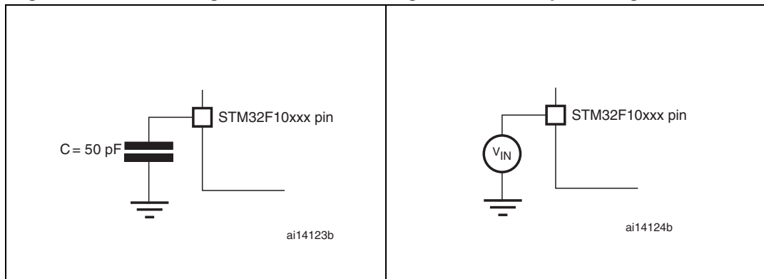
Figure 9. Pin input voltage
