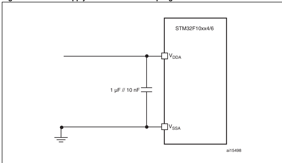
Figure 28. Power supply and reference decoupling
