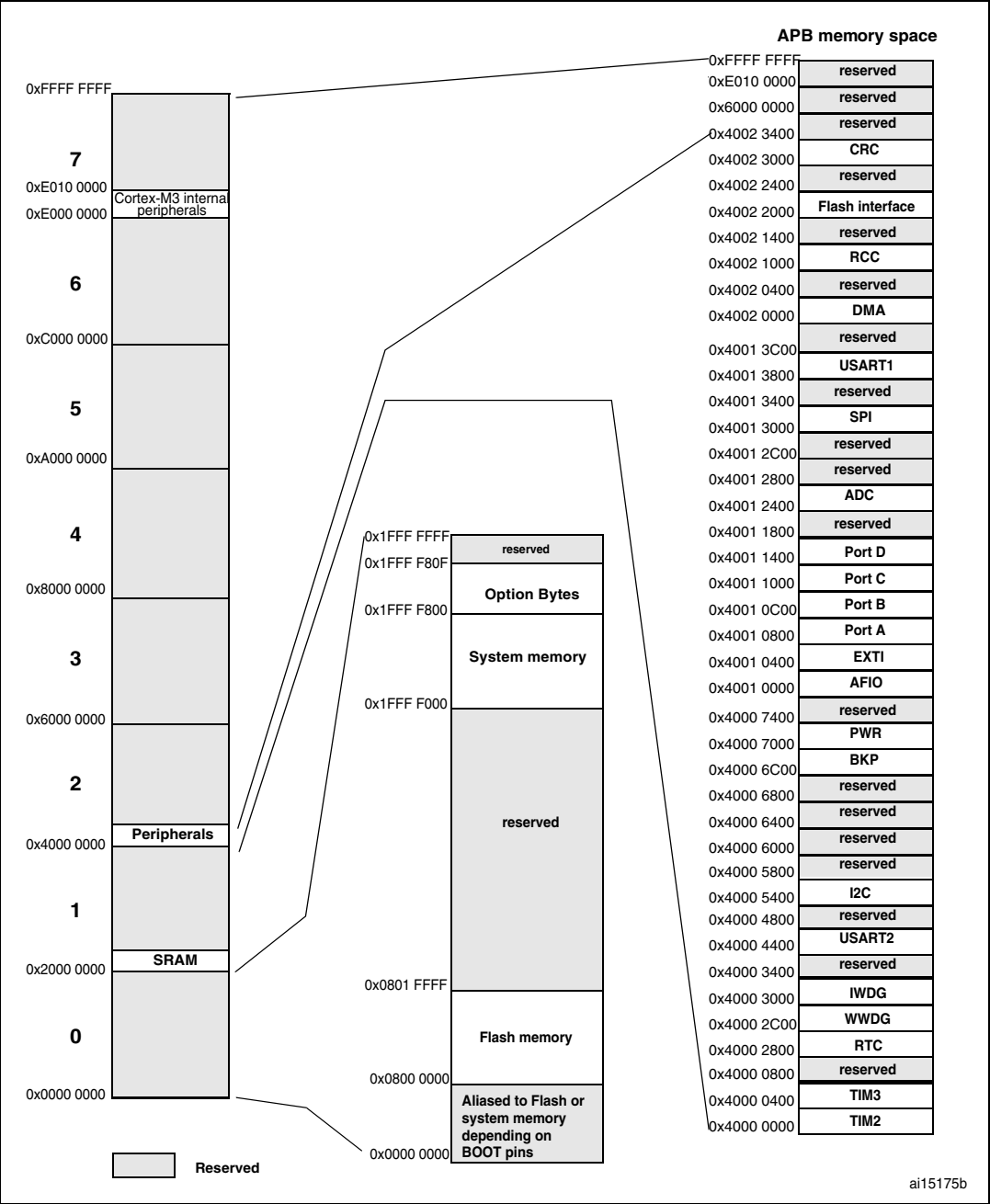
Figure 6. Memory map
