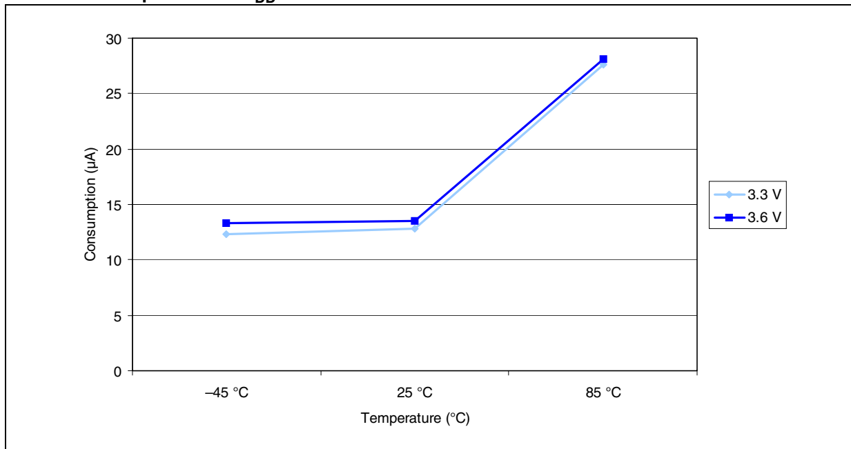
Figure 14. Typical current consumption in Stop mode with regulator in Low-power mode versus temperature at V_{DD} = 3.3\text{ V} and 3.6\text{ V}
