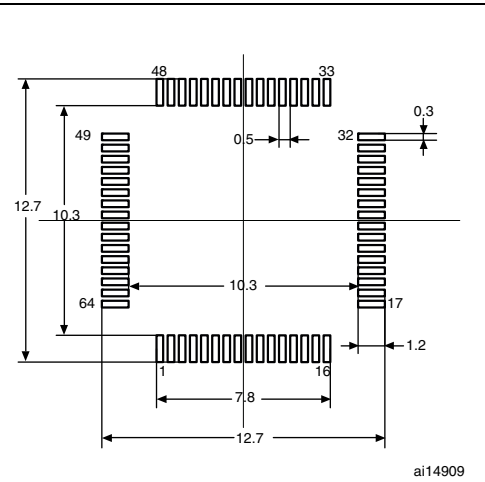
Figure 32. Recommended footprint (1)(2)
