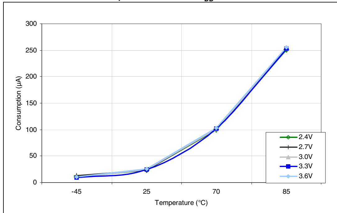
Figure 14. Typical current consumption in Stop mode with regulator in low-power mode versus temperature at different V_{DD} values
