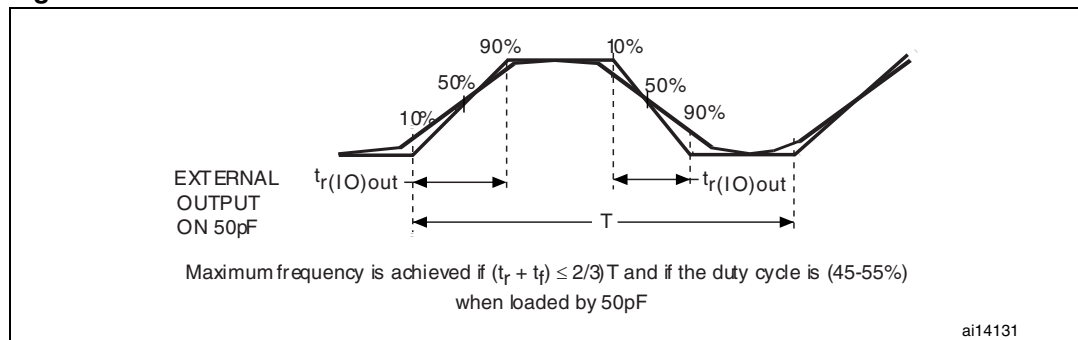
Figure 38. I/O AC characteristics definition
