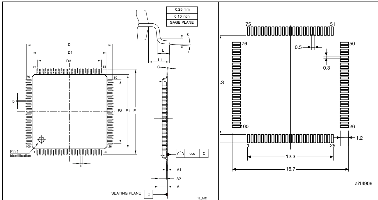
Figure 51. LQFP100 – 14 x 14 mm, 100-pin low-profile quad flat package outline (1) Figure 52. Recommended footprint (1)(2)
