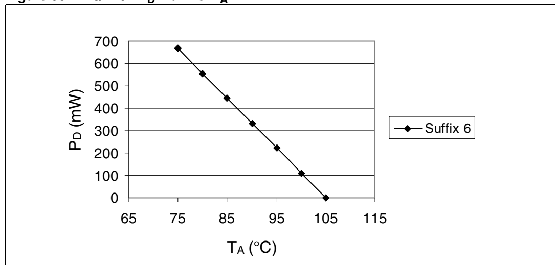
Figure 55. LQFP64 P_D max vs. T_A
