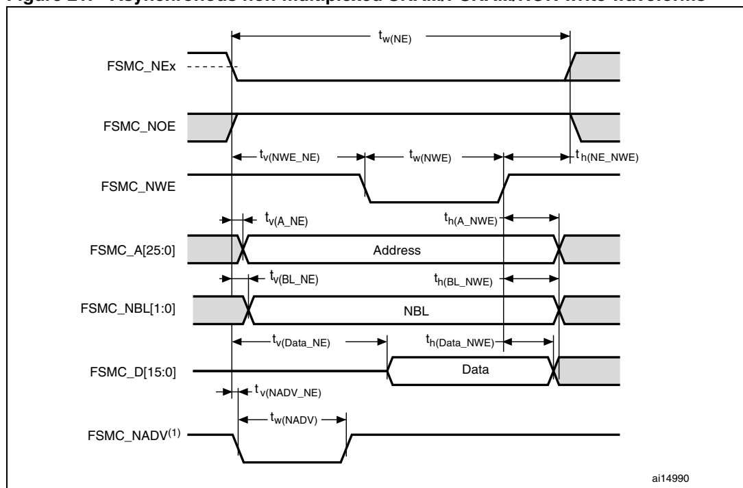
Figure 21. Asynchronous non-multiplexed SRAM/PSRAM/NOR write waveforms
