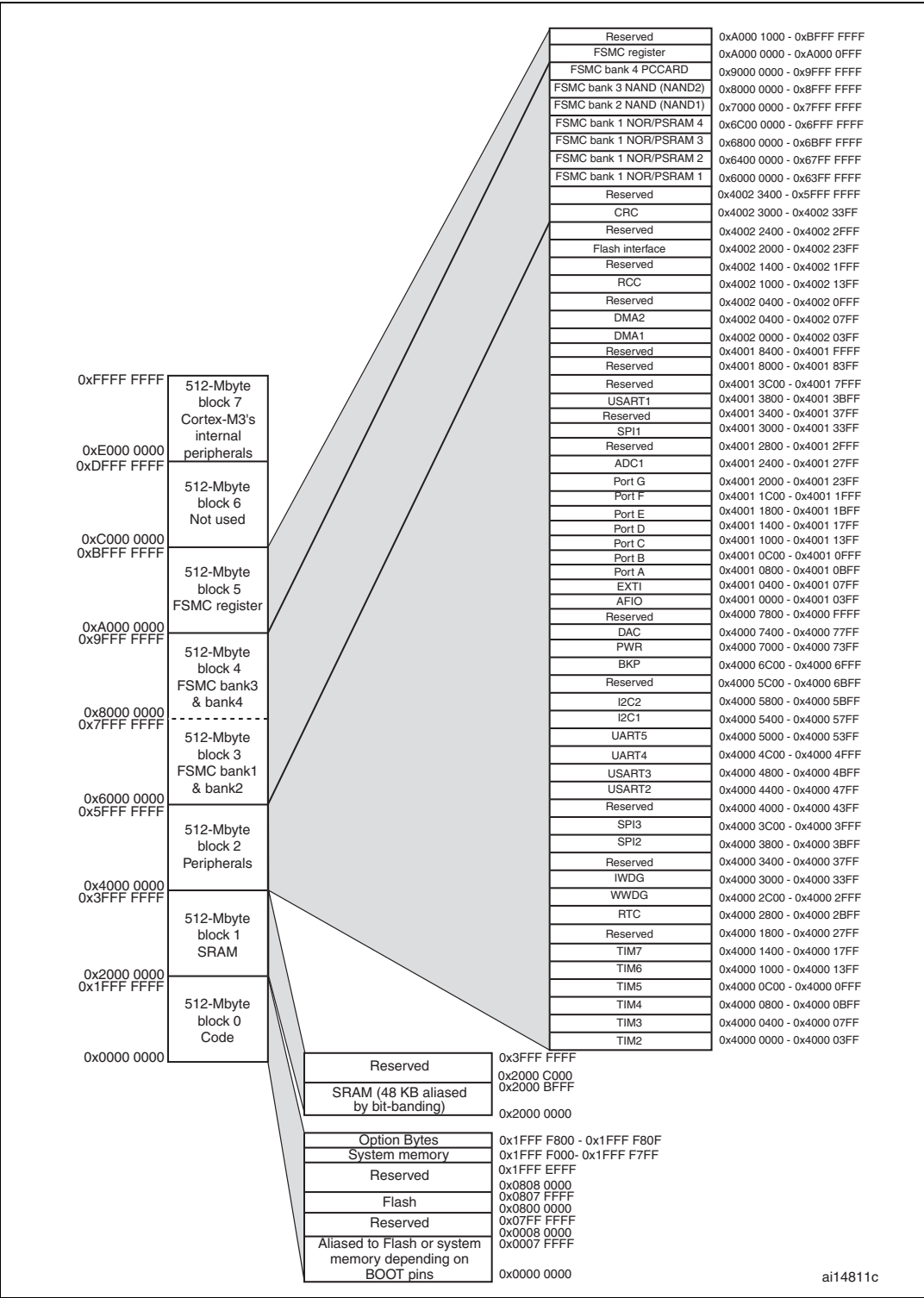
Figure 6. Memory map
