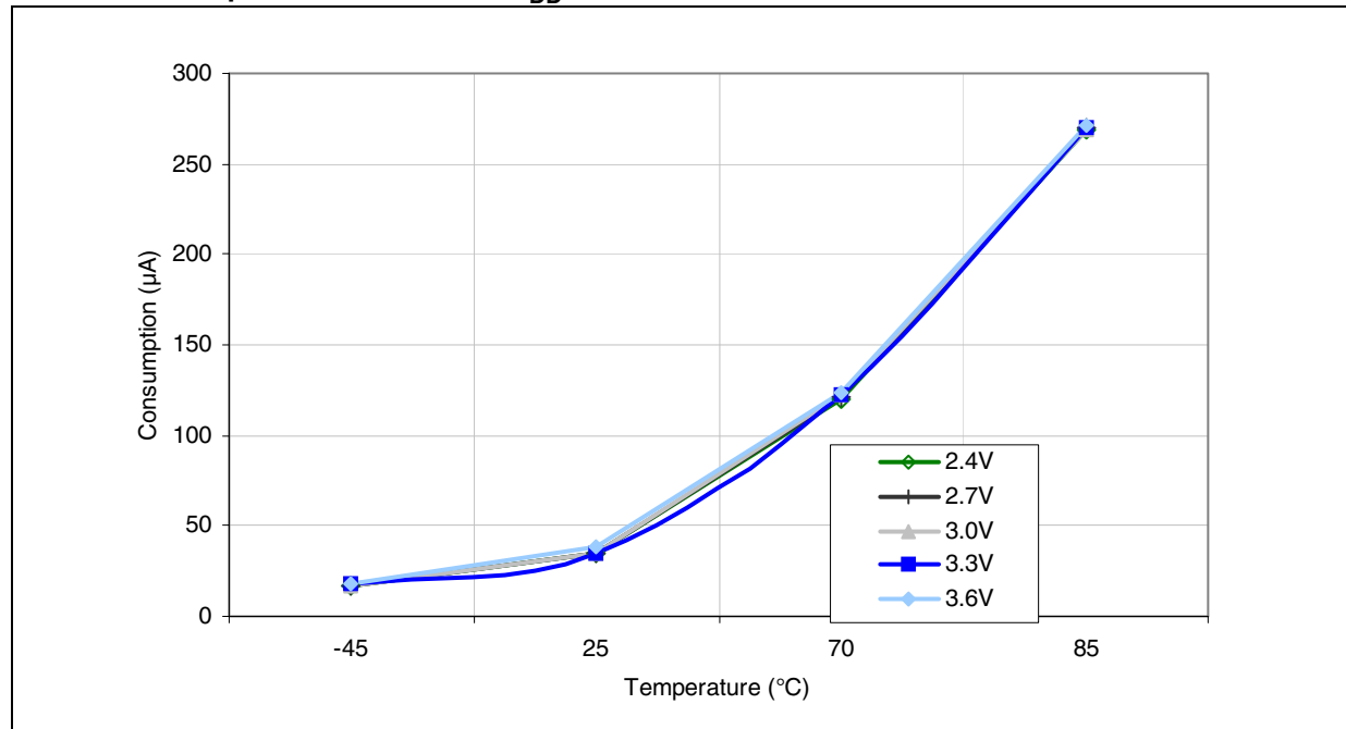
Figure 13. Typical current consumption in Stop mode with regulator in run mode versus temperature at different V_{DD} values
