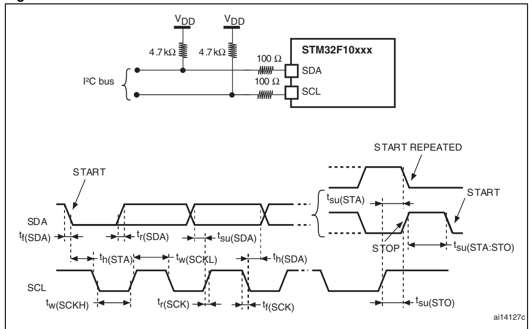
Figure 40. I 2 C bus AC waveforms and measurement circuit (1)
