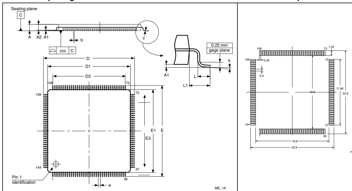
Figure 49. LQFP144, 20 x 20 mm, 144-pin thin quad flat package outline (1)
