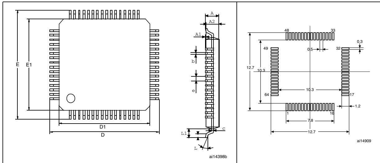
Figure 53. LQFP64 – 10 x 10 mm, 64 pin low-profile quad flat package outline (1) Figure 54. Recommended footprint (1)(2)
