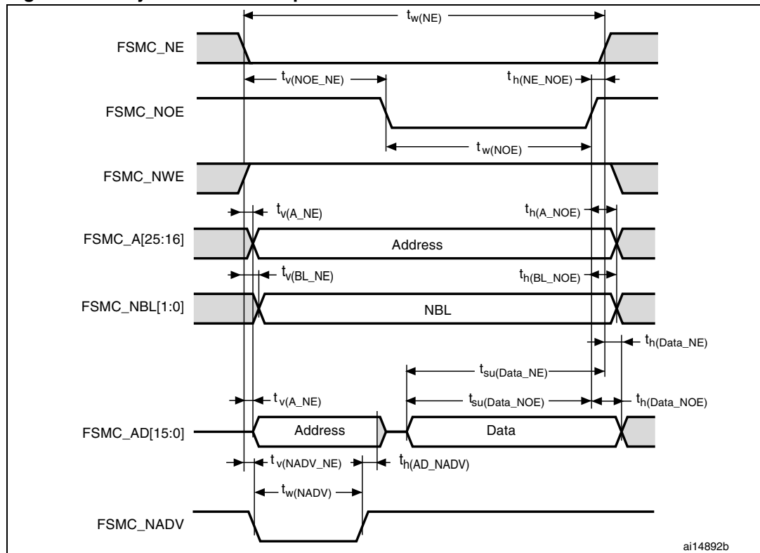
Figure 22. Asynchronous multiplexed NOR/PSRAM read waveforms
