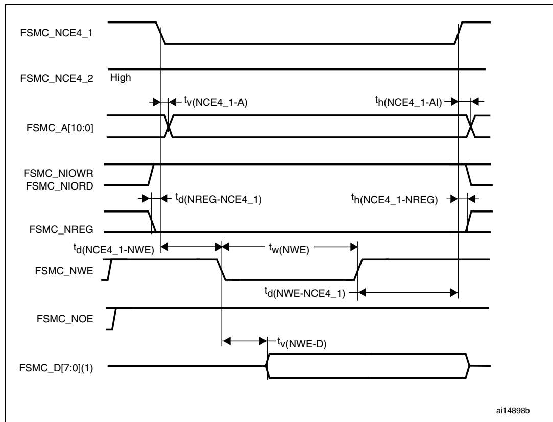
Figure 31. PC Card/CompactFlash controller waveforms for attribute memory write access
