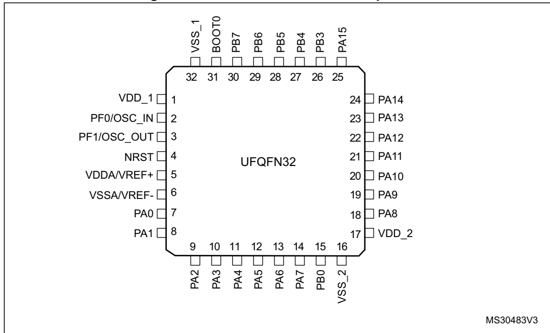
Figure 4. STM32F301x6/x8 UFQFN32 pinout
