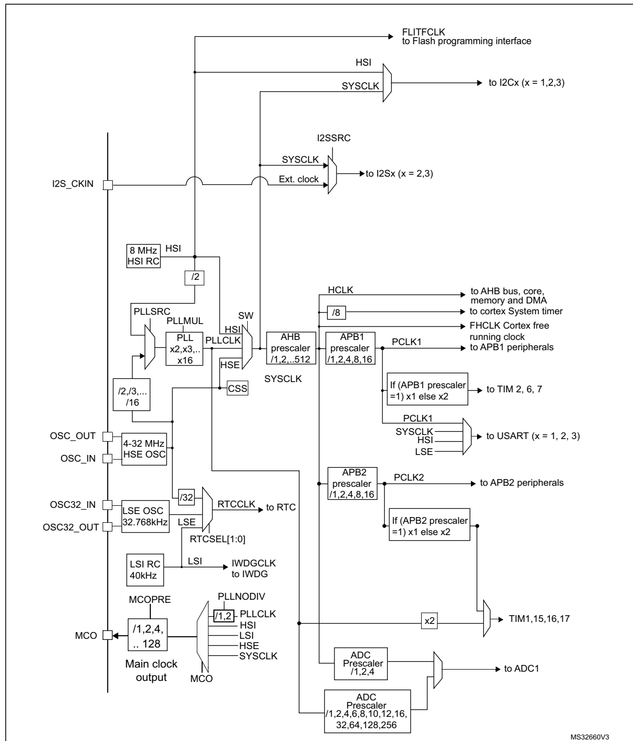
Figure 2. Clock tree
