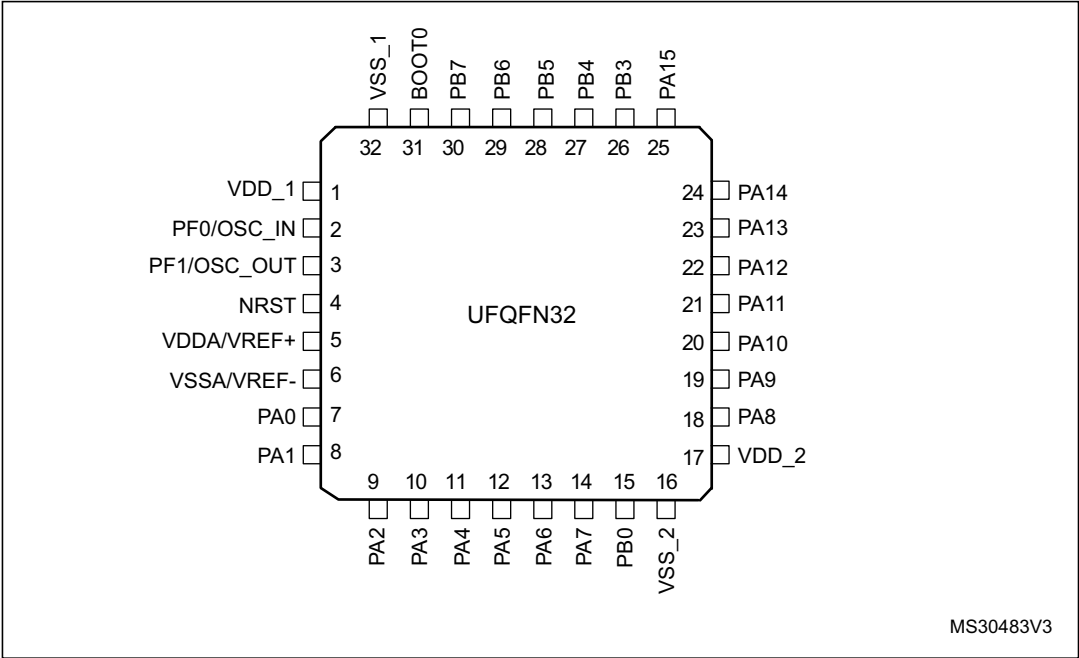
Figure 4. STM32F302x6/x8 UFQFN32 pinout
