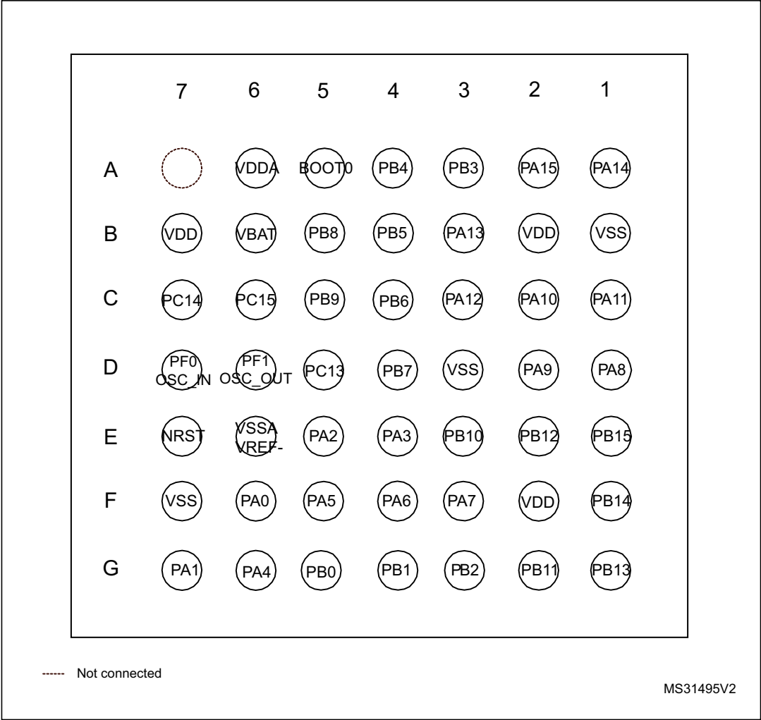
Figure 7. STM32F302x6/x8 WLCSP49 ballout
