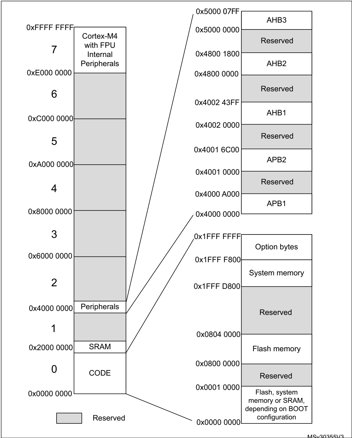
Figure 8. STM32F302x6/x8 memory mapping
