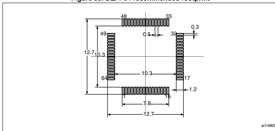
Figure 38. LQFP64 recommended footprint
