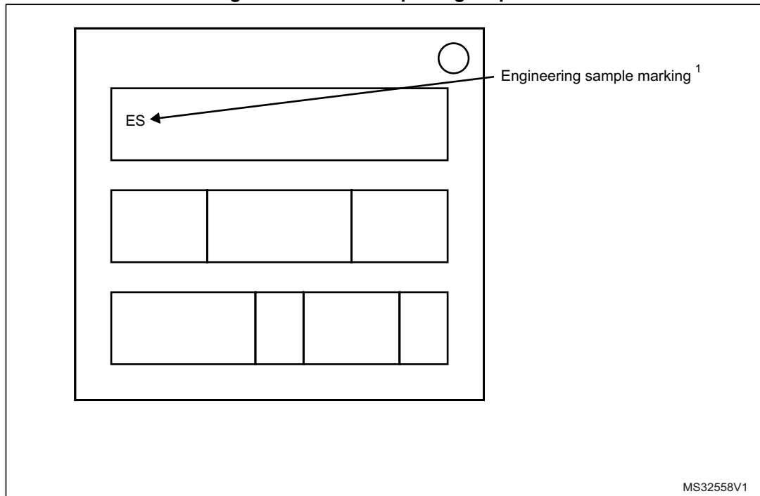
Figure 36. WLCSP49 package top view
