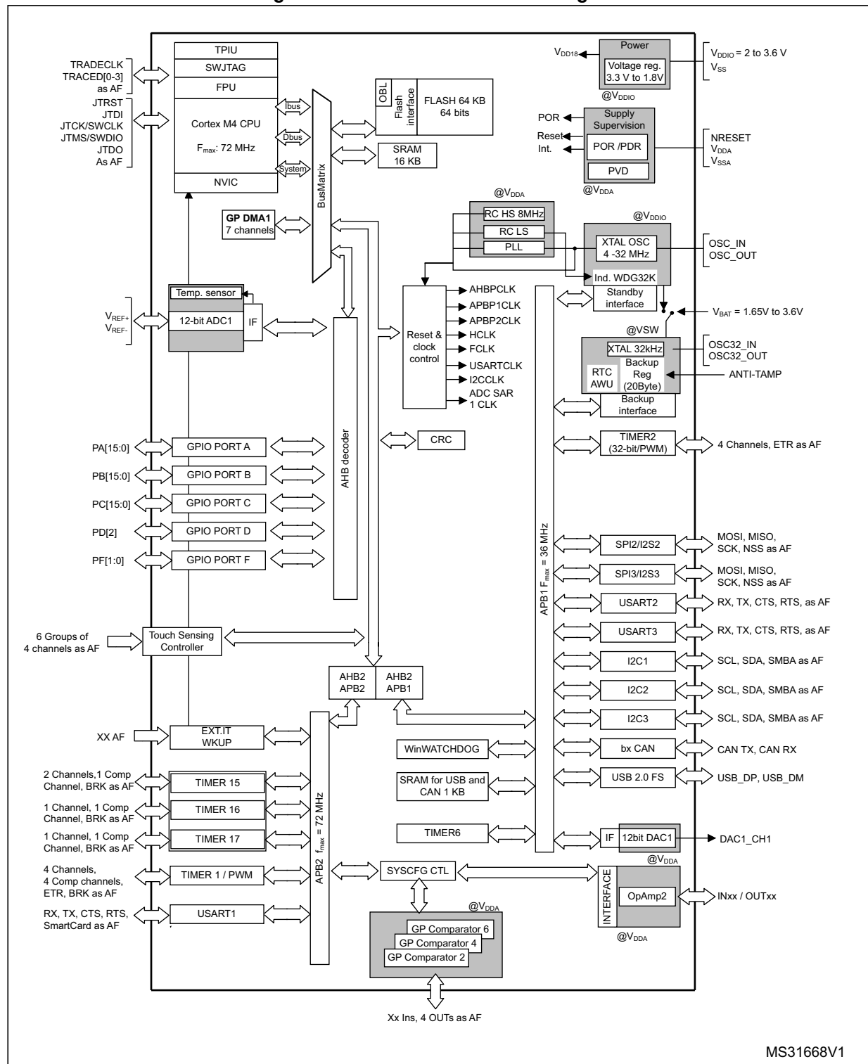
Figure 1. STM32F302x6/x8 block diagram
