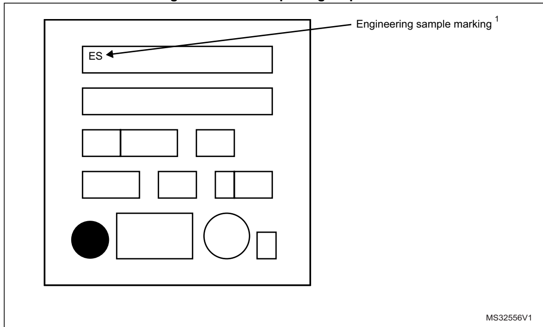
Figure 42. LQFP48 package top view
