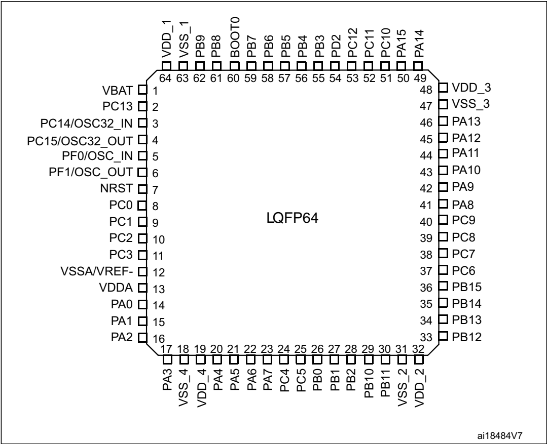
Figure 6. STM32F302x6/x8 LQFP64 pinout
