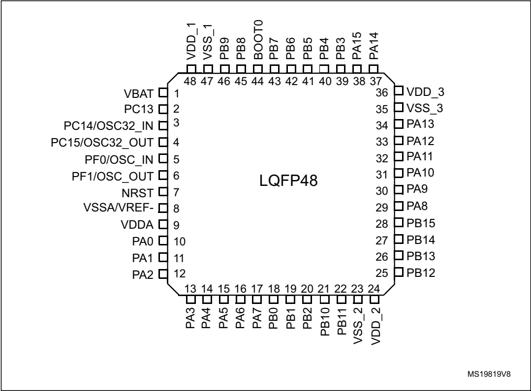
Figure 5. STM32F302x6/x8 LQFP48 pinout
