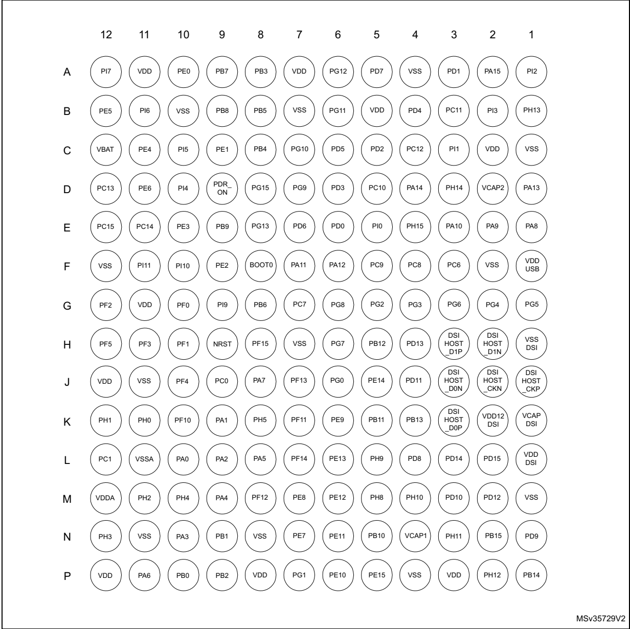
Figure 10. STM32F47x WLCSP168 pinout
