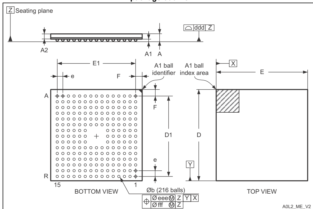
Figure 25. TFBGA216 - thin fine pitch ball grid array 13 × 13 × 0.8mm, package outline
