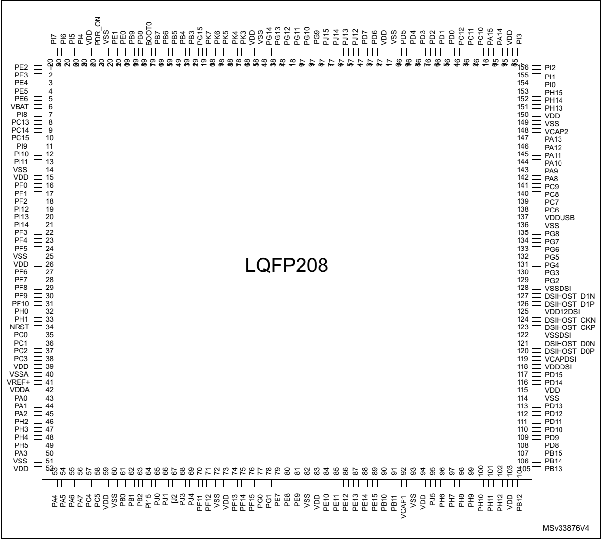
Figure 13. STM32F47x LQFP208 pinout
