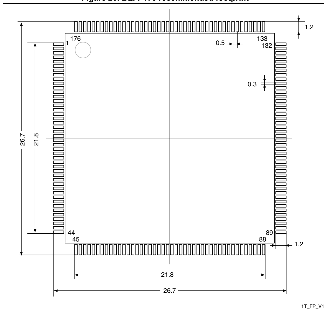
Figure 20. LQFP176 recommended footprint
