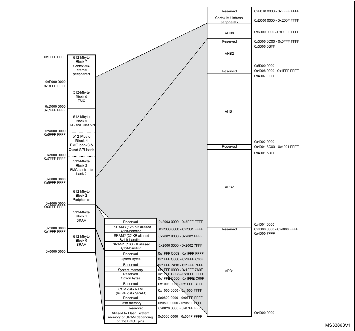
Figure 15. Memory map
