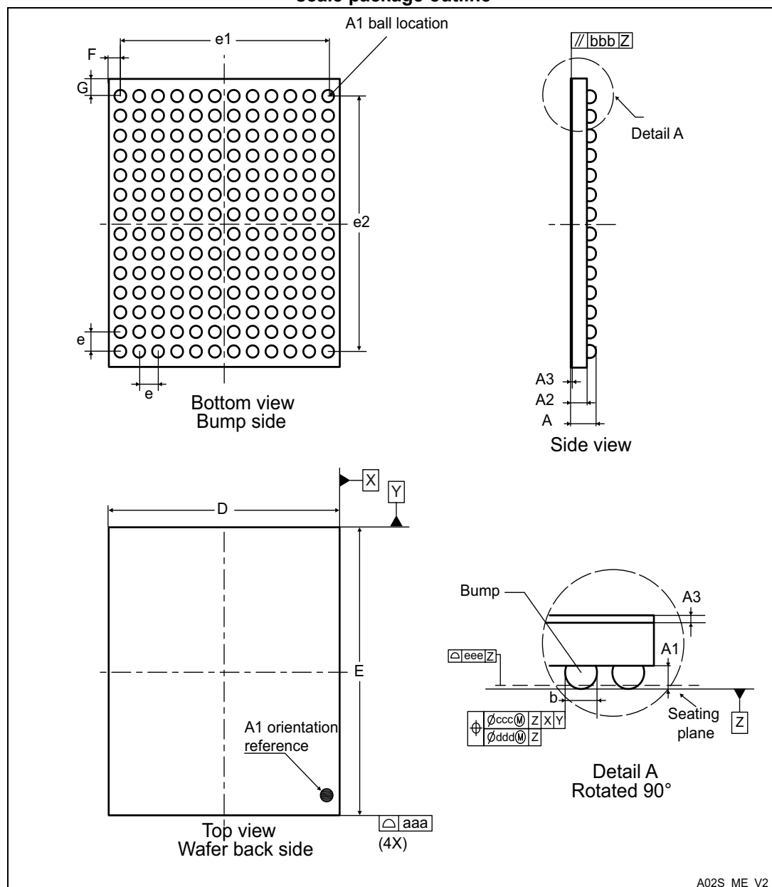
Figure 16. WLCSP168 - 168-pin, 4.891 x 5.692 mm, 0.4 mm pitch wafer level chip scale package outline
