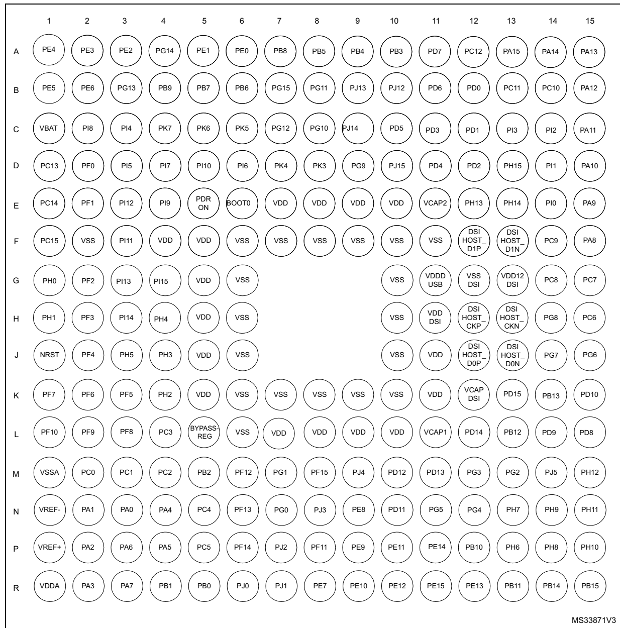
Figure 14. STM32F47x TFBGA216 ballout
