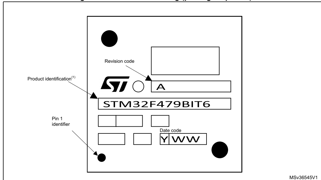
Figure 24. LQFP208 marking (package top view)
