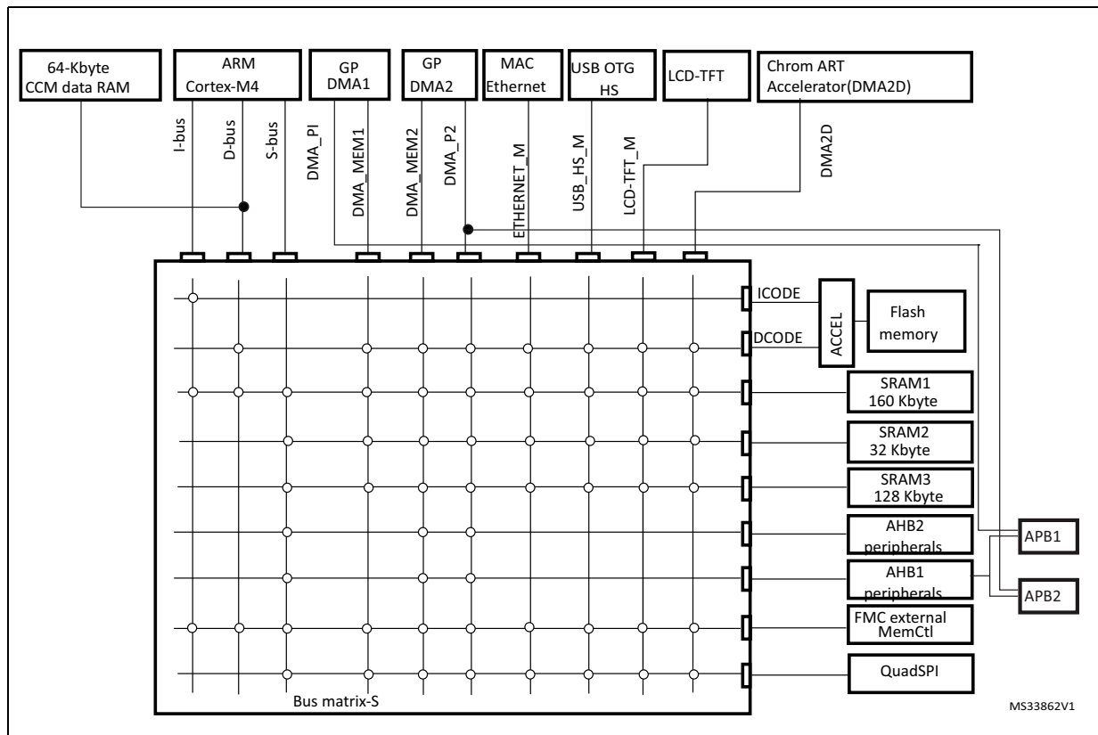
Figure 4. STM32F479xx Multi-AHB matrix
