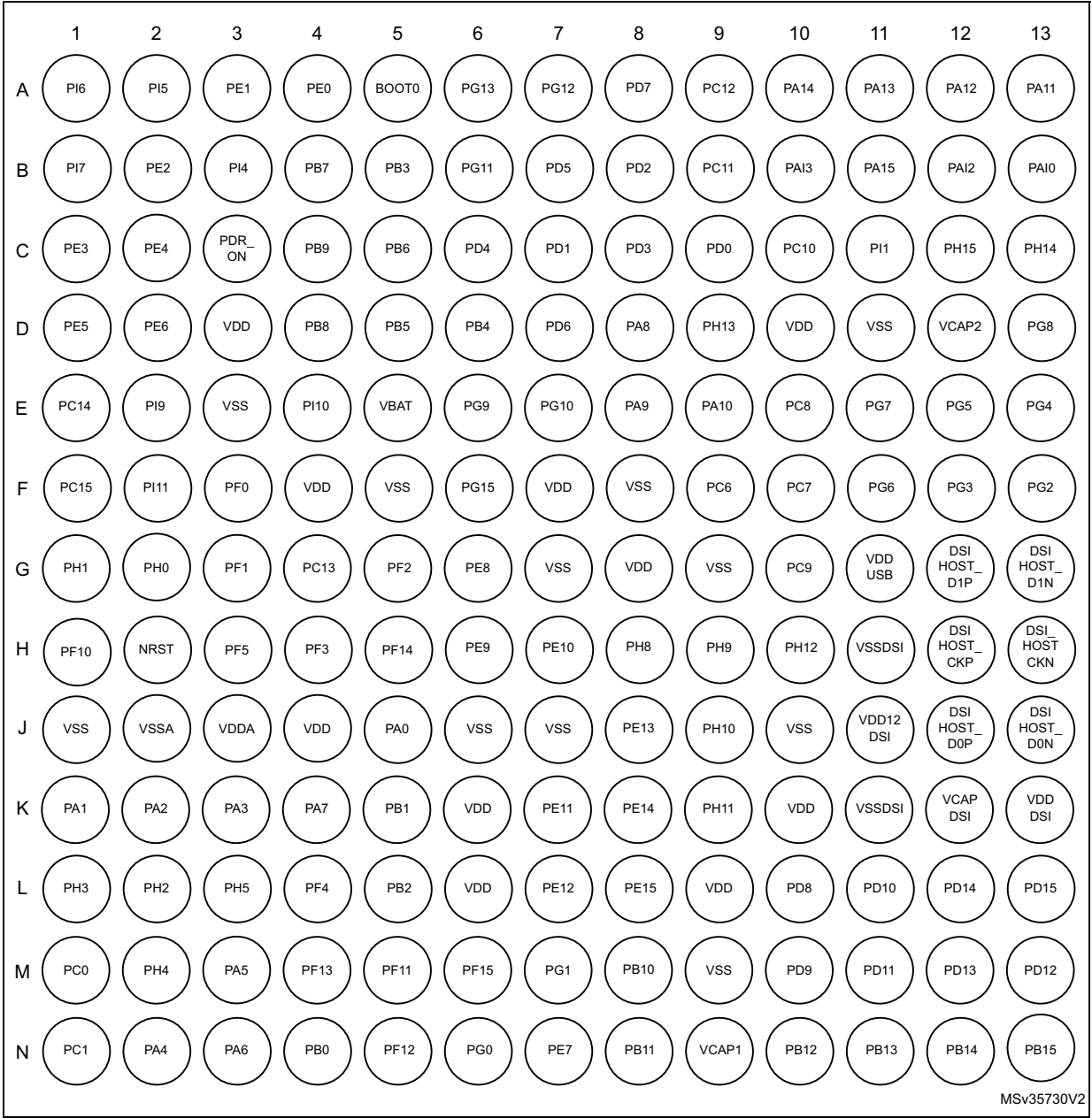
Figure 11. STM32F47x UFBGA169 pinout
