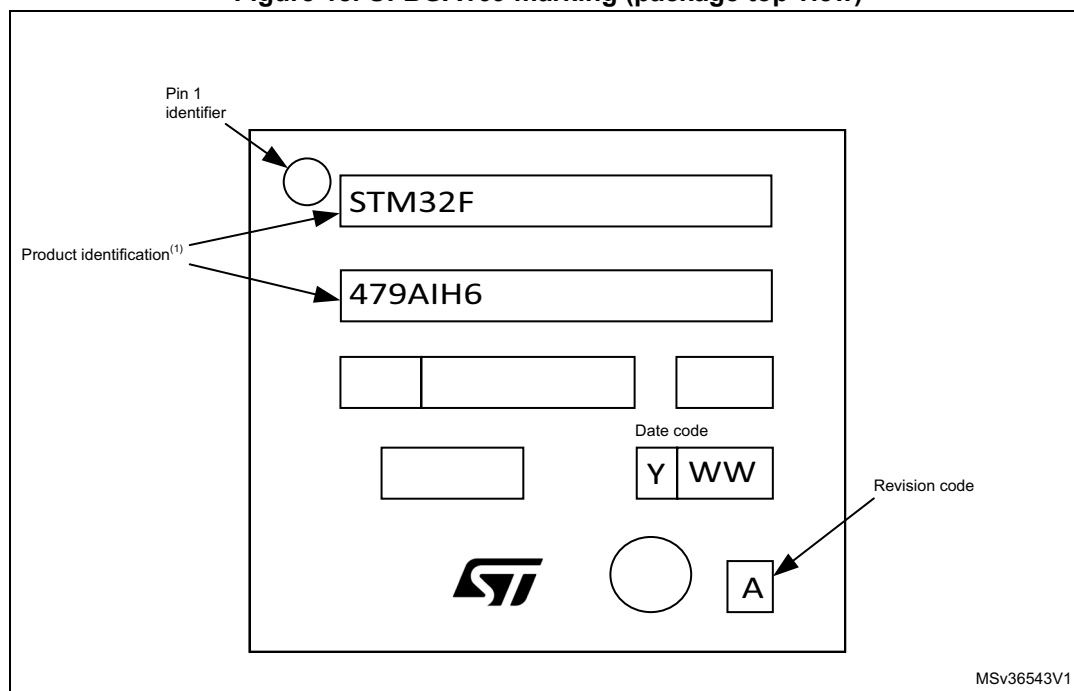
Figure 18. UFBGA169 marking (package top view)
