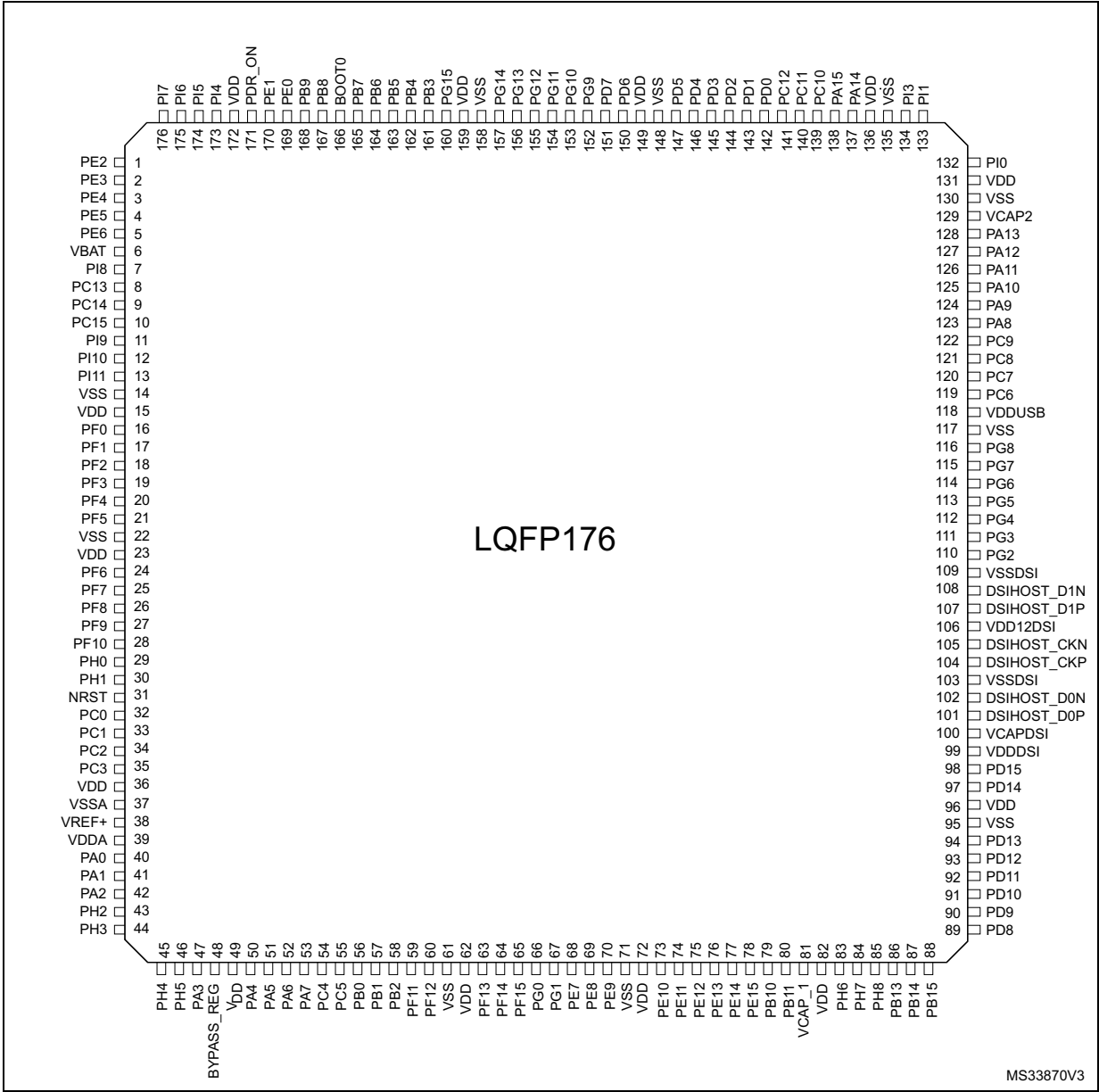
Figure 12. STM32F47x LQFP176 pinout
