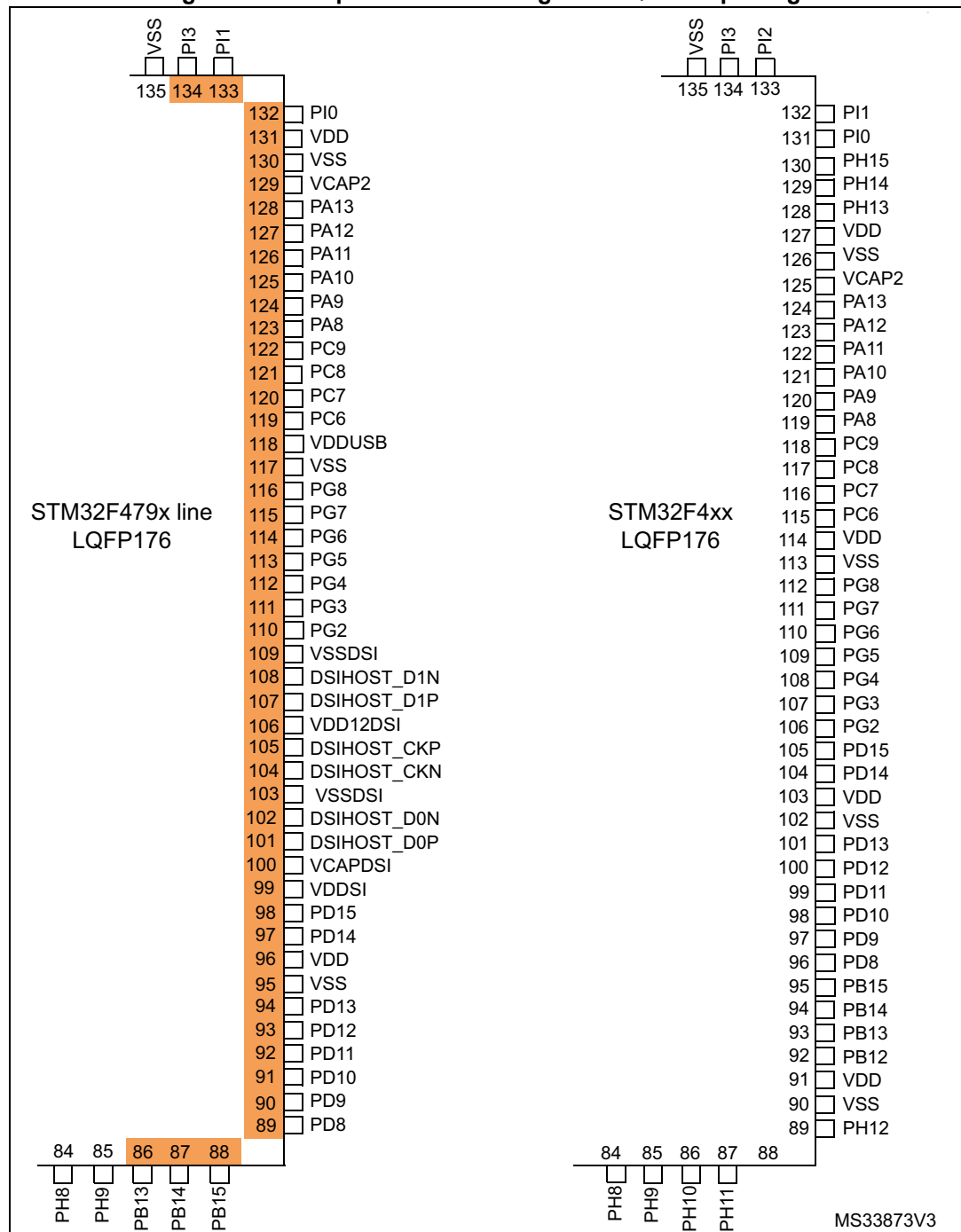
Figure 1. Incompatible board design for LQFP176 package
