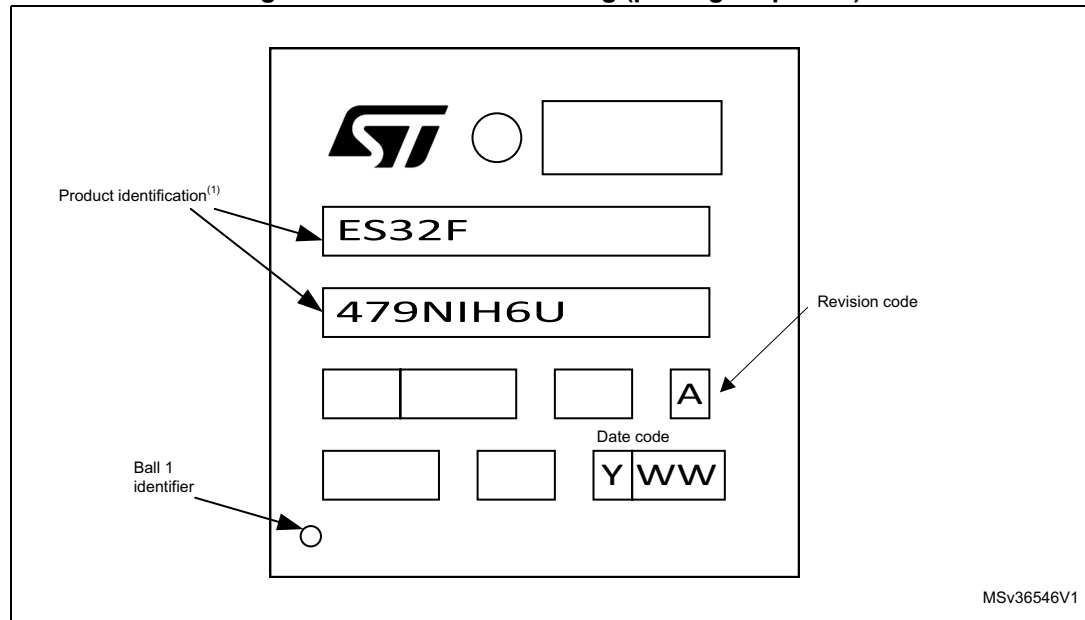
Figure 26. TFBGA216 marking (package top view)
