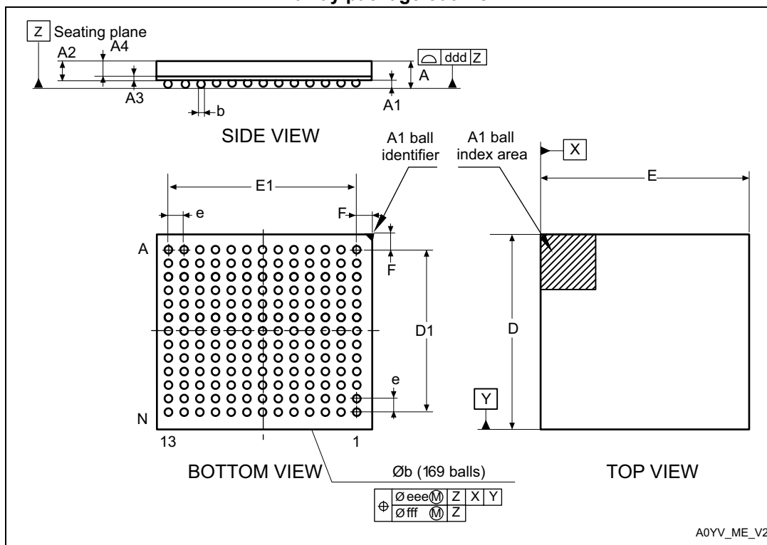
Figure 17. UFBGA169 - 169-pin, 7 x 7 mm, 0.50 mm pitch, ultra fine pitch ball grid array package outline
