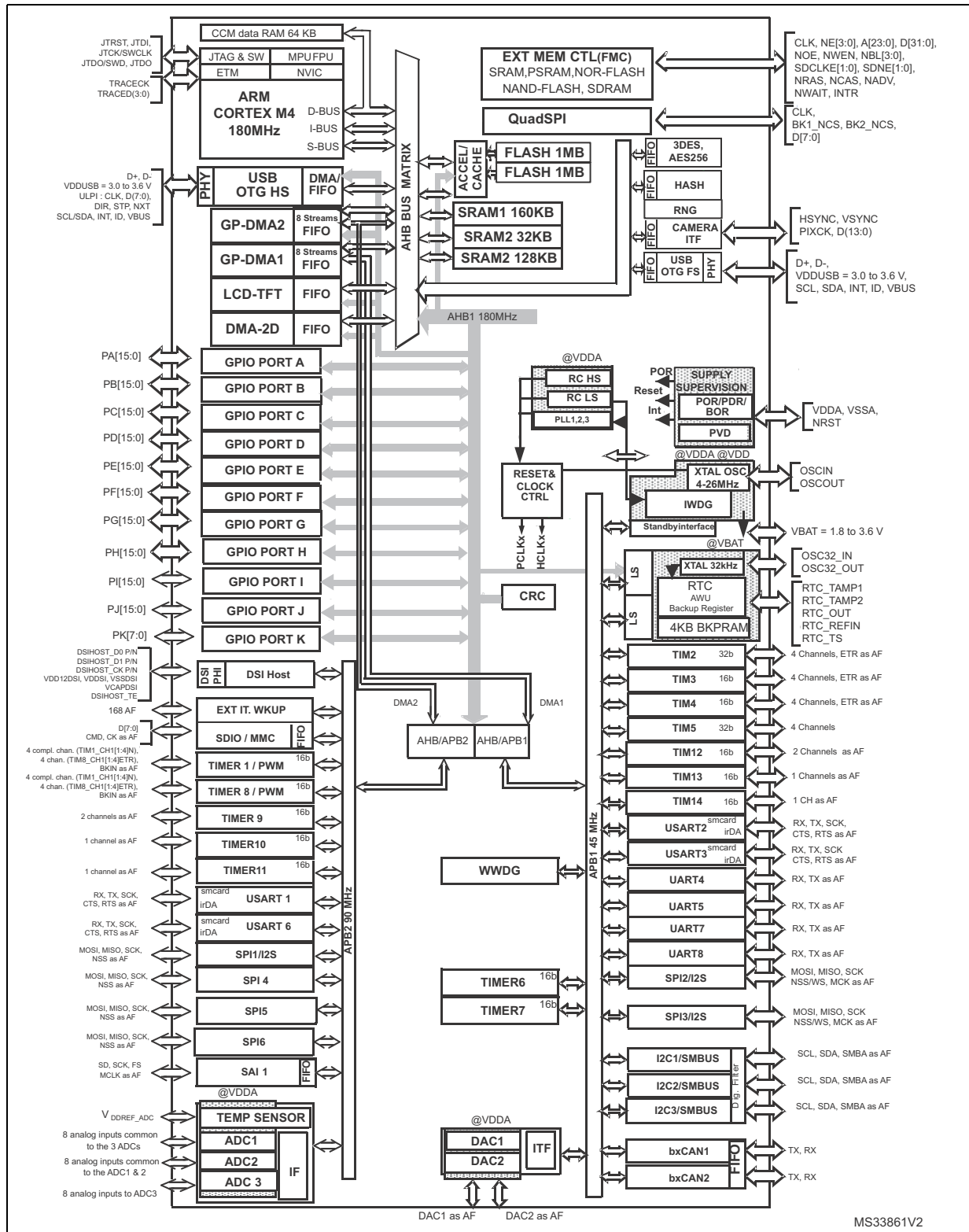
Figure 3. STM32F479xx block diagram
