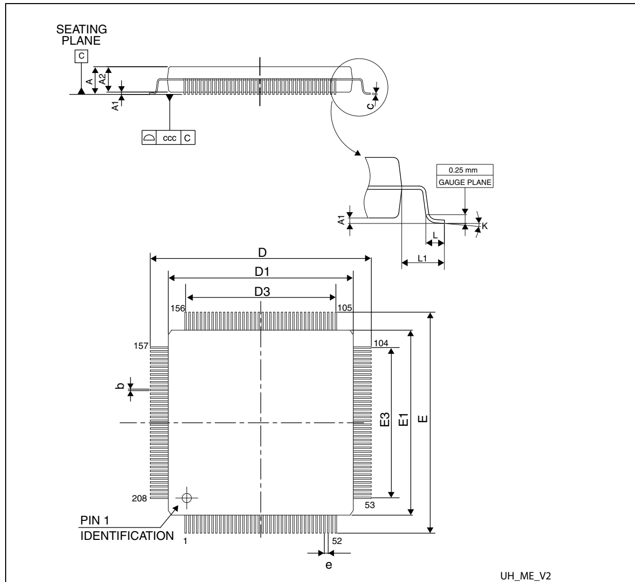
Figure 22. LQFP208, 28 x 28 mm, 208-pin low-profile quad flat package outline
