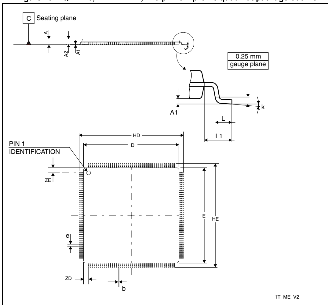
Figure 19. LQFP176, 24 x 24 mm, 176-pin low-profile quad flat package outline
