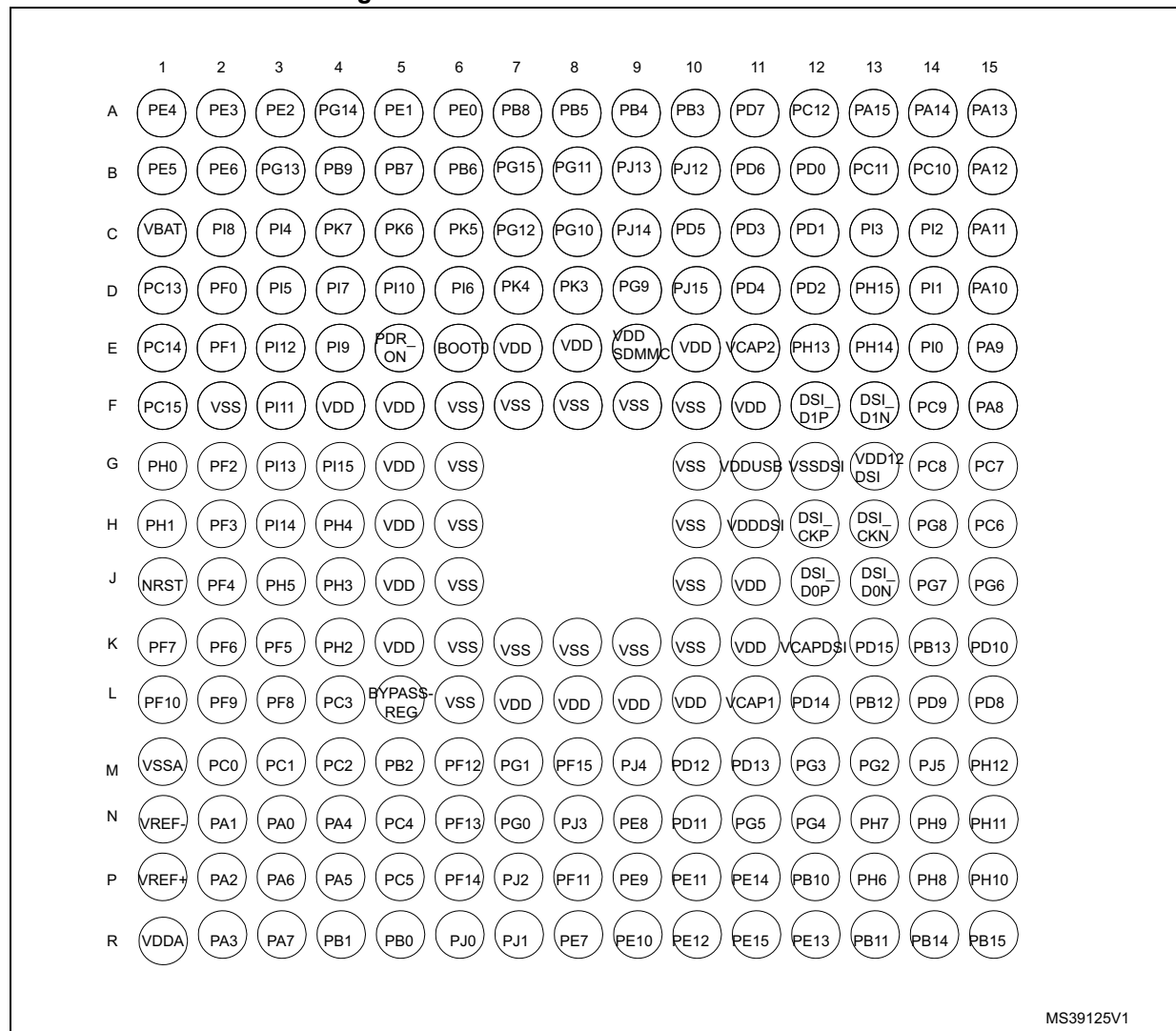
Figure 17. STM32F769xx TFBGA216 ballout
