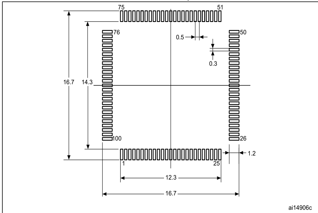
Figure 20. LQFP100, 14 x 14 mm, 100-pin low-profile quad flat package recommended footprint
