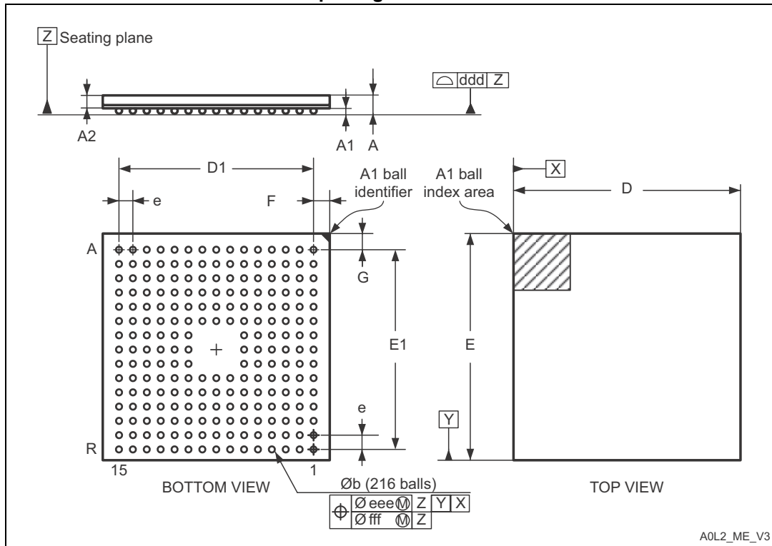
Figure 31. TFBGA216, 13 × 13 × 0.8 mm thin fine-pitch ball grid array package outline
