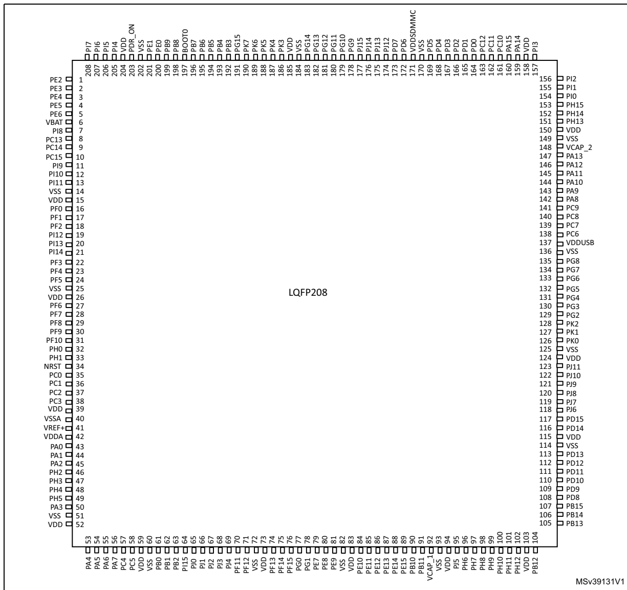
Figure 13. STM32F767xx LQFP208 pinout
