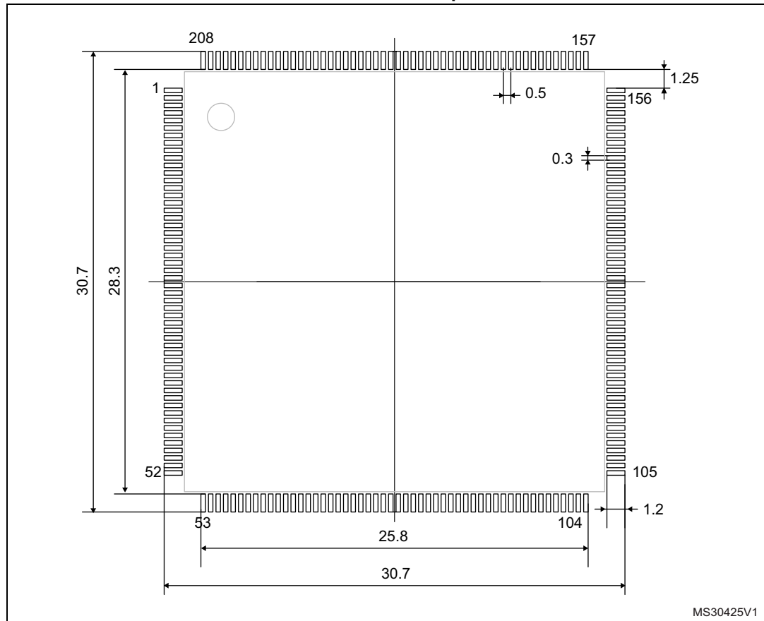
Figure 28. LQFP208, 28 x 28 mm, 208-pin low-profile quad flat package recommended footprint
