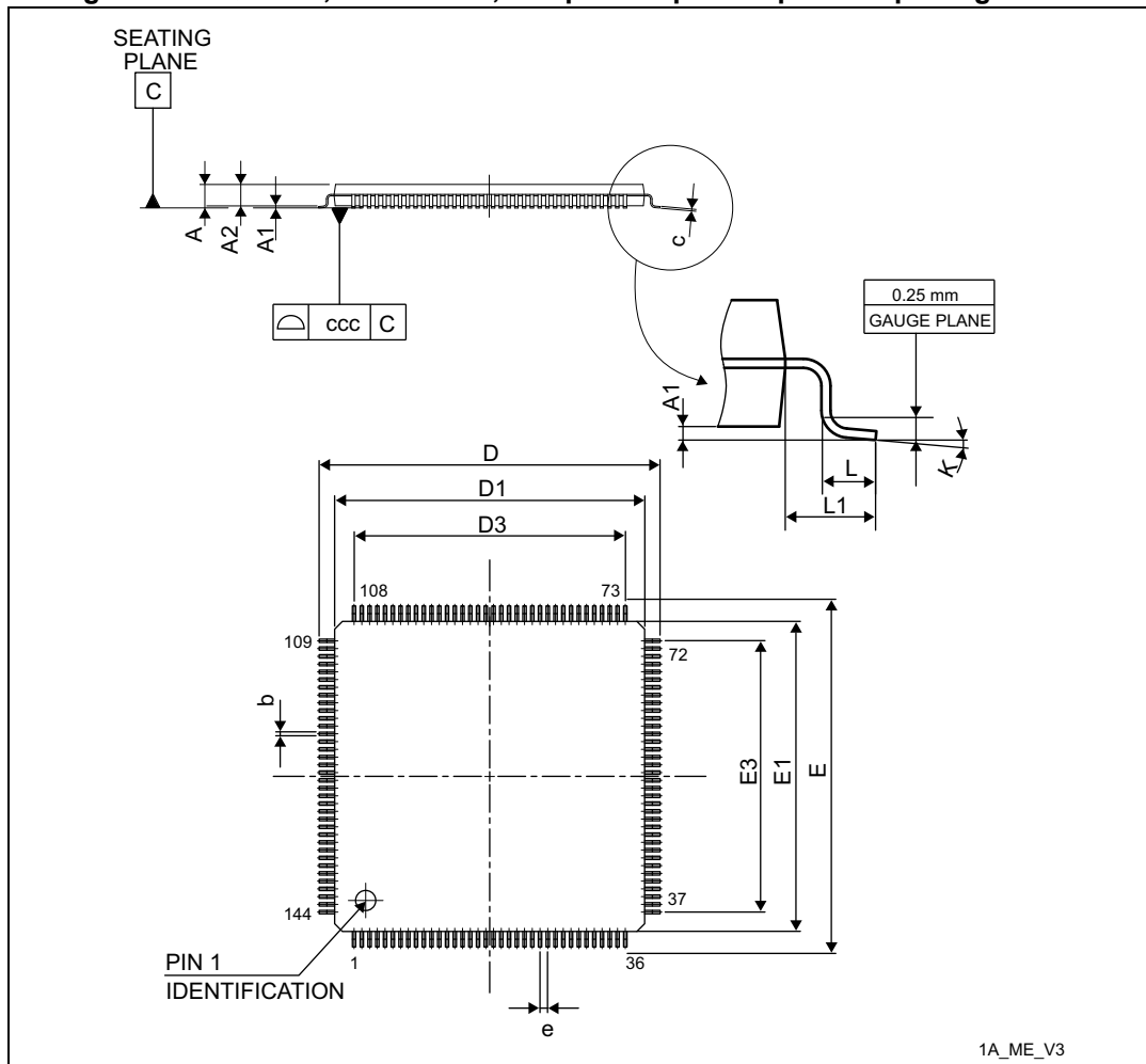
Figure 21. LQFP144, 20 x 20 mm, 144-pin low-profile quad flat package outline
