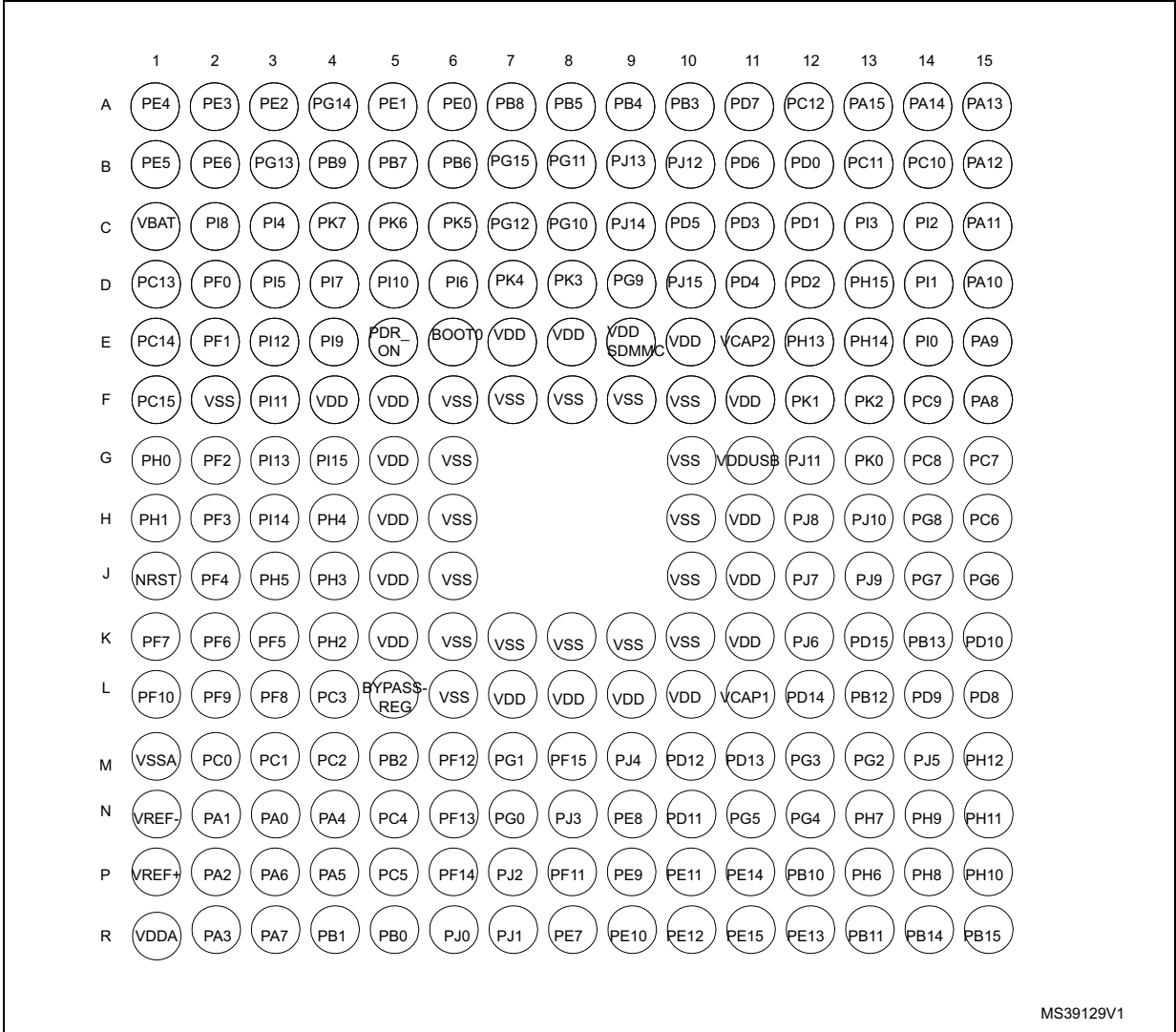
Figure 16. STM32F767xx TFBGA216 ballout
