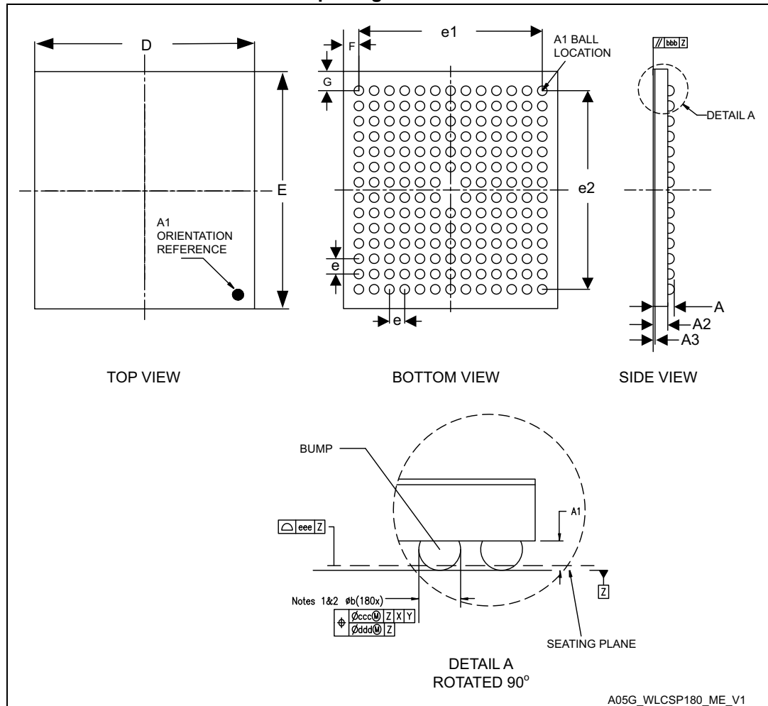
Figure 25. WLCSP 180-bump, 5.5 x 6 mm, 0.4 mm pitch wafer level chip scale package outline
