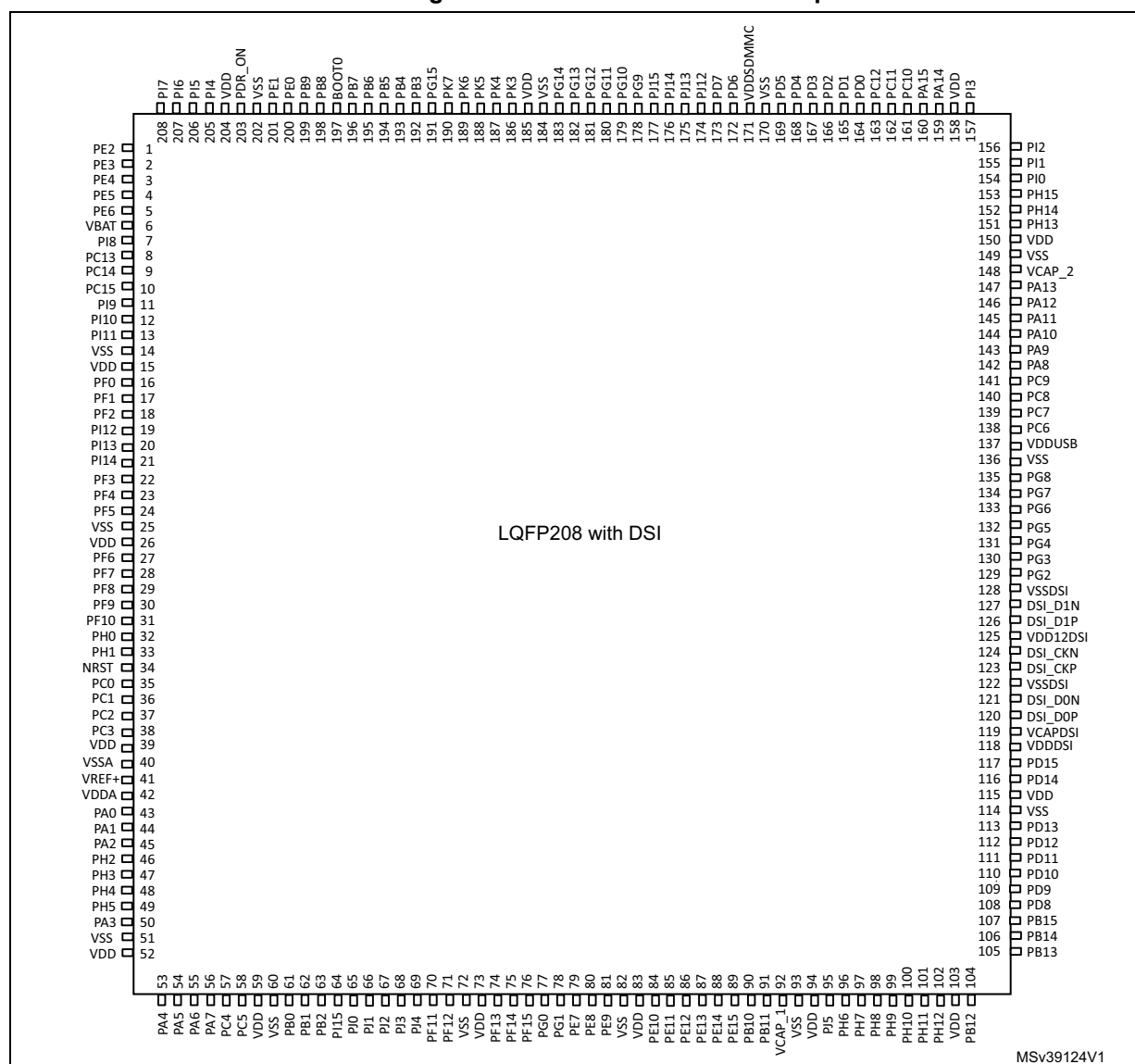
Figure 14. STM32F769xx LQFP208 pinout
