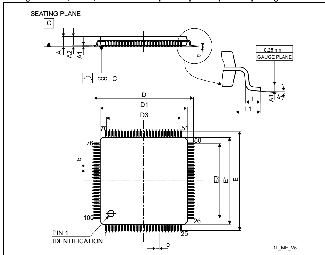
Figure 19. LQFP100, 14 x 14 mm 100-pin low-profile quad flat package outline
