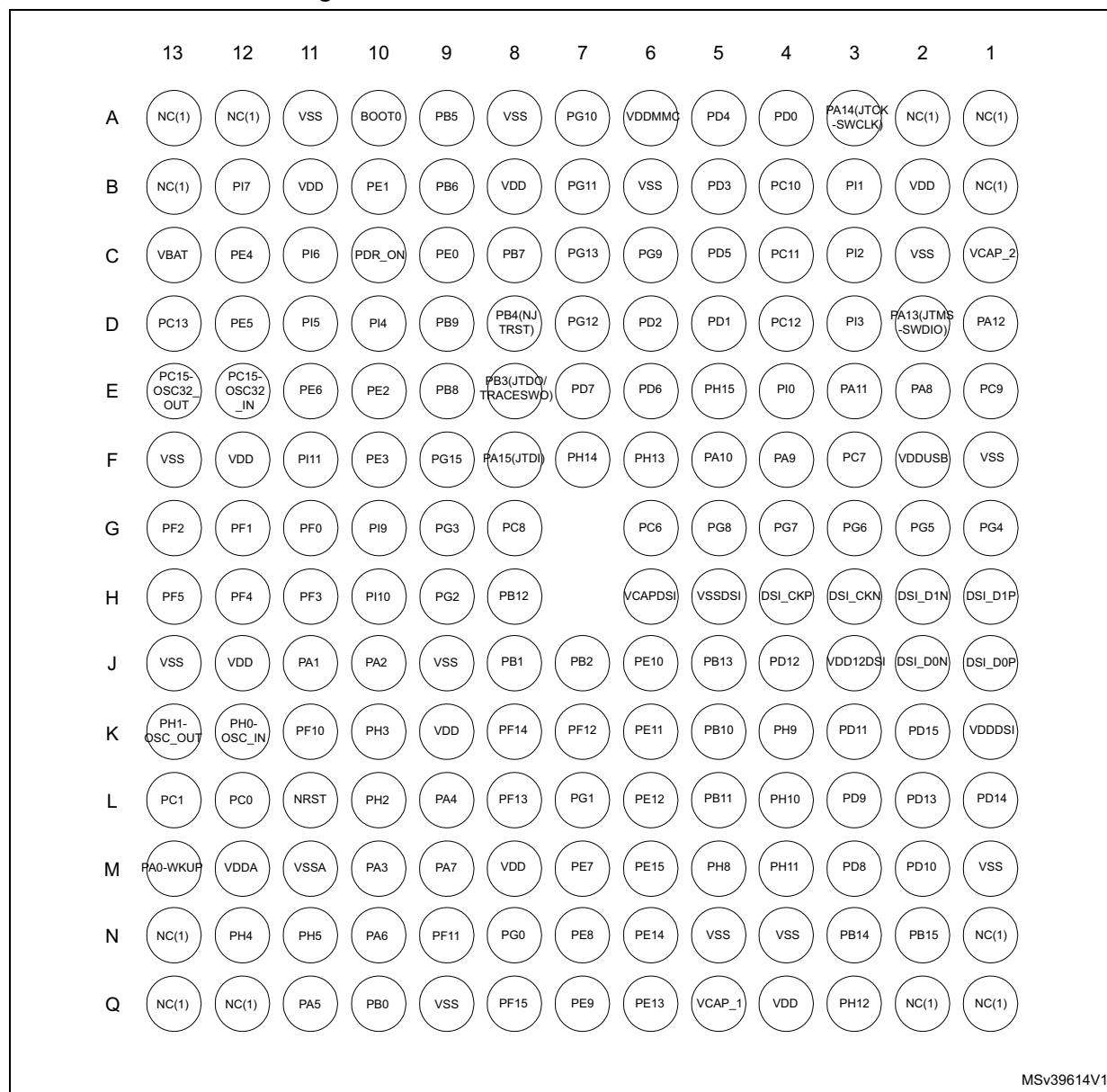
Figure 12. STM32F769xx/STM32F768Ax WLCSP180 ballout
