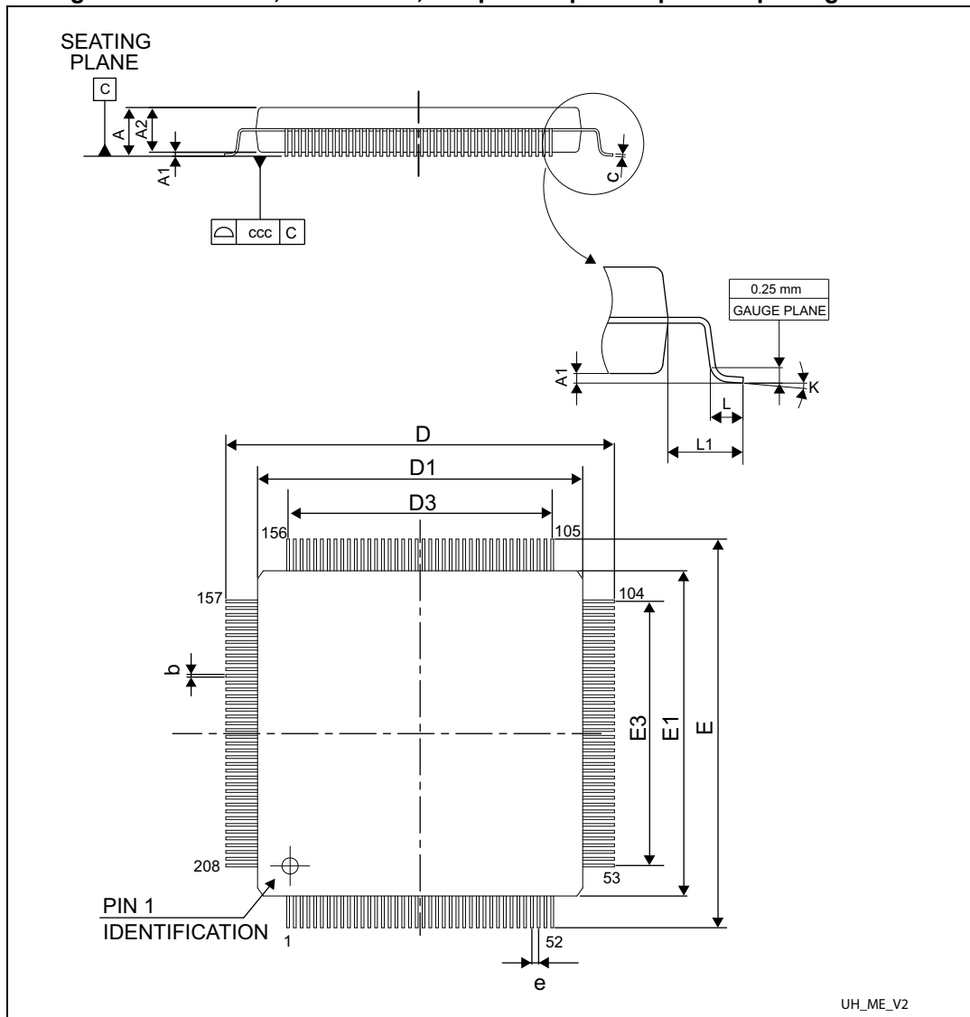
Figure 27. LQFP208, 28 x 28 mm, 208-pin low-profile quad flat package outline
