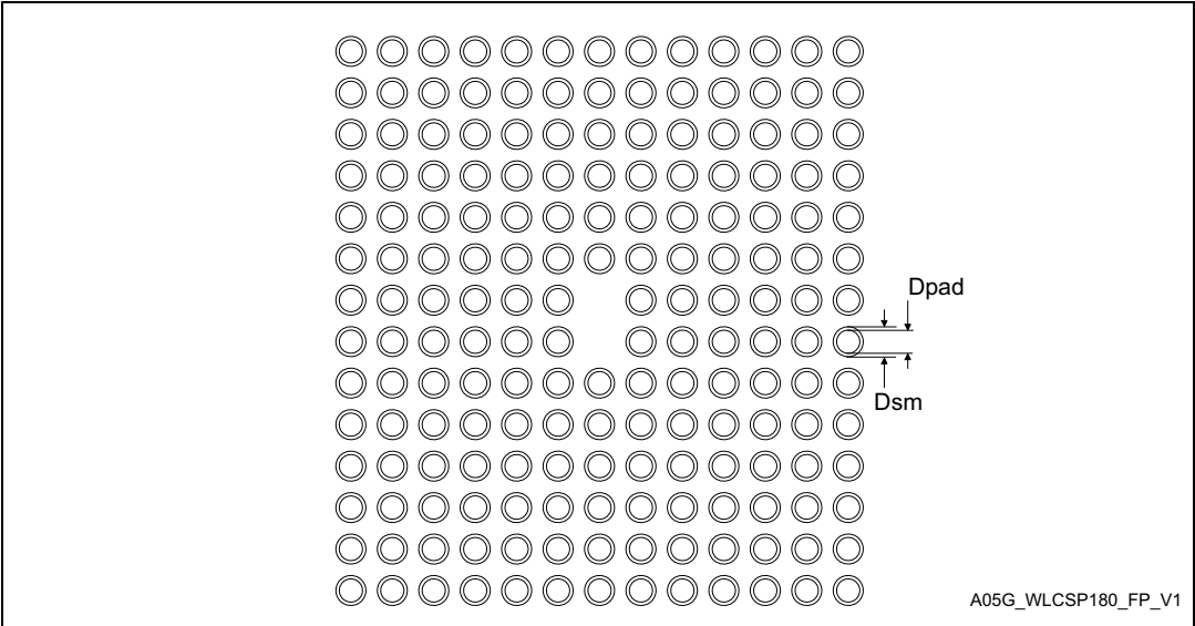
Figure 26. WLCSP 180-bump, 5.5 x 6 mm, 0.4 mm pitch wafer level chip scale package recommended footprint
