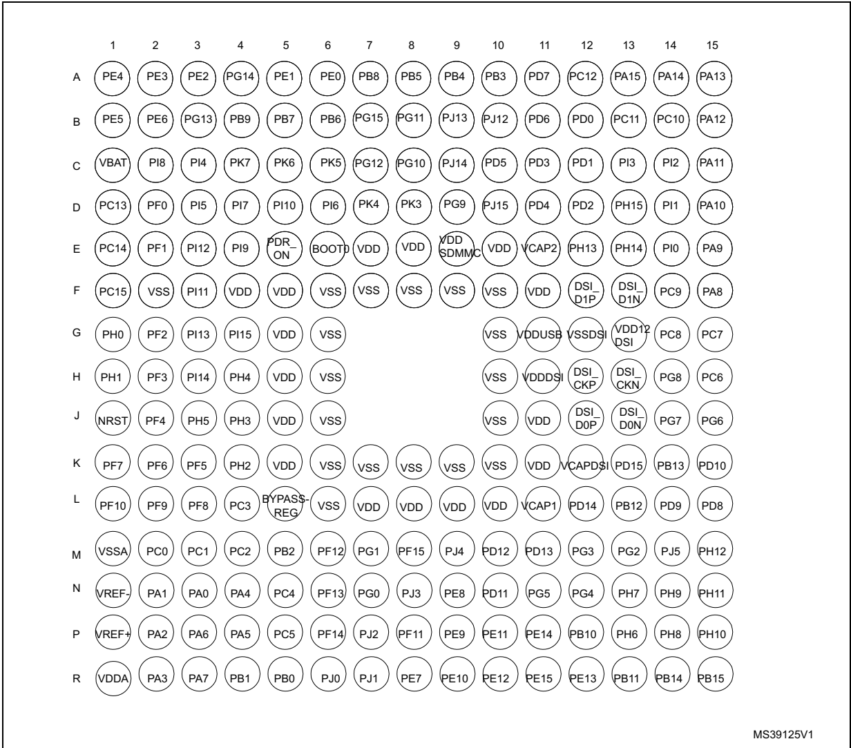
Figure 17. STM32F779xx TFBGA216 ballout
