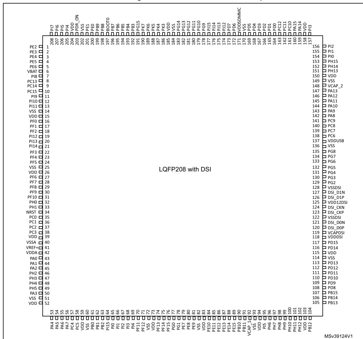
Figure 14. STM32F779xx LQFP208 pinout
