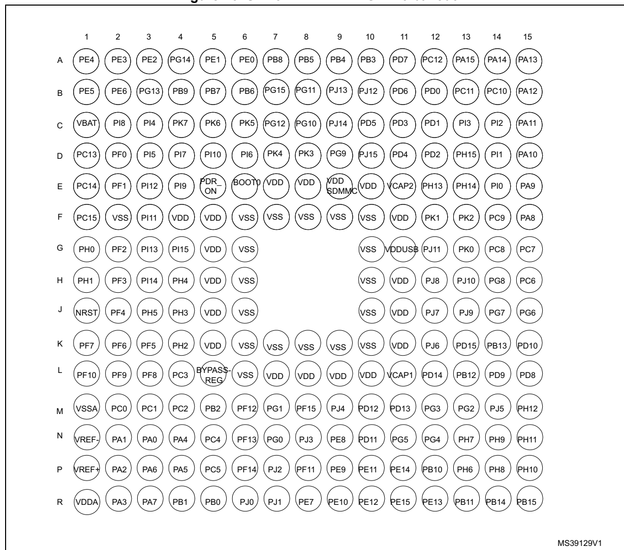
Figure 16. STM32F77xxx TFBGA216 ballout
