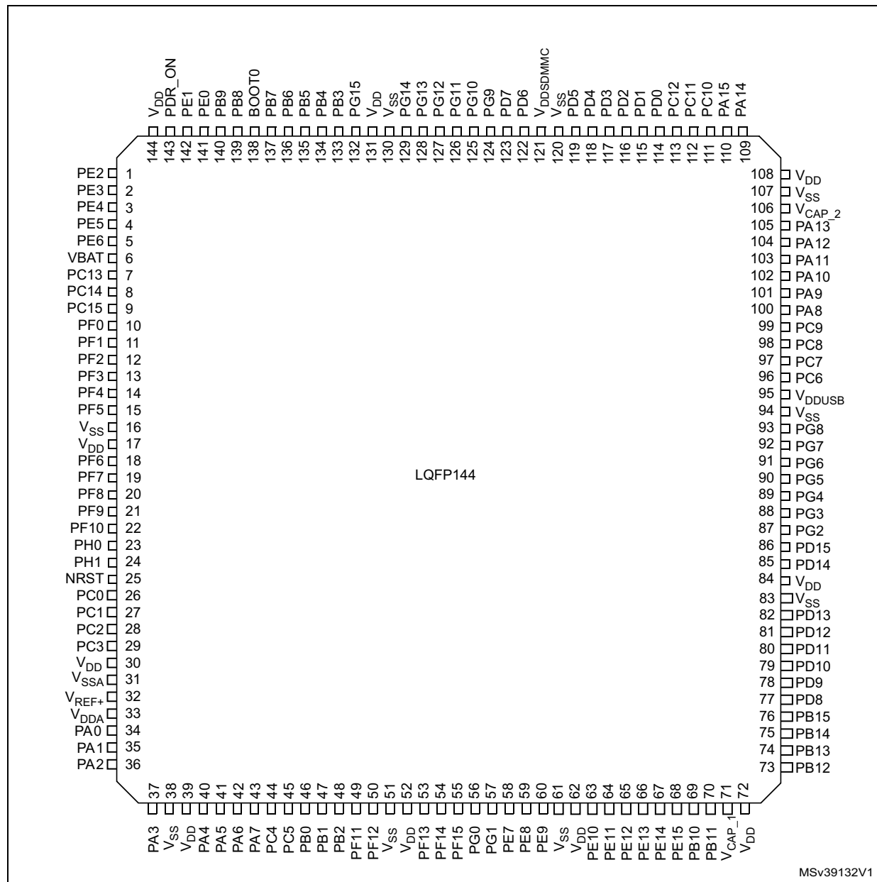
Figure 10. STM32F77xxx LQFP144 pinout
