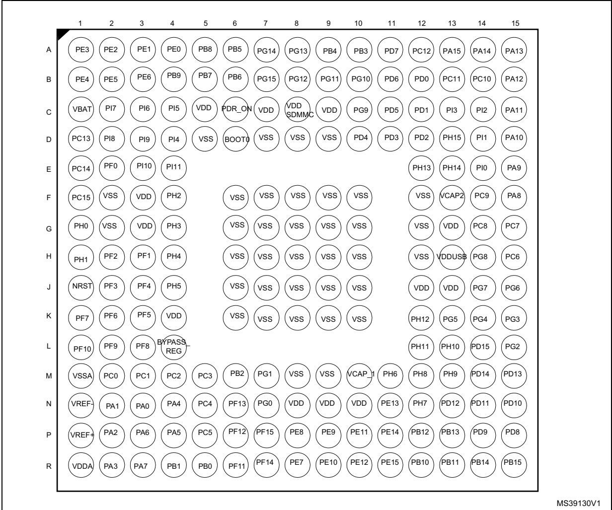
Figure 15. STM32F77xxx UFBGA176 ballout
