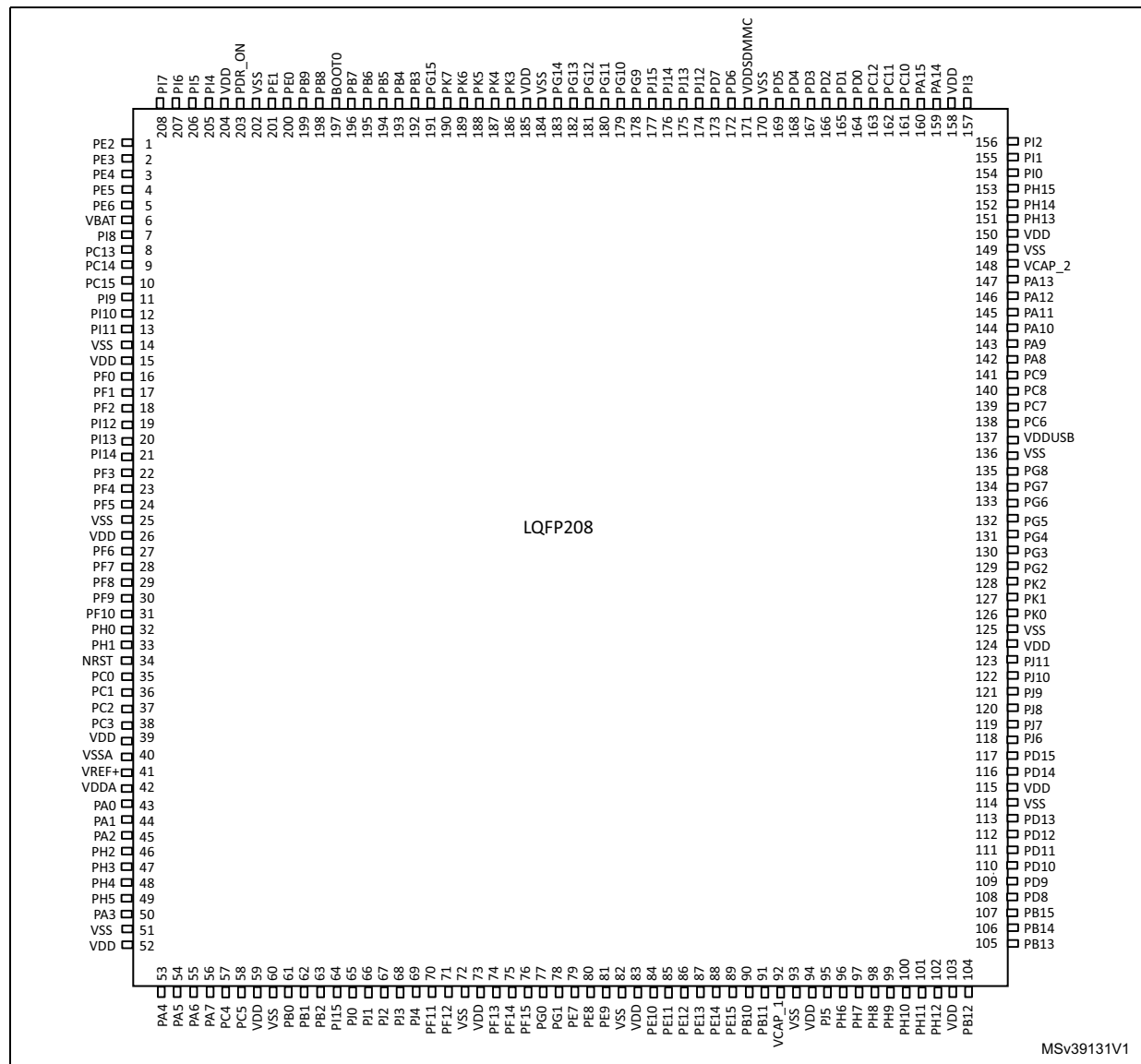
Figure 13. STM32F77xxx LQFP208 pinout
