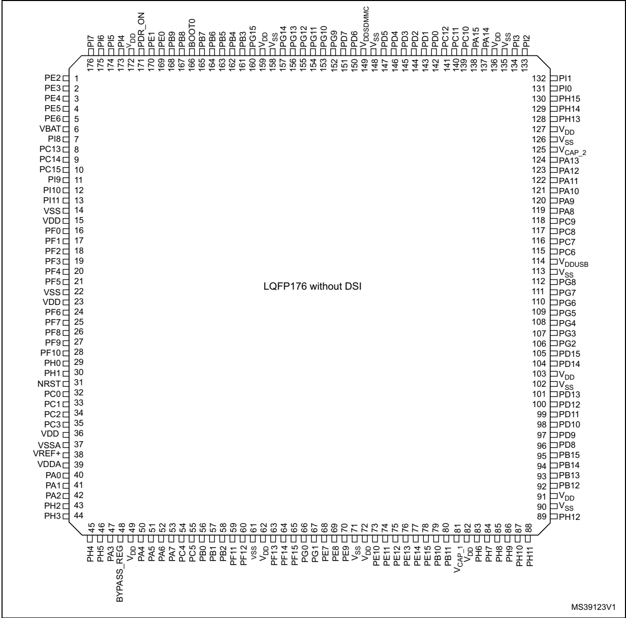
Figure 11. STM32F77xxx LQFP176 pinout
