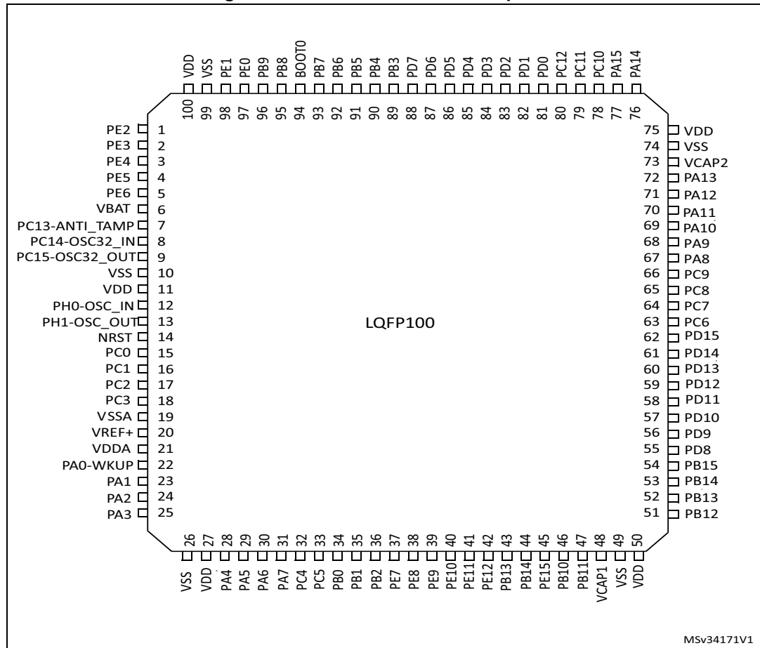
Figure 9. STM32F77xxx LQFP100 pinout
