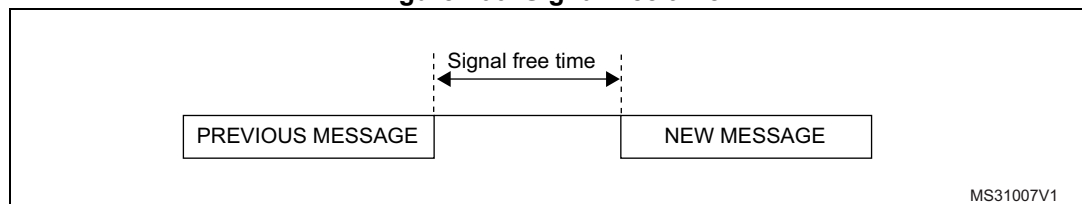
Figure 406. Signal free time
