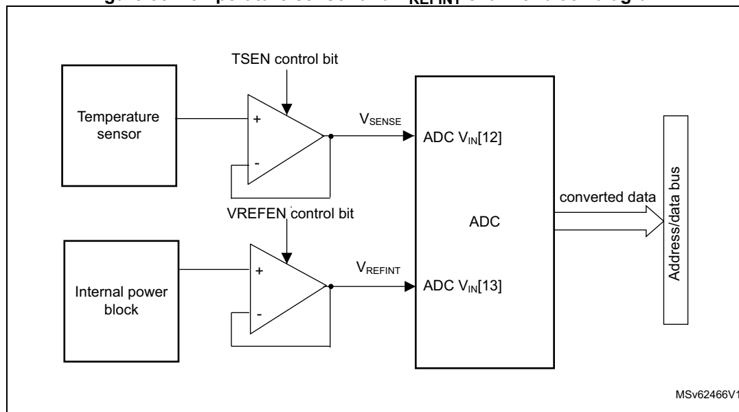
Figure 55. Temperature sensor and V REFINT channel block diagram
