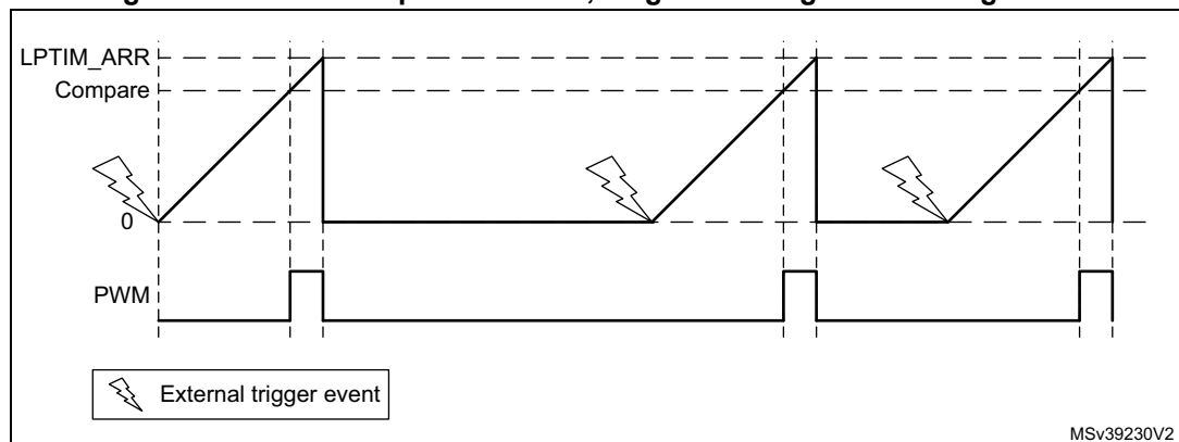
Figure 271. LPTIM output waveform, single counting mode configuration
