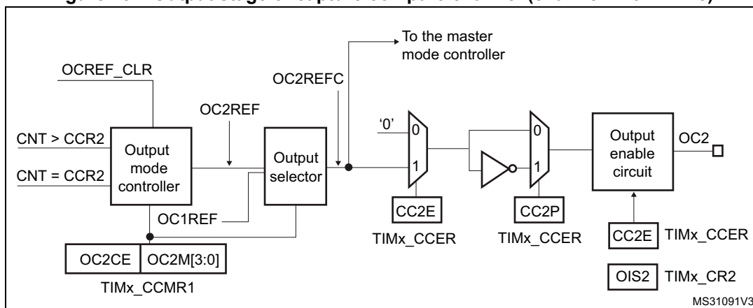
Figure 252. Output stage of capture/compare channel (channel 2 for TIM15)
