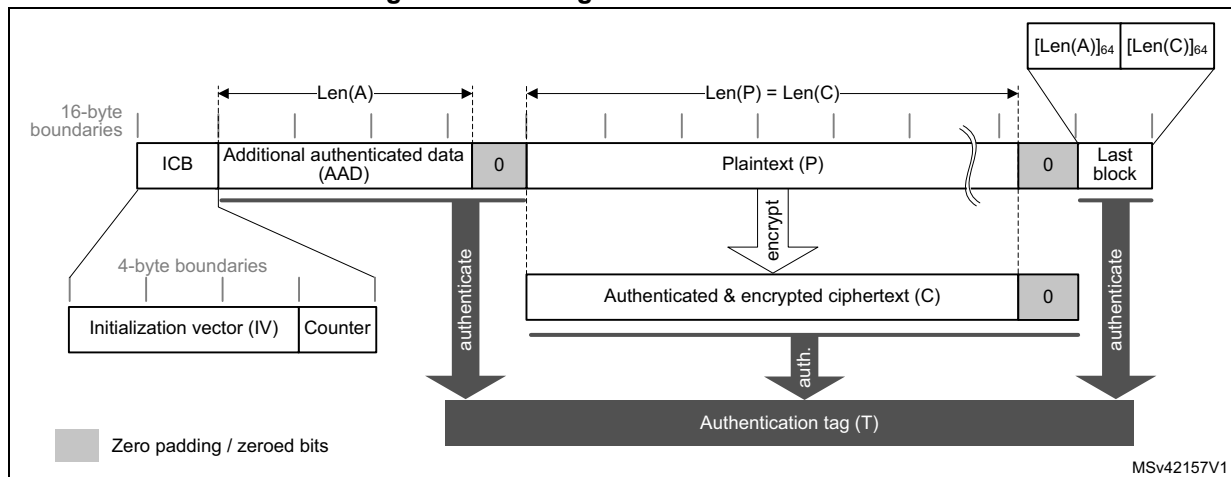
Figure 91. Message construction in GCM
