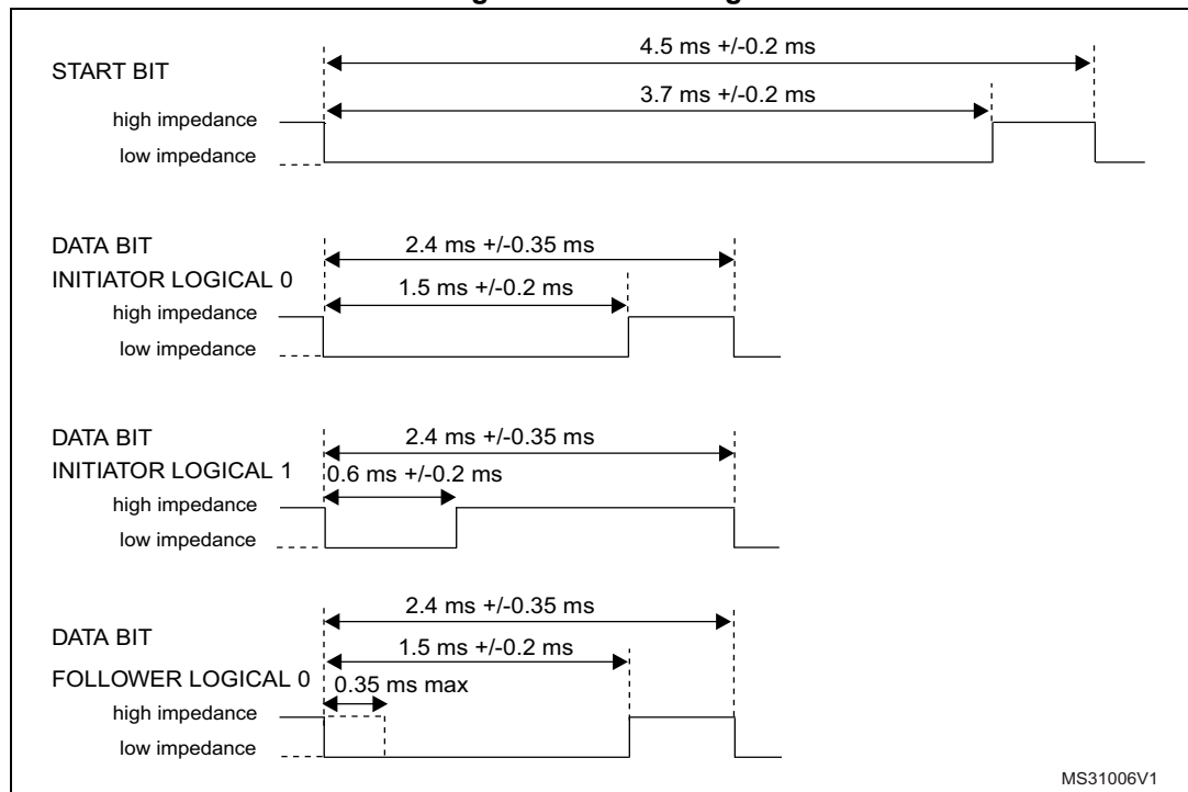
Figure 405. Bit timings
