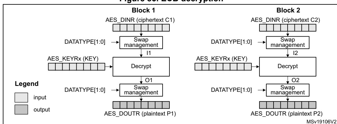
Figure 83. ECB decryption
