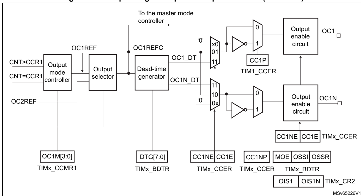
Figure 251. Output stage of capture/compare channel (channel 1)
