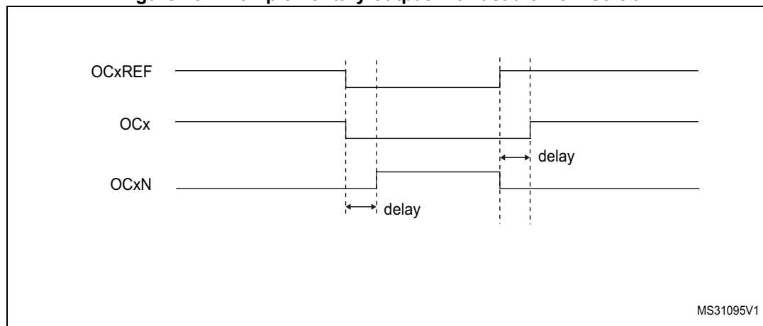
Figure 257. Complementary output with dead-time insertion.
