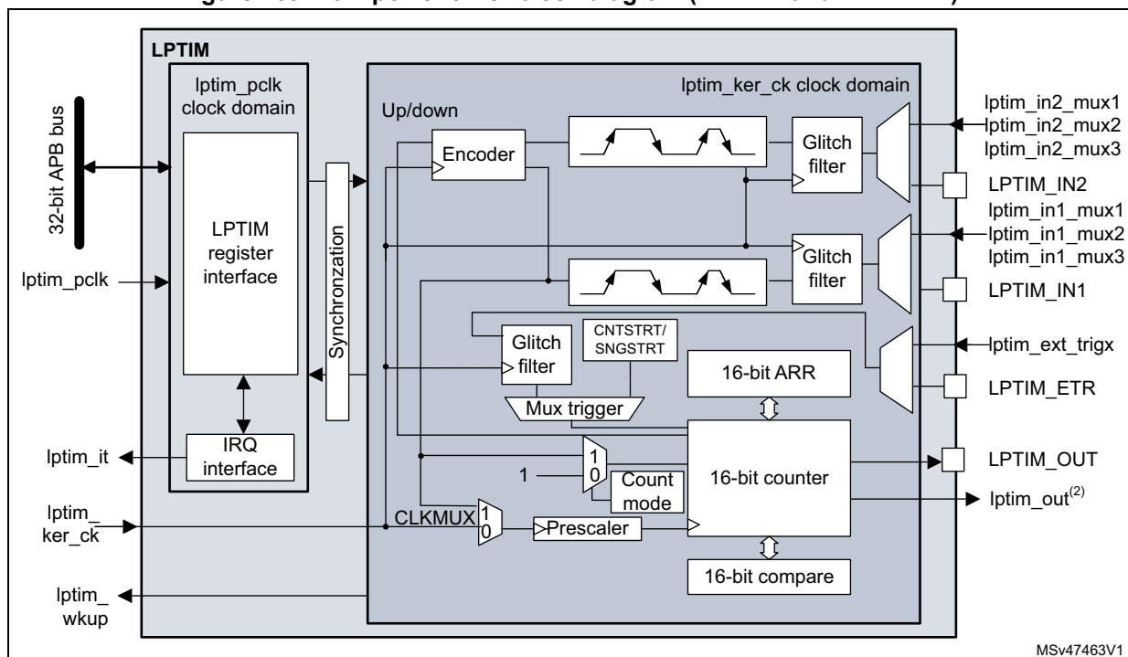
Figure 269. Low-power timer block diagram (LPTIM1 and LPTIM2 (1) )
