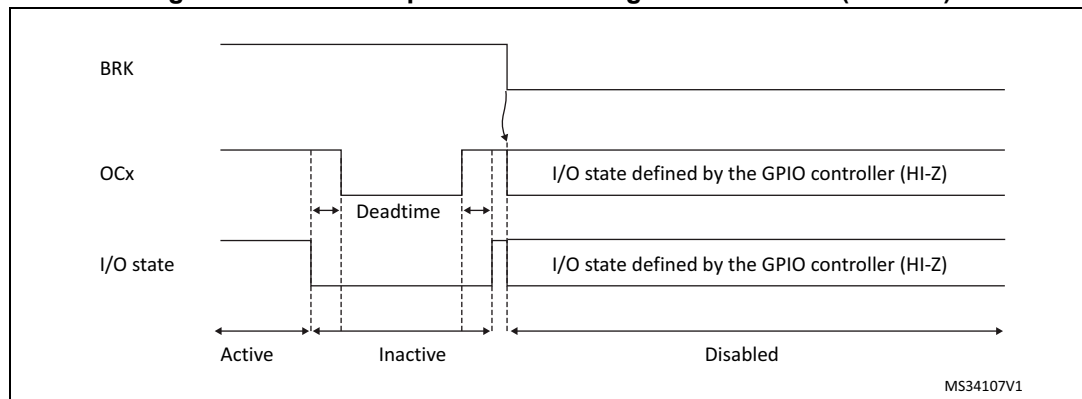
Figure 146. PWM output state following BRK assertion (OSSR=0)
