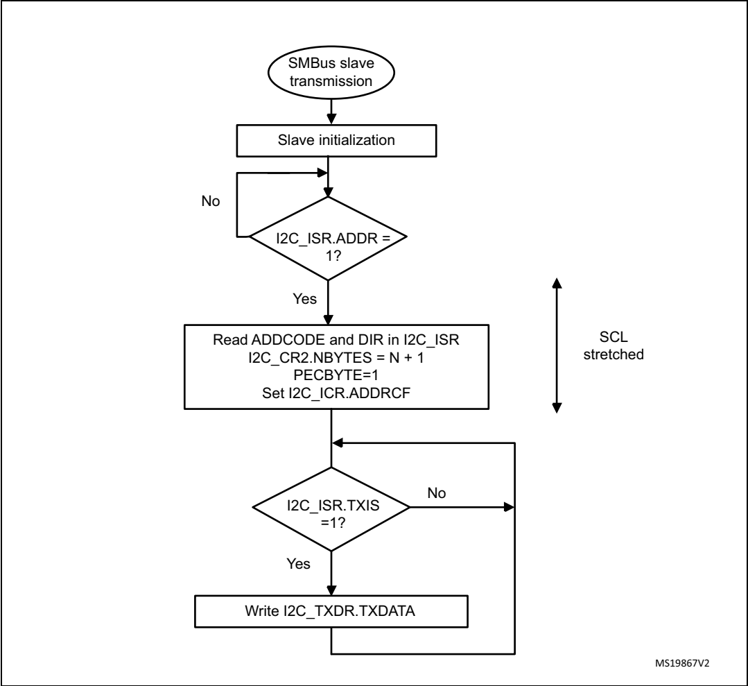
Figure 307. Transfer sequence flowchart for SMBus slave transmitter N bytes + PEC
