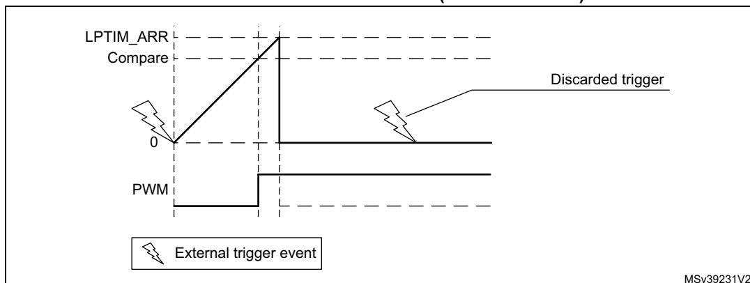
Figure 272. LPTIM output waveform, Single counting mode configuration and Set-once mode activated (WAVE bit is set)
