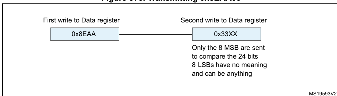
Figure 373. Transmitting 0x8EAA33
