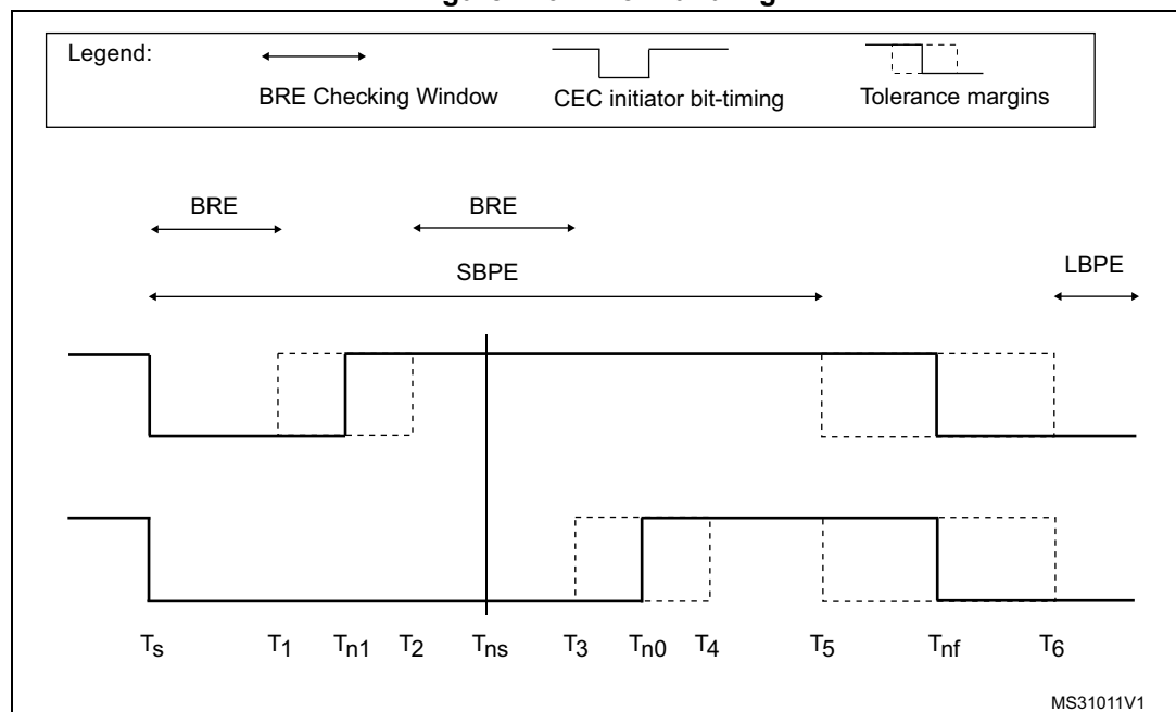
Figure 410. Error handling
