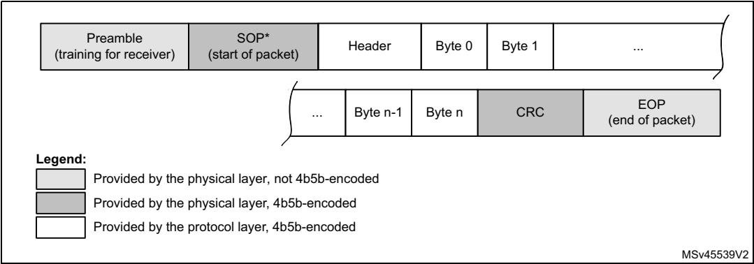
Figure 395. Packet format
