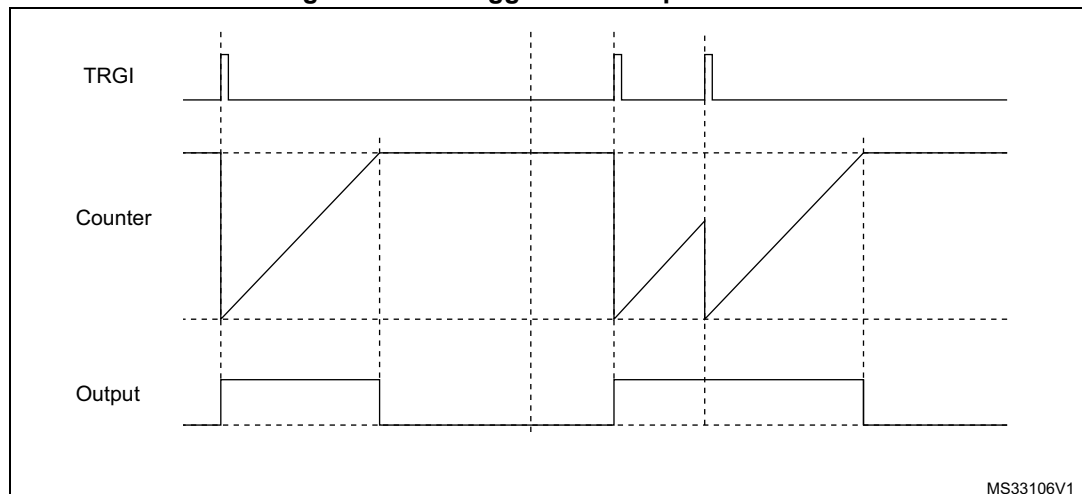
Figure 196. Retriggerable one-pulse mode.
