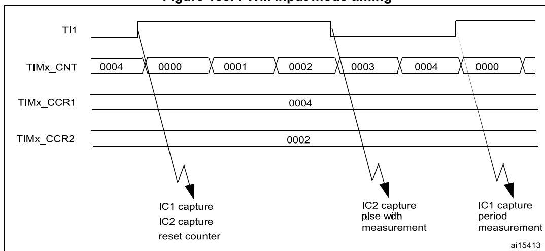
Figure 188. PWM input mode timing
