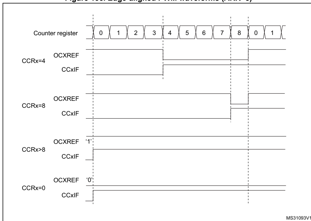
Figure 135. Edge-aligned PWM waveforms (ARR=8)
