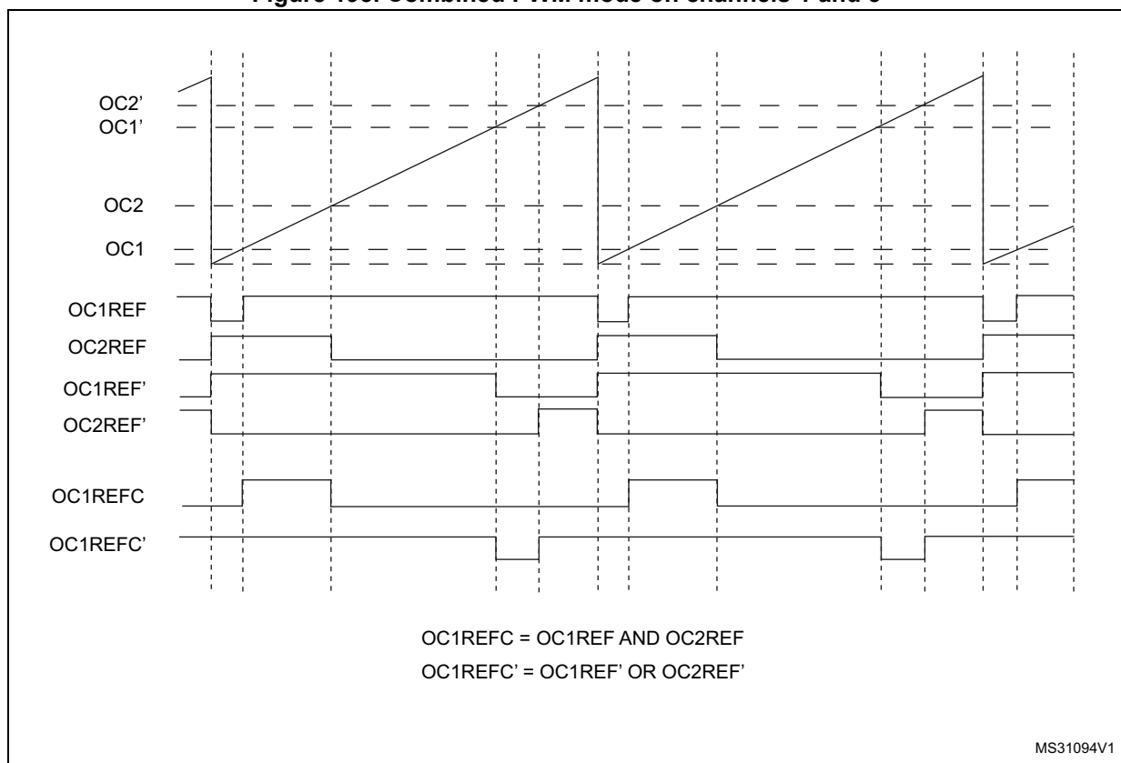
Figure 193. Combined PWM mode on channels 1 and 3
