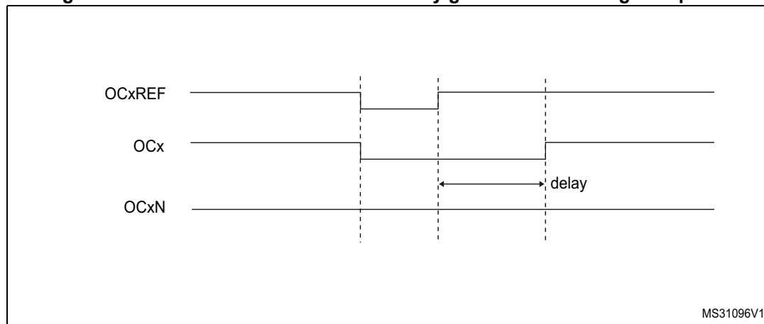
Figure 258. Dead-time waveforms with delay greater than the negative pulse.
