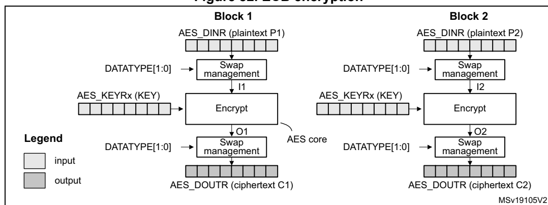
Figure 82. ECB encryption
