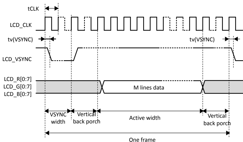
Figure 53. LCD-TFT vertical timing diagram
