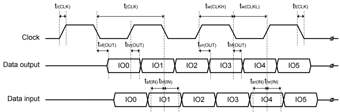
Figure 42. OctoSPI Hyperbus clock
