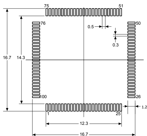
Figure 74. LQFP - 100 pins, 14 x 14 mm low-profile quad flat recommended footprint
