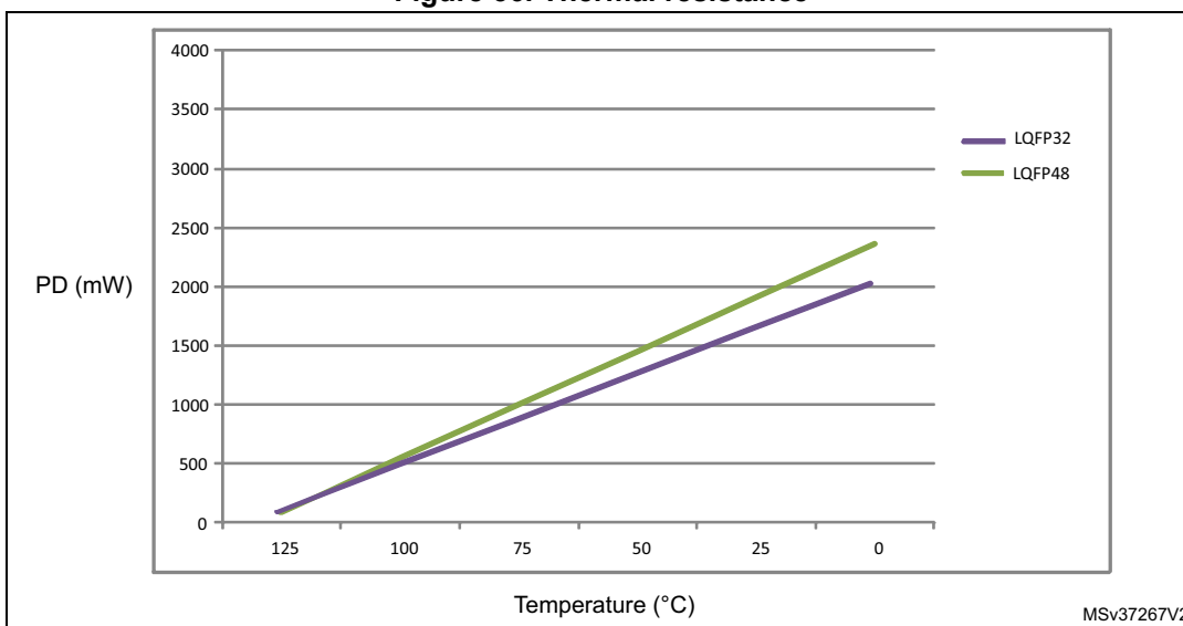
Figure 36. Thermal resistance
