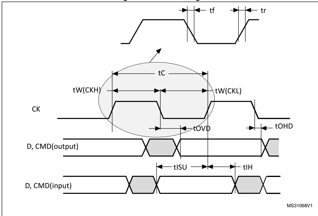
Figure 35. SDIO timings
