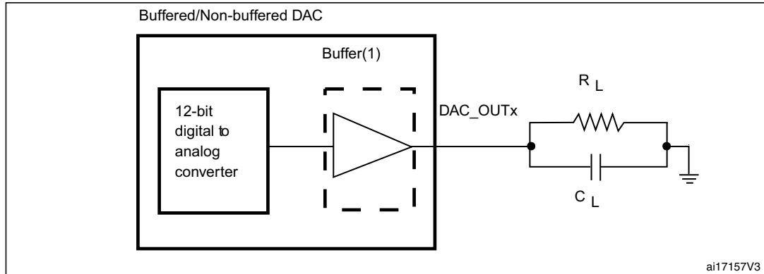
Figure 39. 12-bit buffered /non-buffered DAC
