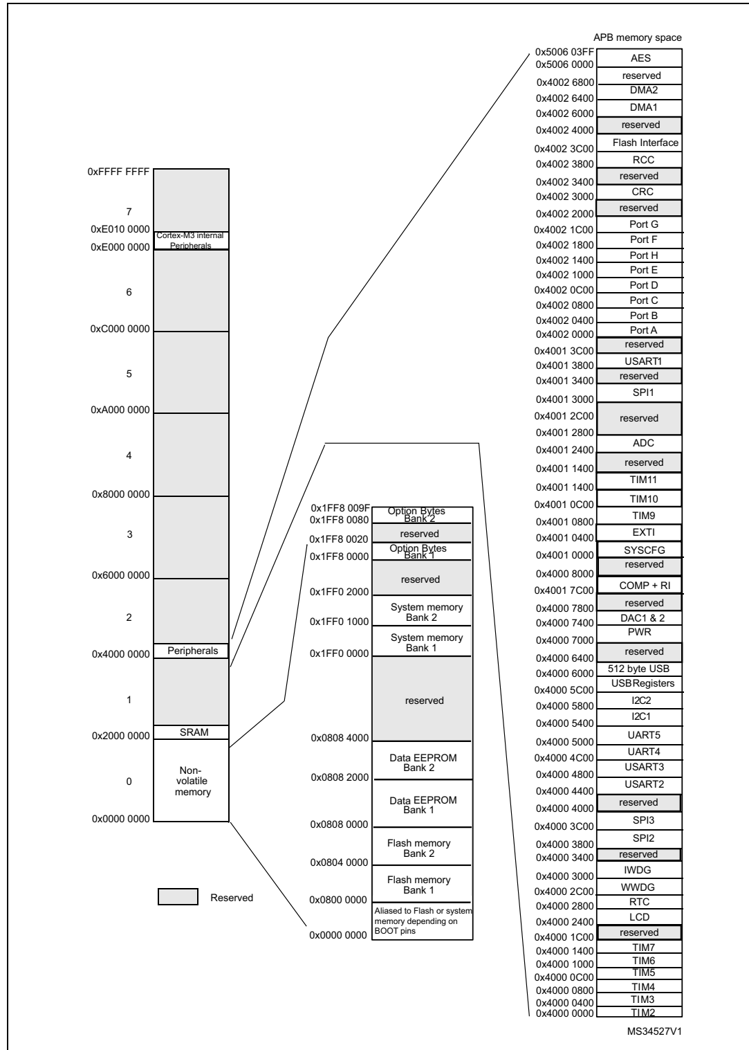
Figure 7. Memory map
