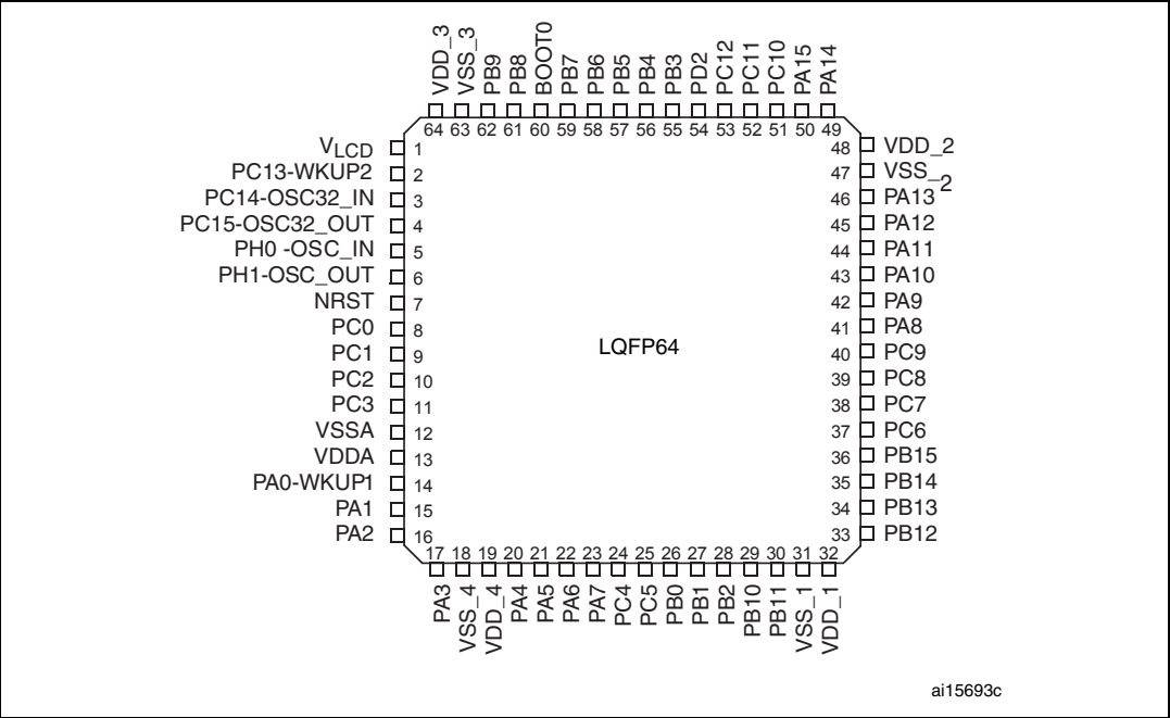
Figure 6. STM32L162RD LQFP64 pinout
