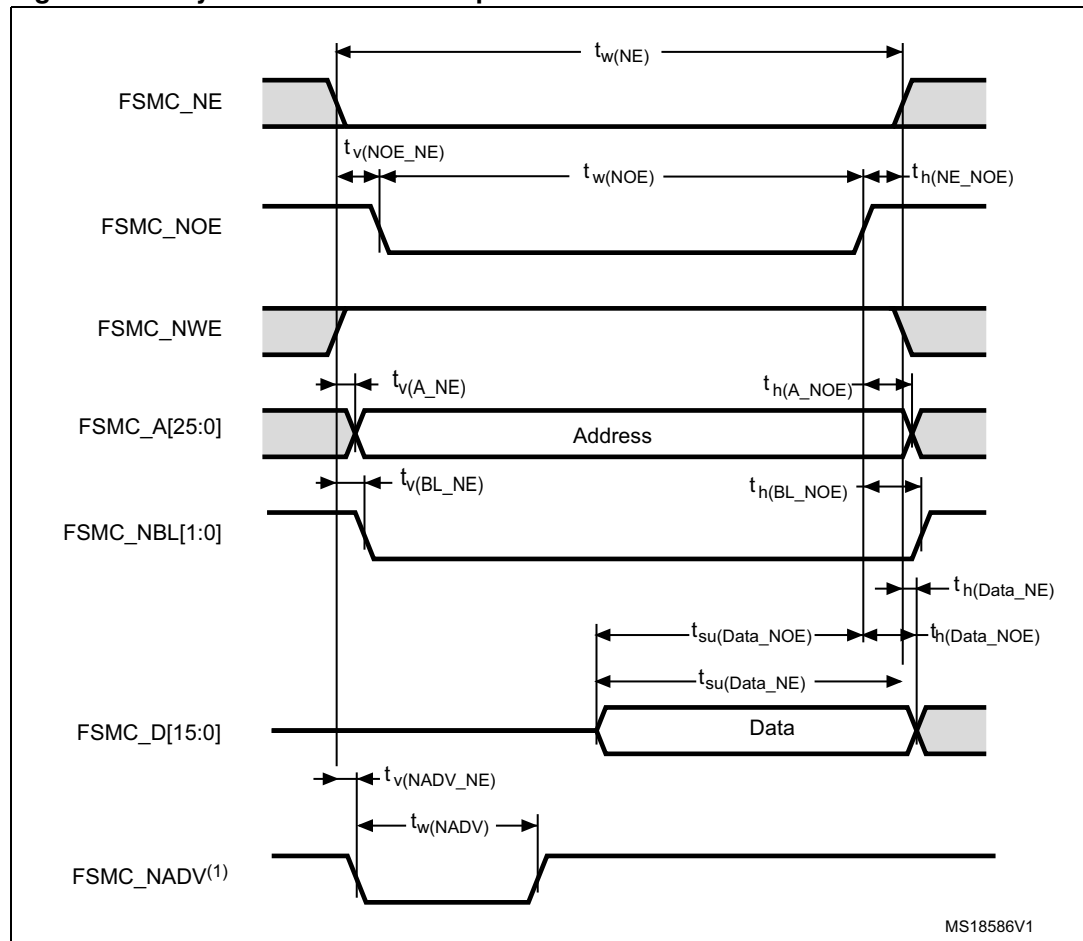
Figure 17. Asynchronous non-multiplexed SRAM/PSRAM/NOR read waveforms
