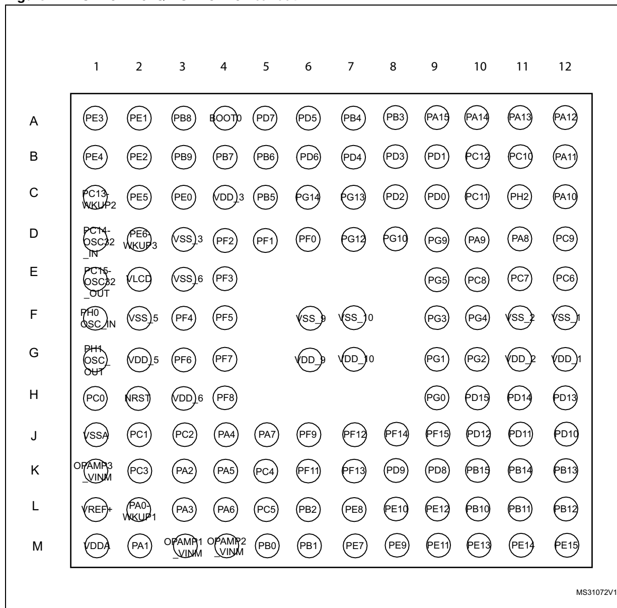
Figure 4. STM32L162QD UFBGA132 ballout
