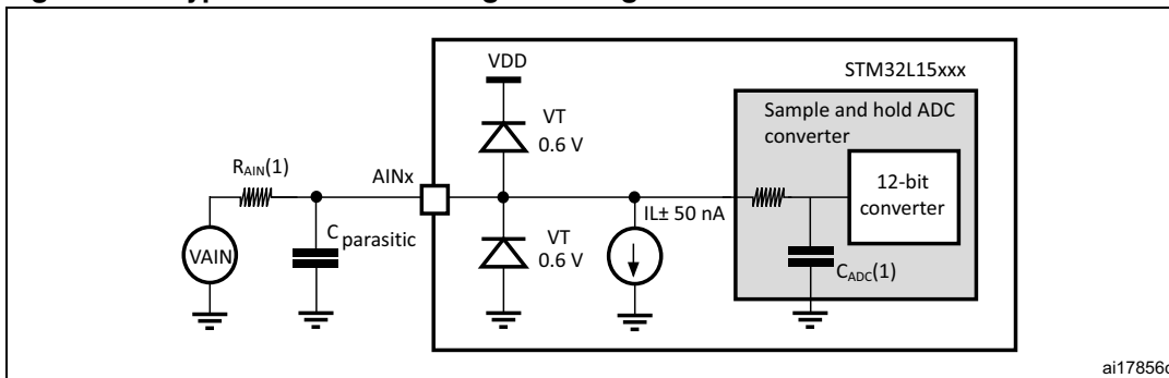
Figure 36. Typical connection diagram using the ADC
