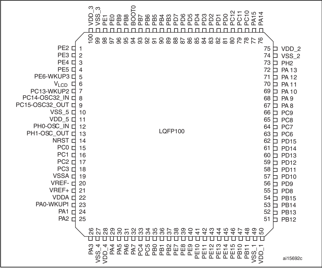
Figure 5. STM32L162VD LQFP100 pinout
