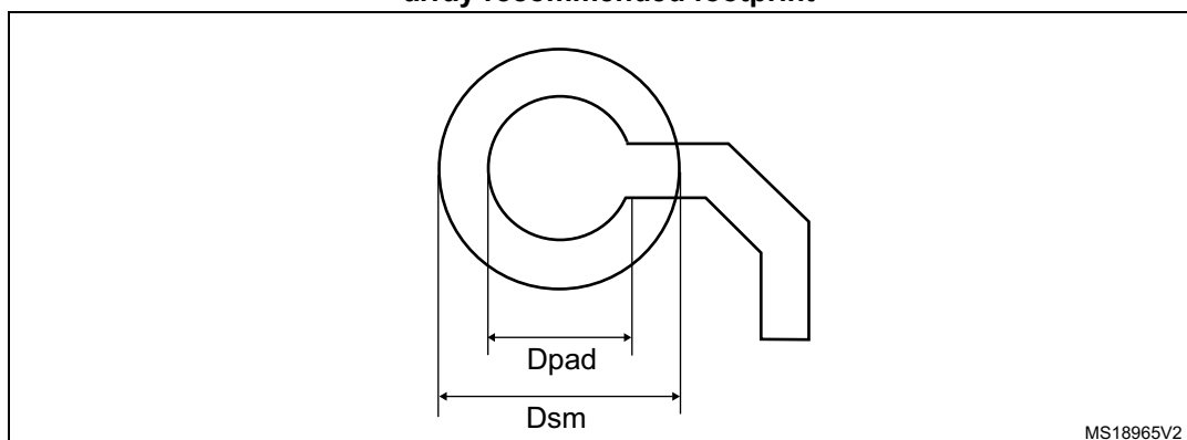
Figure 64. UFBGA169 - 169-ball, 7 x 7 mm, 0.50 mm pitch, ultra fine pitch ball grid array recommended footprint
