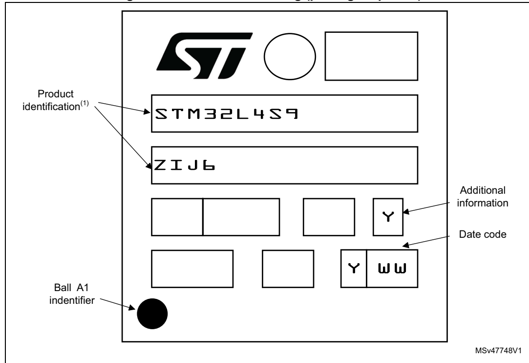
Figure 68. UFBGA144 marking (package top view)
