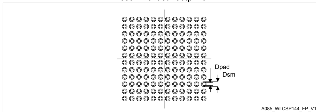
Figure 73. WLCSP - 144 bump, 5.24x 5.24 mm, 0.40 mm pitch, wafer level chip scale, recommended footprint
