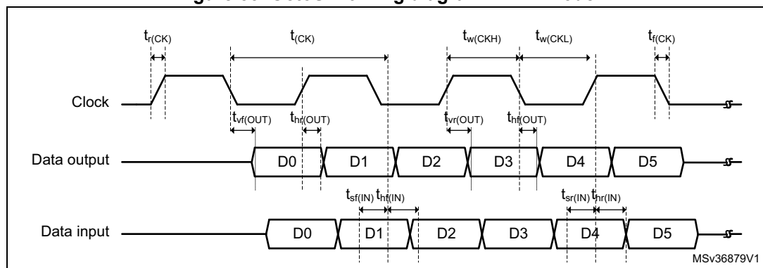
Figure 56. OctoSPI Hyperbus clock
