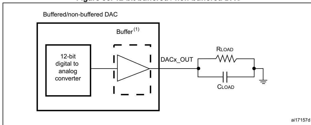
Figure 35. 12-bit buffered / non-buffered DAC
