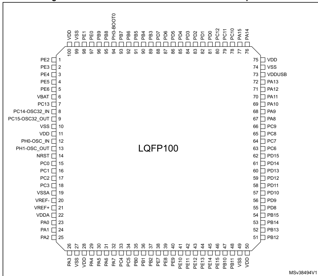
Figure 15. STM32L4S5xx and STM32L4S7xx LQFP100 pinout (1)
