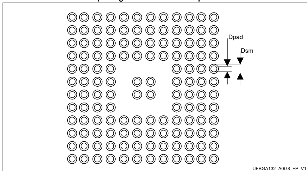
Figure 76. UFBGA132 - 132-ball, 7 x 7 mm ultra thin fine pitch ball grid array package recommended footprint
