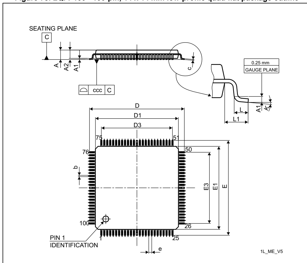
Figure 78. LQFP100 - 100-pin, 14 x 14 mm low-profile quad flat package outline
