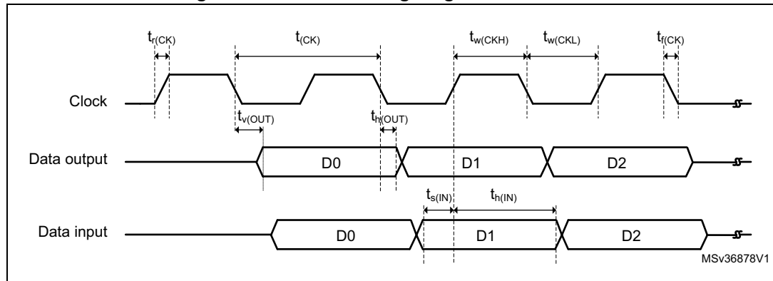
Figure 54. OctoSPI timing diagram - SDR mode
