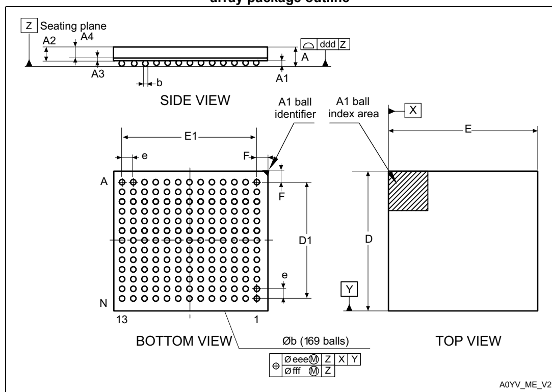
Figure 63. UFBGA169 - 169-ball, 7 x 7 mm, 0.50 mm pitch, ultra fine pitch ball grid array package outline
