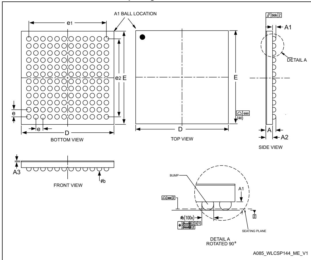
Figure 72. WLCSP - 144 bump, 5.24x 5.24 mm, 0.40 mm pitch, wafer level chip scale, package outline
