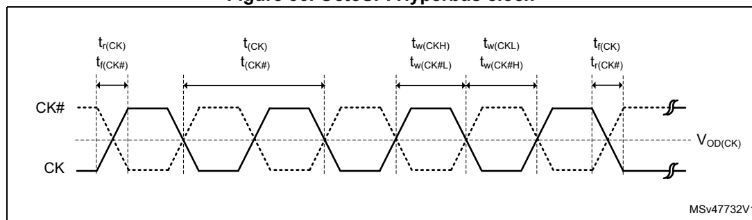
Figure 56. OctoSPI Hyperbus clock
