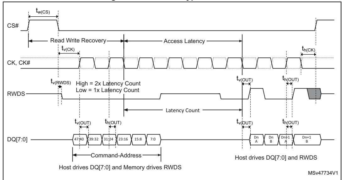
Figure 58. OctoSPI Hyperbus write
