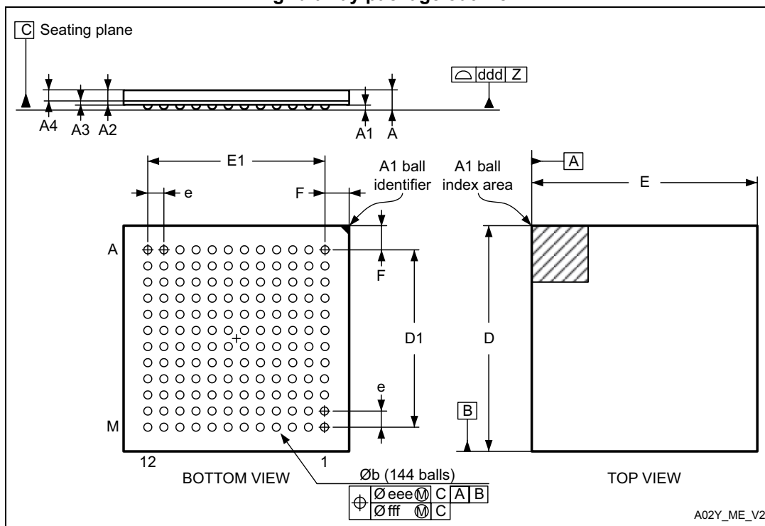
Figure 66. UFBGA144 - 144-pin, 10 x 10 mm, 0.80 mm pitch, ultra fine pitch ball grid array package outline
