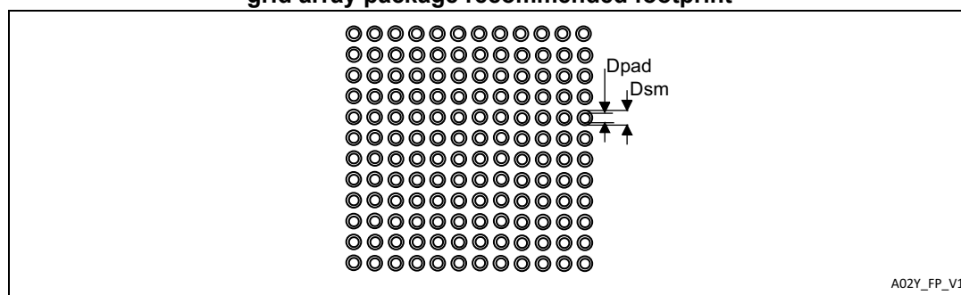
Figure 67. UFBGA144 - 144-pin, 10 x 10 mm, 0.80 mm pitch, ultra fine pitch ball grid array package recommended footprint
