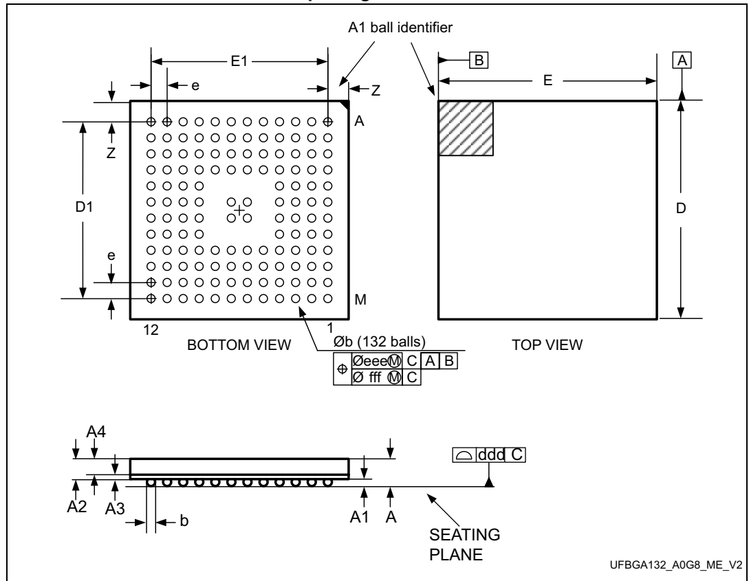
Figure 75. UFBGA132 - 132-ball, 7 x 7 mm ultra thin fine pitch ball grid array package outline
