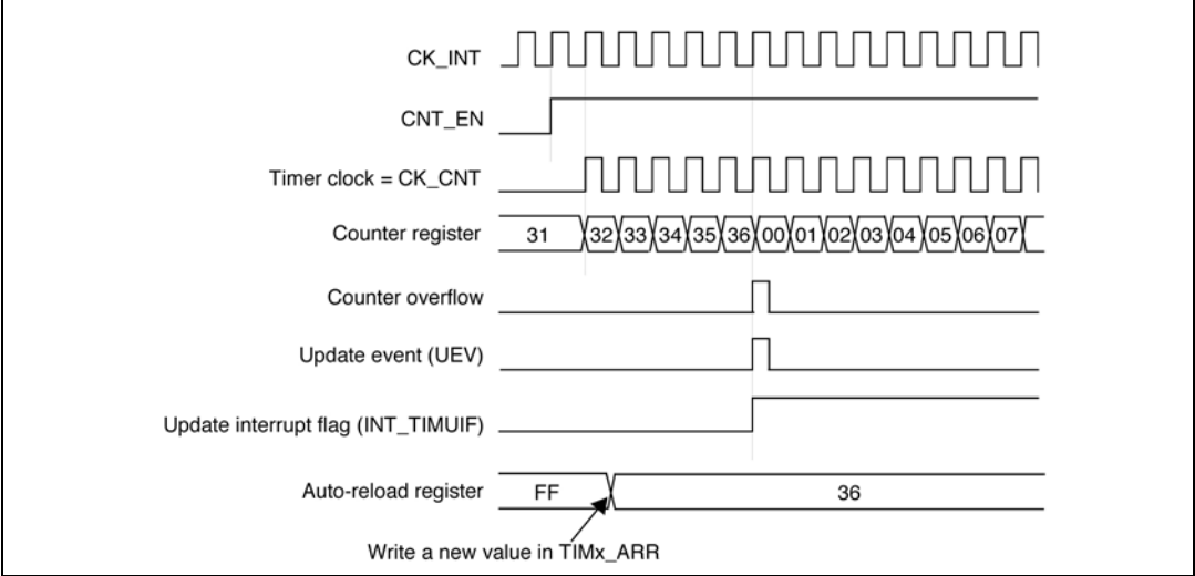
Figure 19. Counter timing diagram, update event when TIM_ARBE = 0 (TIMx_ARR not buffered)
