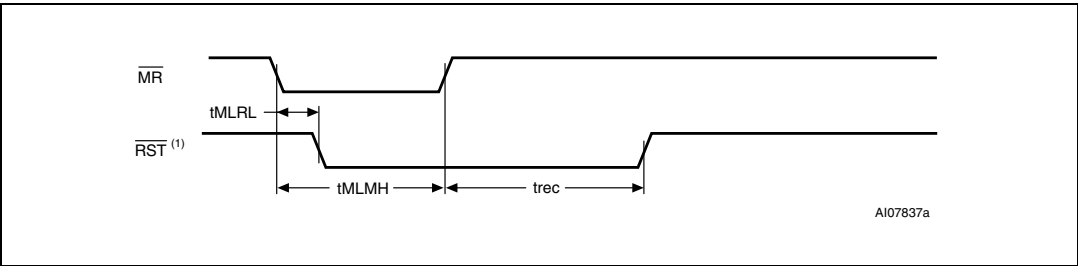
Figure 25. \overline{\text{MR}} timing waveform
