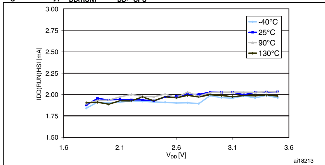
Figure 13. Typ. I_{DD}(\text{RUN}) vs. V_{DD} , f_{CPU} = 16 \text{ MHz}
