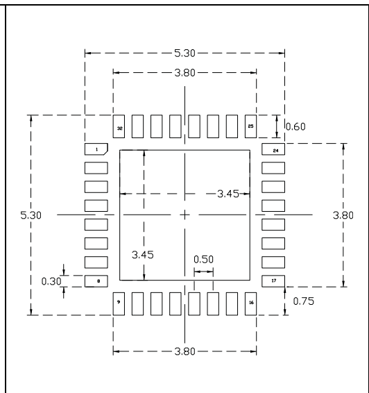
Figure 48. UFQFPN32 recommended footprint (1)(4)
