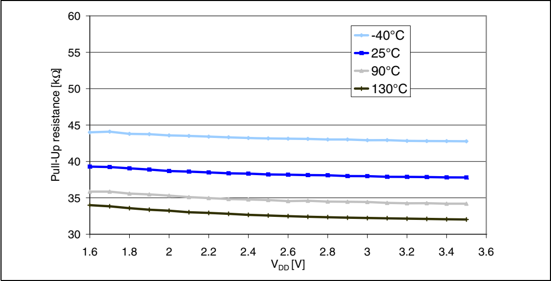
Figure 22. Typical pull-up resistance R_{PU} vs V_{DD} with V_{IN}=V_{SS}
