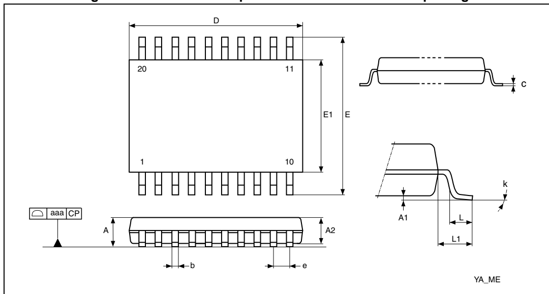
Figure 49. TSSOP20 - 20-pin thin shrink small outline package
