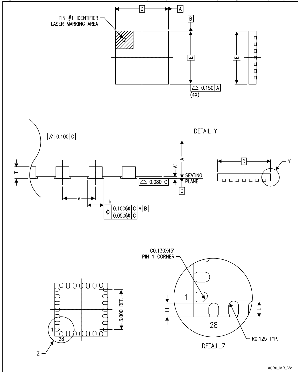
Figure 45. UFQFPN28 – 28-lead ultra thin fine pitch quad flat no-lead package outline (4 x 4)
