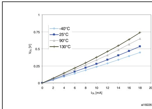
Figure 24. Typ. V_{OL} @ V_{DD} = 3.0 V (high sink ports)
