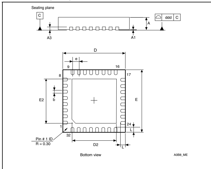
Figure 43. UFQFPN32 - 32-lead ultra thin fine pitch quad flat no-lead package outline (5 x 5) (1)(2)(3)
