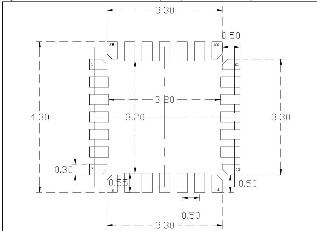
Figure 46. UFQFPN28 recommended footprint (dimensions in mm)
