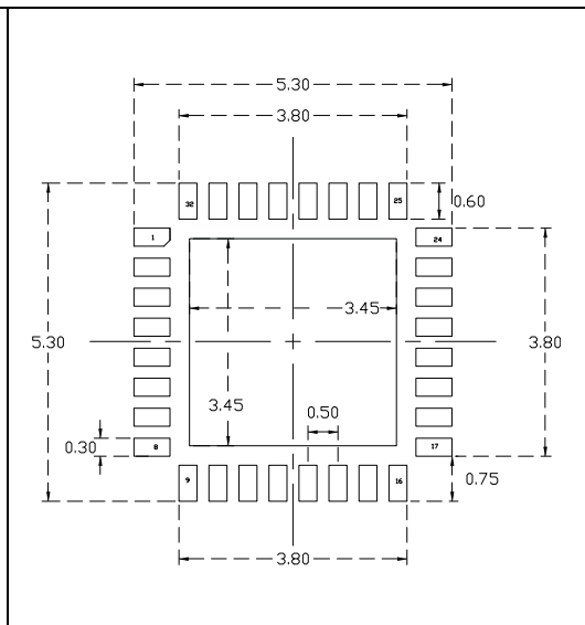
Figure 44. UFQFPN32 recommended footprint (1)(4)
