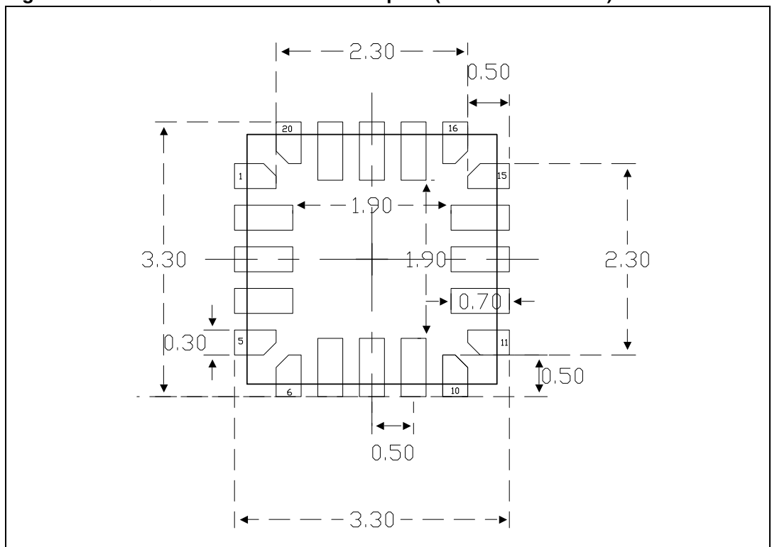
Figure 48. UFQFPN20 recommended footprint (dimensions in mm)
