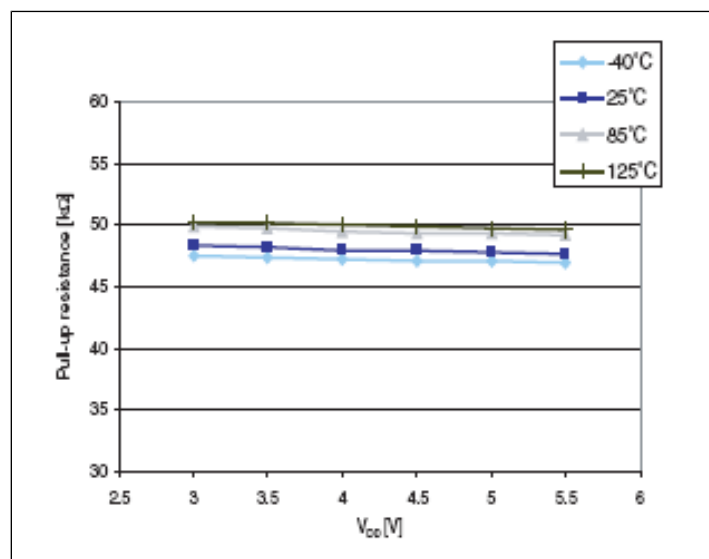
Figure 23: Typical pull-up resistance vs V_{\text{DD}} @ 4 temperatures
