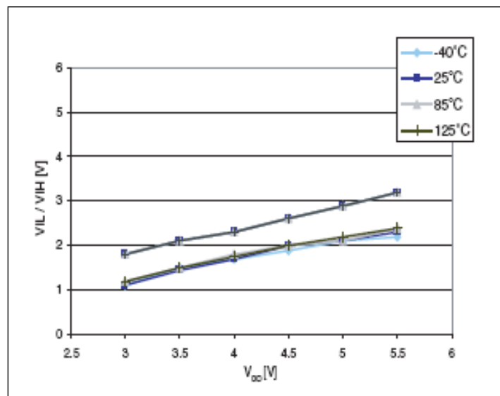
Figure 22: Typical V_{\text{IL}} and V_{\text{IH}} vs V_{\text{DD}} @ 4 temperatures
