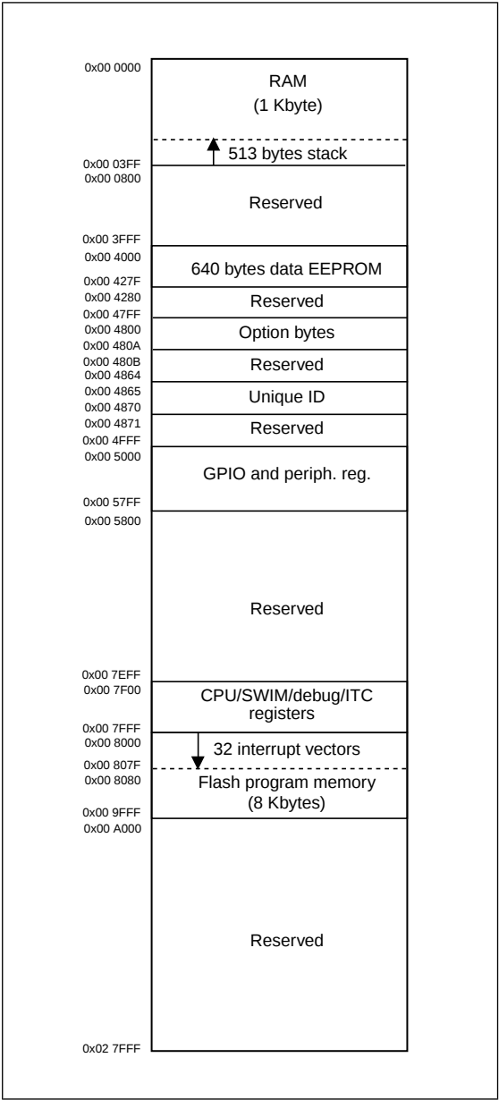
Figure 6: Memory map
