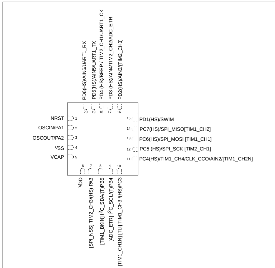
Figure 5: STM8S103Fx UFQFPN20-pin pinout
