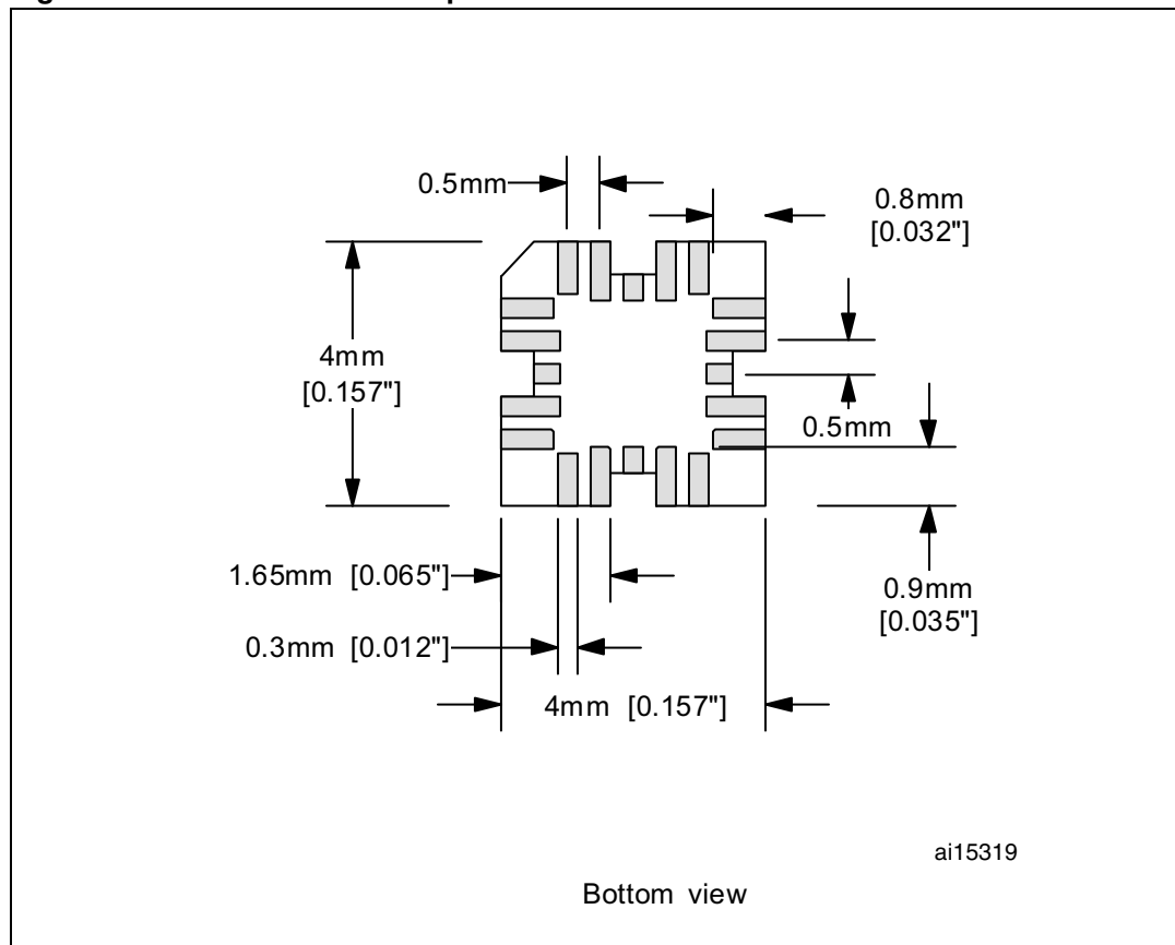
Figure 16. Recommended footprint for on-board emulation
