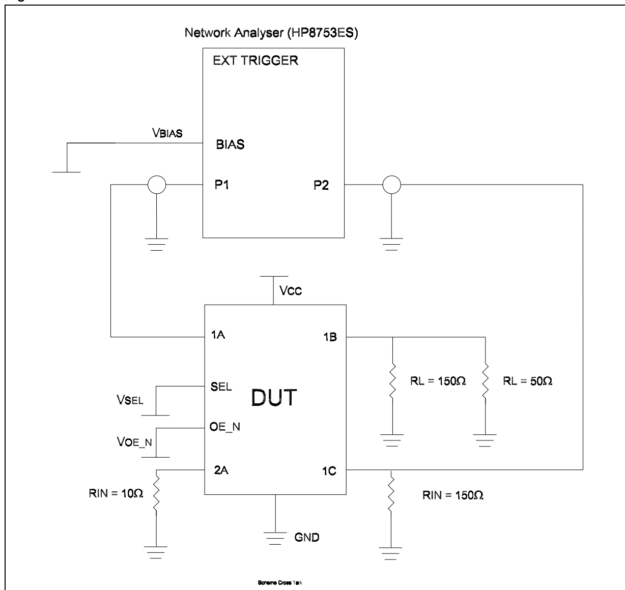
Figure 11. Crosstalk Test Circuit
