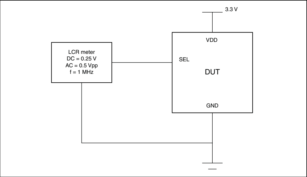
Figure 5. Test circuit for SEL pin input capacitance ( C_{IN} )
