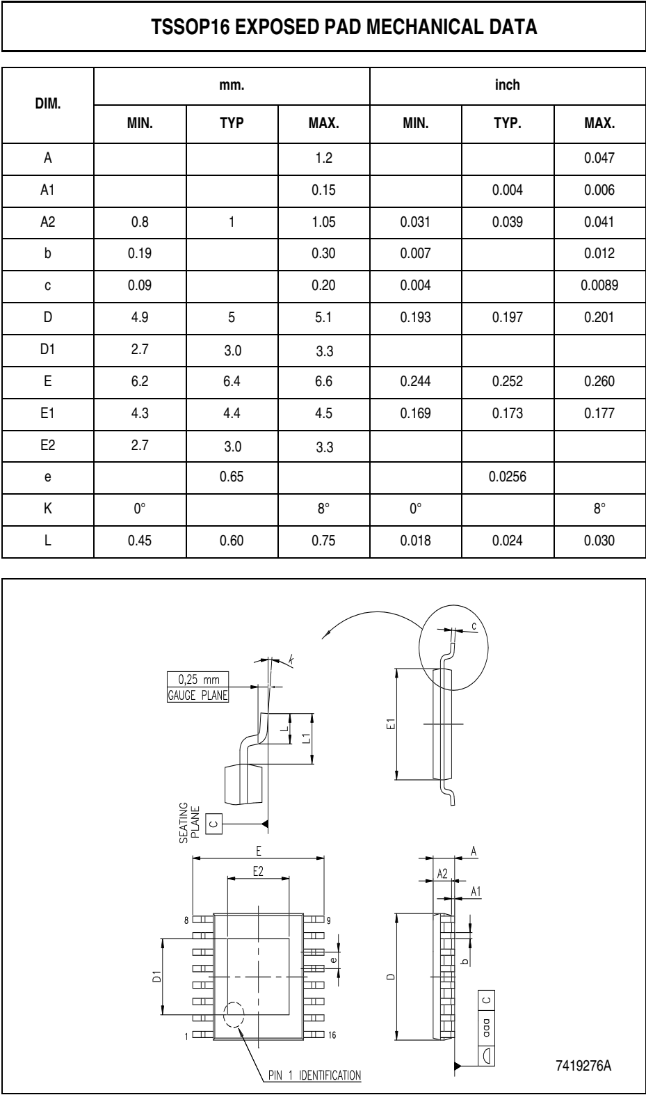
Figure 20. TSSOP16 exposed pad mechanical data
